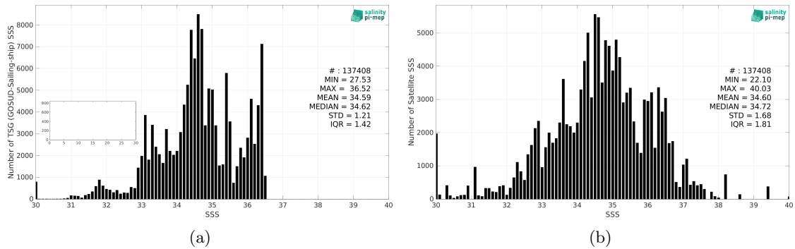
Figure 2: Histograms of SSS from TSG (GOSUD-Sailing-ship) (a) and SMOS SSS L2Q v331 - No FLAG (CMEMS-CATDS-CPDC) (b) considering all match-up pairs per bins of 0.1 over the Pacific Ocean Pi-MEP region and for the full satellite product period.
