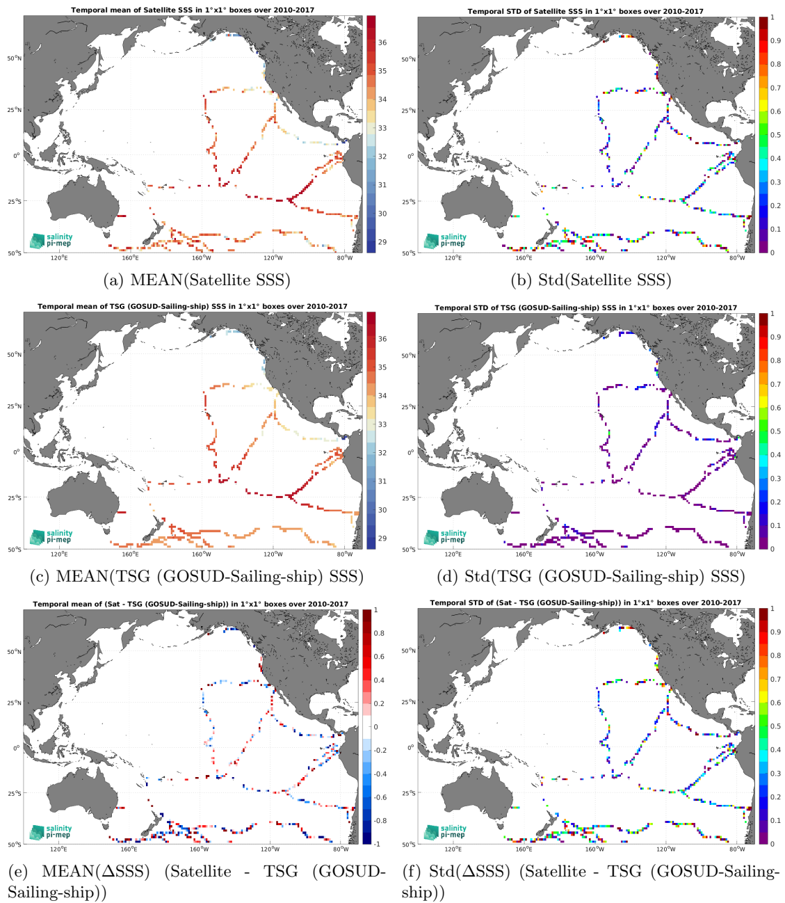
Figure 6: Temporal mean (left) and Std (right) of SSS from SMOS SSS L2Q v331 - No FLAG (CMEMS-CATDS-CPDC) (top), TSG (GOSUD-Sailing-ship) (middle), and of \Delta SSS (Satellite - TSG (GOSUD-Sailing-ship)). Only match-up pairs are used to generate these maps.
