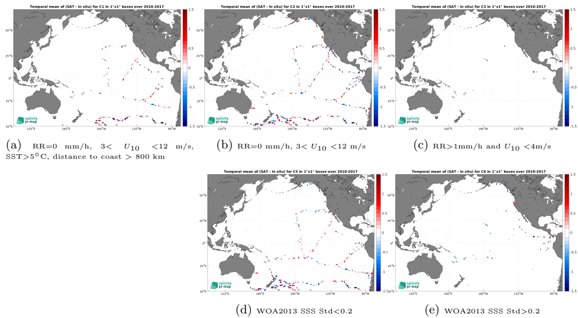
Figure 12: Temporal mean gridded over spatial boxes of size 1^\circ \times 1^\circ of \Delta SSS (SMOS SSS L2Q v331 - No FLAG (CMEMS-CATDS-CPDC) - TSG (GOSUD-Sailing-ship)) for 5 different sub-datasets corresponding to: RR=0 mm/h, 3 < U_{10} < 12 m/s, SST > 5^\circ\text{C} , distance to coast > 800 km (a), RR=0 mm/h, 3 < U_{10} < 12 m/s (b), RR > 1 mm/h and U_{10} < 4 m/s (c), WOA2013 SSS Std < 0.2 (d), WOA2013 SSS Std > 0.2 (e).
