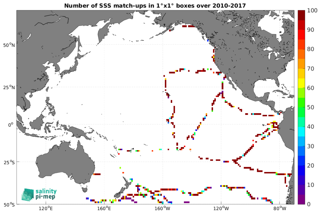
Figure 4: Number of SSS match-ups between TSG (GOSUD-Sailing-ship) SSS and the SMOS SSS L2Q v331 - No FLAG (CMEMS-CATDS-CPDC) SSS product for the Pacific Ocean Pi-MEP region over 1^\circ \times 1^\circ boxes and for the full satellite product period.
