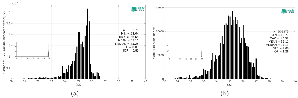
Figure 3: Histograms of SSS from TSG (GOSUD-Research-vessel) (a) and SMOS SSS L2Q v331 - No FLAG (CMEMS-CATDS-CPDC) (b) considering all match-up pairs per bins of 0.1 over the Pacific Ocean Pi-MEP region and for the full satellite product period.
