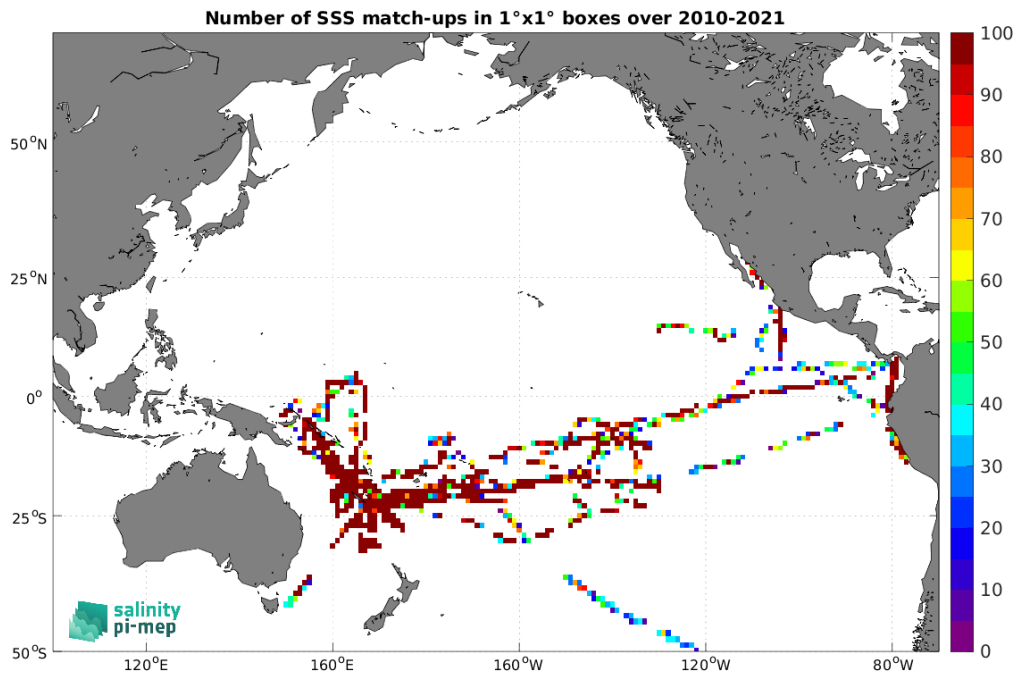
Figure 5: Number of SSS match-ups between TSG (GOSUD-Research-vessel) SSS and the SMOS SSS L2Q v331 - No FLAG (CMEMS-CATDS-CPDC) SSS product for the Pacific Ocean Pi-MEP region over 1^\circ \times 1^\circ boxes and for the full satellite product period.
