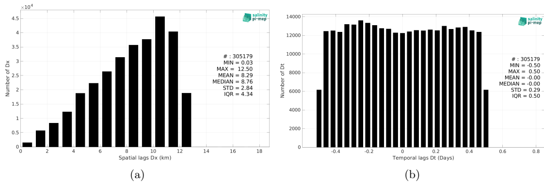
Figure 5: Histograms of the spatial (a) and temporal (b) lags between the location/time of the TSG (GOSUD-Research-vessel) measurement and the date of the corresponding SMOS SSS L2Q v331 - No FLAG (CMEMS-CATDS-CPDC) SSS pixel.
