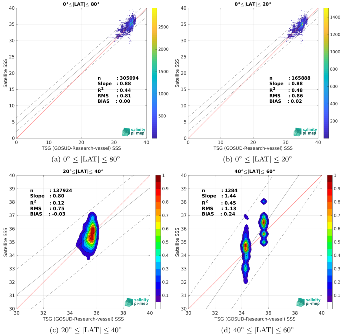
Figure 9: Contour maps of the concentration of SMOS SSS L2Q v331 - No FLAG (CMEMS-CATDS-CPDC) SSS (y-axis) versus TSG (GOSUD-Research-vessel) SSS (x-axis) at match-up pairs for different latitude bands. For each plot, the red line shows x=y . The black thin and dashed lines indicate a linear fit through the data cloud and the \pm 95\% confidence levels, respectively. The number match-up pairs n , the slope and R^2 coefficient of the linear fit, the root mean square (RMS) and the mean bias between satellite and in situ data are indicated for each latitude band in each plots.
