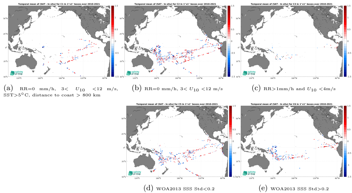
Figure 12: Temporal mean gridded over spatial boxes of size 1^\circ \times 1^\circ of \Delta SSS (SMOS SSS L2Q v331 - No FLAG (CMEMS-CATDS-CPDC) - TSG (GOSUD-Research-vessel)) for 5 different subdatasets corresponding to:RR=0 mm/h, 3 < U_{10} < 12 m/s, SST > 5^\circ\text{C} , distance to coast > 800 km (a), RR=0 mm/h, 3 < U_{10} < 12 m/s (b), RR > 1 mm/h and U_{10} < 4 m/s (c), WOA2013 SSS Std < 0.2 (d), WOA2013 SSS Std > 0.2 (e).
