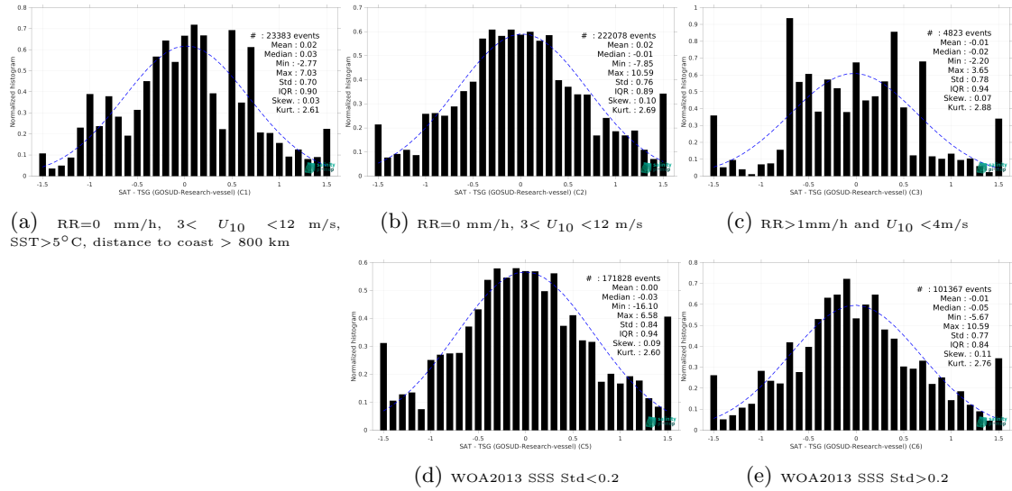
Figure 13: Normalized histogram of \Delta SSS (SMOS SSS L2Q v331 - No FLAG (CMEMS-CATDS-CPDC) - TSG (GOSUD-Research-vessel)) for 5 different subdatasets corresponding to: RR=0 mm/h, 3 < U_{10} < 12 m/s, SST>5°C, distance to coast > 800 km (a), RR=0 mm/h, 3 < U_{10} < 12 m/s (b), RR>1mm/h and U_{10} < 4 m/s (c), WOA2013 SSS Std<0.2 (d), WOA2013 SSS Std>0.2 (e).
