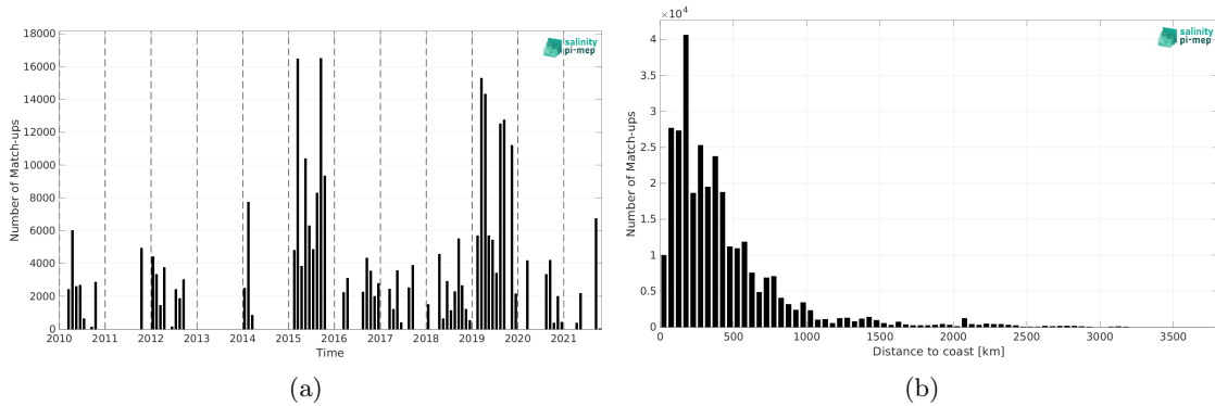
Figure 1: Number of match-ups between TSG (GOSUD-Research-vessel) and SMOS SSS L2Q v331 - No FLAG (CMEMS-CATDS-CPDC) SSS as a function of time (a) and as function of the distance to coast (b) over the Pacific Ocean Pi-MEP region and for the full satellite product period.
