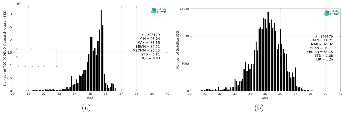
Figure 2: Histograms of SSS from TSG (GOSUD-Research-vessel) (a) and SMOS SSS L2Q v331 - No FLAG (CMEMS-CATDS-CPDC) (b) considering all match-up pairs per bins of 0.1 over the Pacific Ocean Pi-MEP region and for the full satellite product period.
