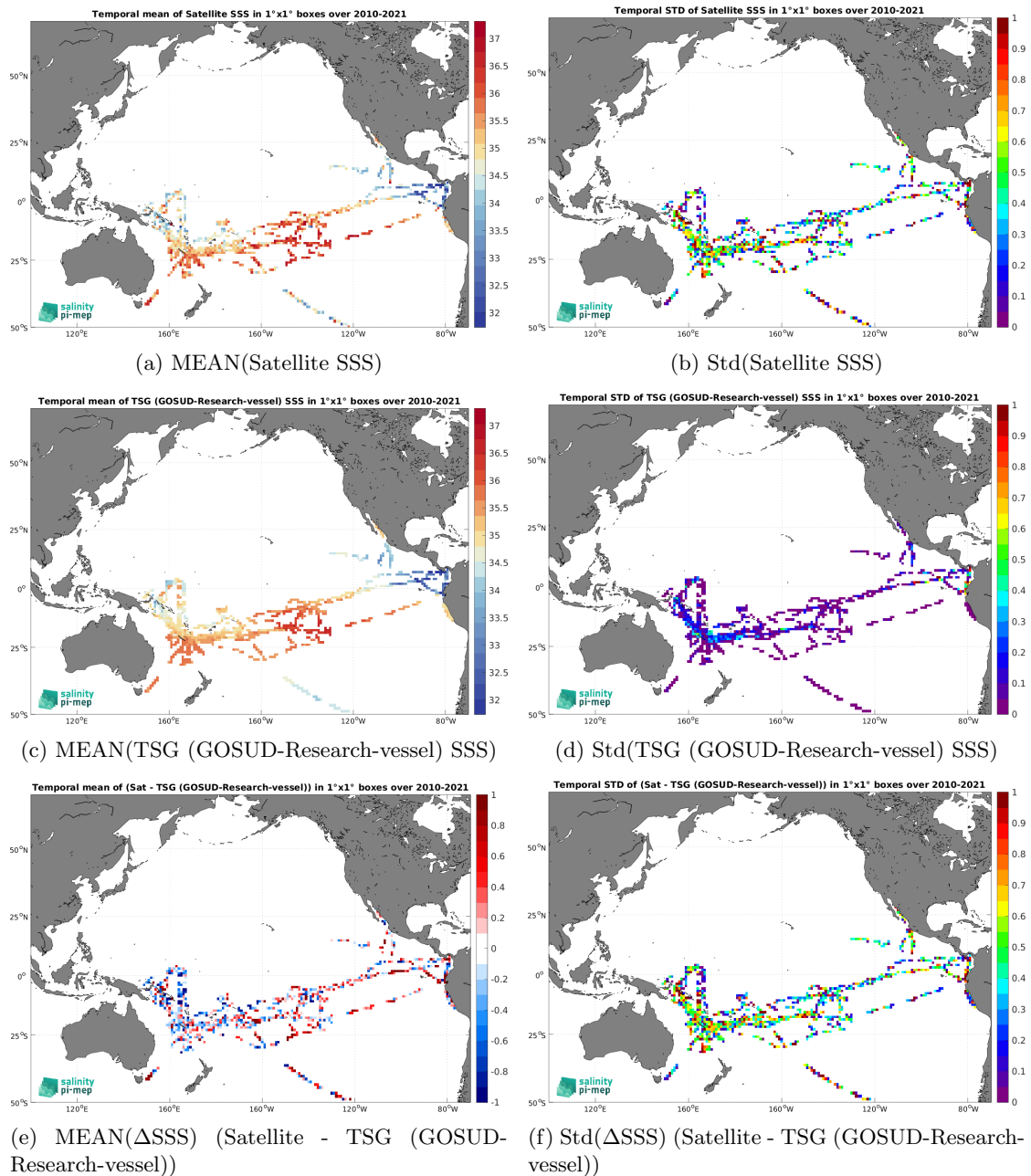
Figure 6: Temporal mean (left) and Std (right) of SSS from SMOS SSS L2Q v331 - No FLAG (CMEMS-CATDS-CPDC) (top), TSG (GOSUD-Research-vessel) (middle), and of \Delta SSS (Satellite - TSG (GOSUD-Research-vessel)). Only match-up pairs are used to generate these maps.
