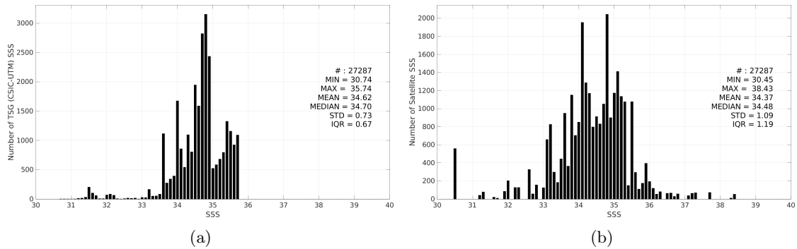
Figure 3: Histograms of SSS from TSG (CSIC-UTM) (a) and SMOS SSS L2Q v331 - No FLAG (CMEMS-CATDS-CPDC) (b) considering all match-up pairs per bins of 0.1 over the Pacific Ocean Pi-MEP region and for the full satellite product period.
