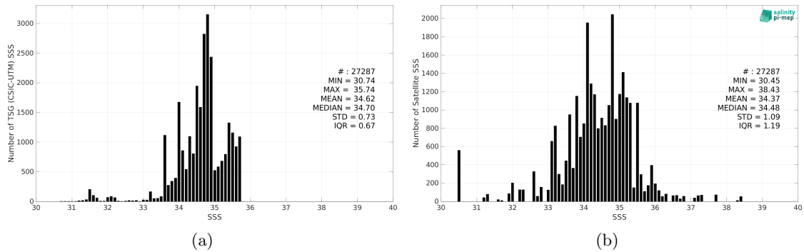
Figure 2: Histograms of SSS from TSG (CSIC-UTM) (a) and SMOS SSS L2Q v331 - No FLAG (CMEMS-CATDS-CPDC) (b) considering all match-up pairs per bins of 0.1 over the Pacific Ocean Pi-MEP region and for the full satellite product period.
