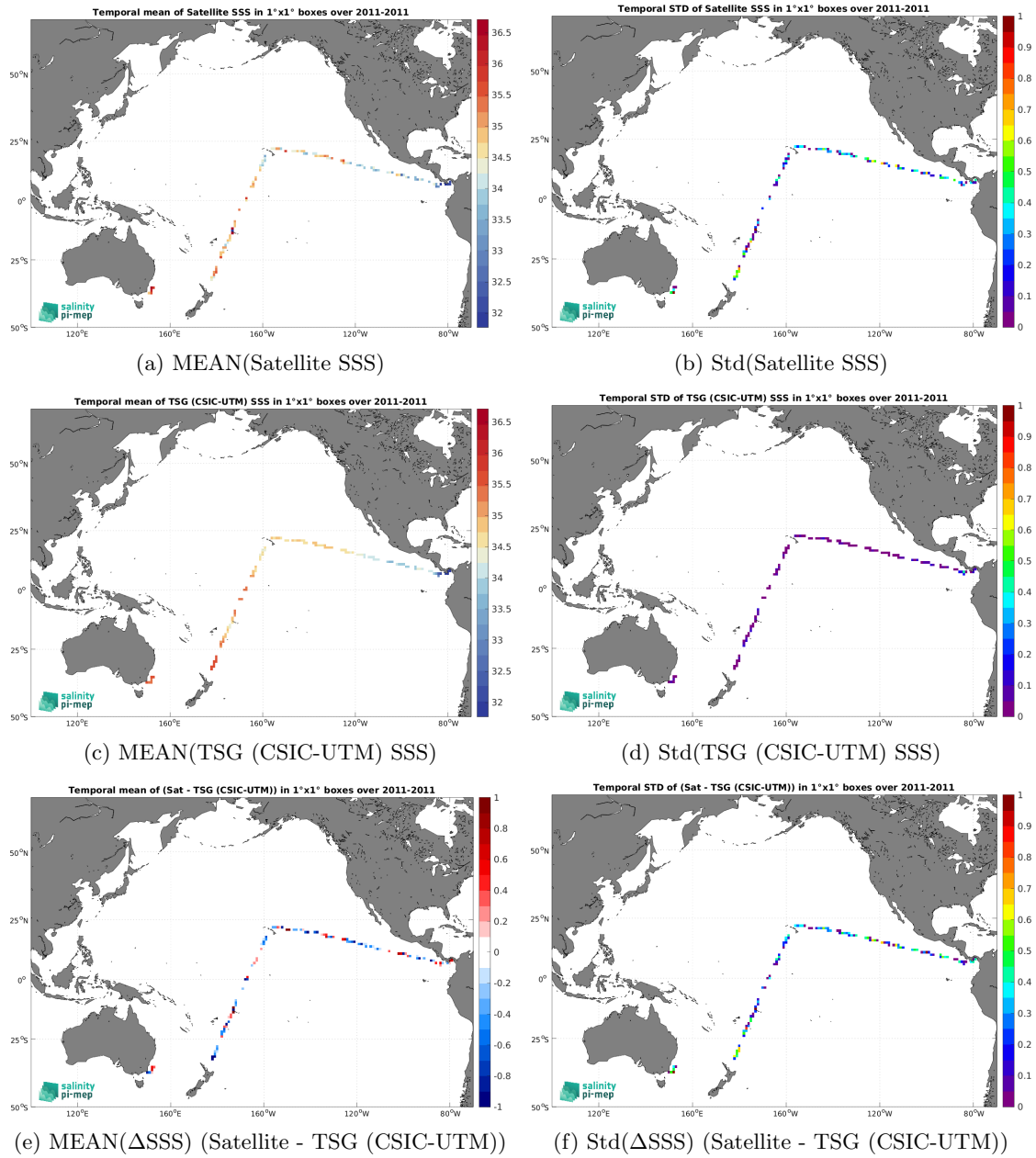
Figure 6: Temporal mean (left) and Std (right) of SSS from SMOS SSS L2Q v331 - No FLAG (CMEMS-CATDS-CPDC) (top), TSG (CSIC-UTM) (middle), and of \Delta SSS (Satellite - TSG (CSIC-UTM)). Only match-up pairs are used to generate these maps.
