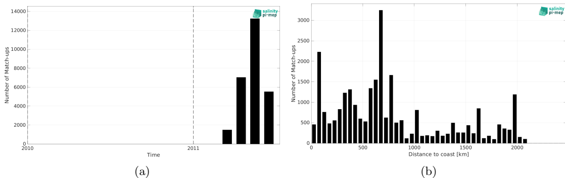
Figure 1: Number of match-ups between TSG (CSIC-UTM) and SMOS SSS L2Q v331 - No FLAG (CMEMS-CATDS-CPDC) SSS as a function of time (a) and as function of the distance to coast (b) over the Pacific Ocean Pi-MEP region and for the full satellite product period.
