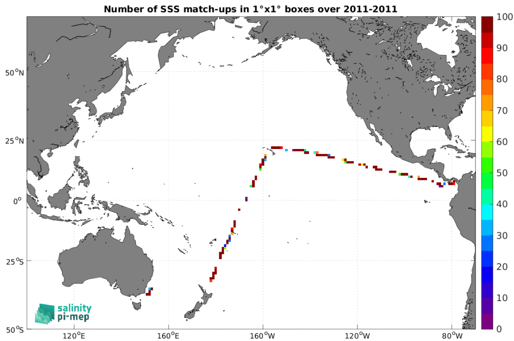
Figure 4: Number of SSS match-ups between TSG (CSIC-UTM) SSS and the SMOS SSS L2Q v331 - No FLAG (CMEMS-CATDS-CPDC) SSS product for the Pacific Ocean Pi-MEP region over 1^\circ \times 1^\circ boxes and for the full satellite product period.
