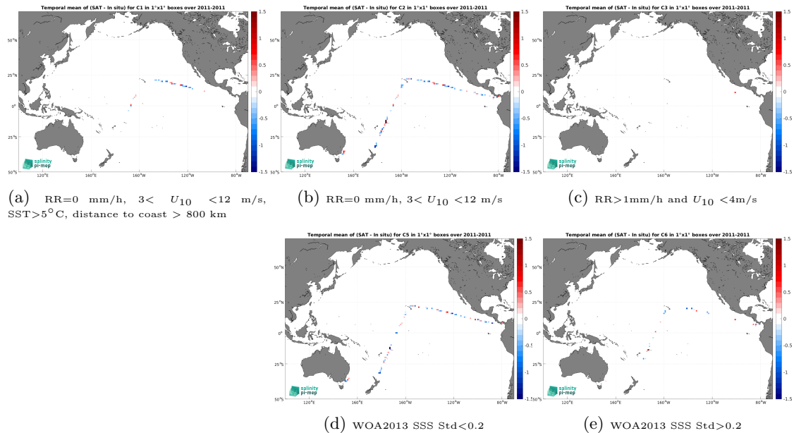
Figure 12: Temporal mean gridded over spatial boxes of size 1^{\circ}\times 1^{\circ} of \Delta\text{SSS} (SMOS SSS L2Q v331 - No FLAG (CMEMS-CATDS-CPDC) - TSG (CSIC-UTM)) for 5 different subdatasets corresponding to:RR=0 mm/h, 3 < U_{10} < 12 m/s, SST >5^{\circ}\text{C} , distance to coast > 800 km (a), RR=0 mm/h, 3 < U_{10} < 12 m/s (b), RR >1 mm/h and U_{10} < 4 m/s (c), WOA2013 SSS Std <0.2 (d), WOA2013 SSS Std >0.2 (e).
