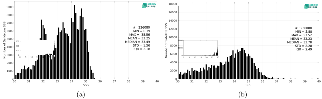
Figure 3: Histograms of SSS from Saildrone (a) and SMOS SSS L2Q v331 - No FLAG (CMEMS-CATDS-CPDC) (b) considering all match-up pairs per bins of 0.1 over the Pacific Ocean Pi-MEP region and for the full satellite product period.
