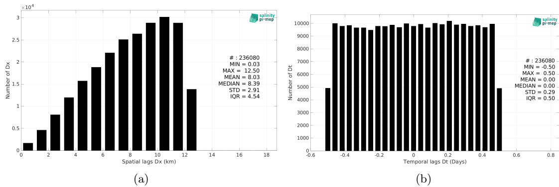
Figure 6: Histograms of the spatial (a) and temporal (b) lags between the location/time of the Saildrone measurement and the date of the corresponding SMOS SSS L2Q v331 - No FLAG (CMEMS-CATDS-CPDC) SSS pixel.
