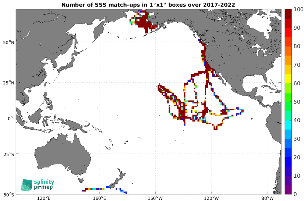
Figure 5: Number of SSS match-ups between Saildrone SSS and the SMOS SSS L2Q v331 - No FLAG (CMEMS-CATDS-CPDC) SSS product for the Pacific Ocean Pi-MEP region over 1^\circ \times 1^\circ boxes and for the full satellite product period.
