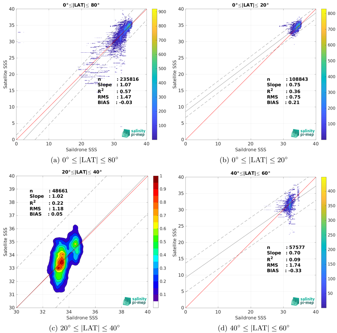
Figure 10: Contour maps of the concentration of SMOS SSS L2Q v331 - No FLAG (CMEMS-CATDS-CPDC) SSS (y-axis) versus Saildrone SSS (x-axis) at match-up pairs for different latitude bands. For each plot, the red line shows x=y . The black thin and dashed lines indicate a linear fit through the data cloud and the \pm 95\% confidence levels, respectively. The number match-up pairs n , the slope and R^2 coefficient of the linear fit, the root mean square (RMS) and the mean bias between satellite and in situ data are indicated for each latitude band in each plots.
