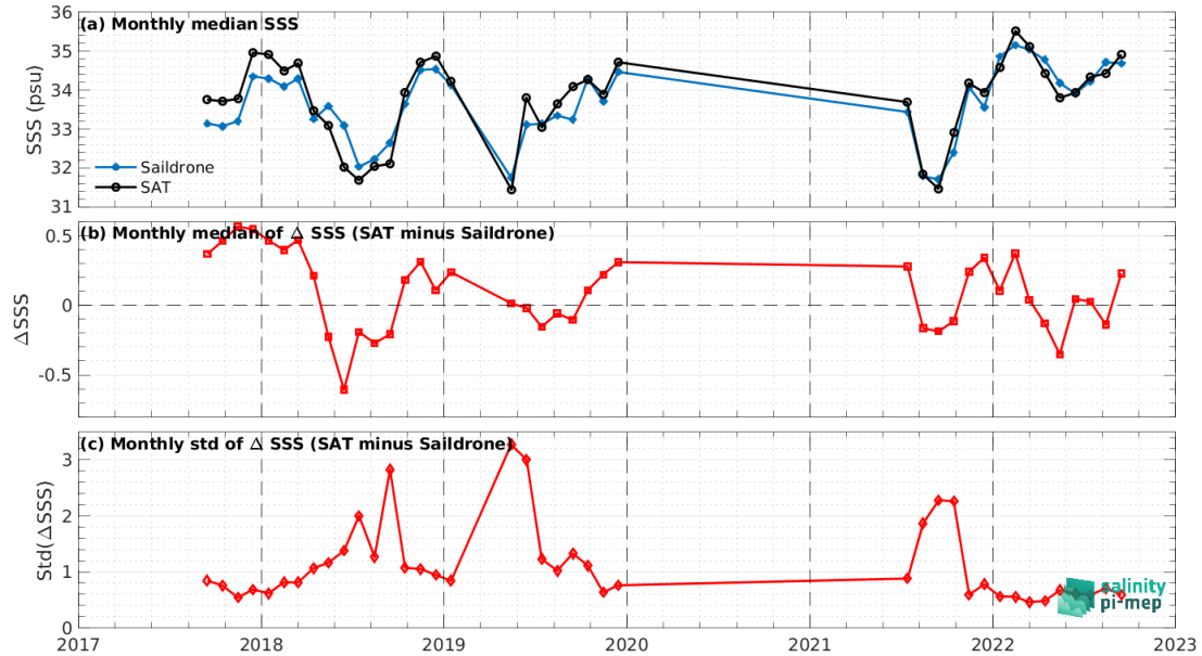
Figure 8: Time series of the monthly median SSS (top), median of \Delta SSS (Satellite - Sairdrone) and Std of \Delta SSS (Satellite - Sairdrone) over the Pacific Ocean Pi-MEP region considering all match-ups collected by the Pi-MEP.
