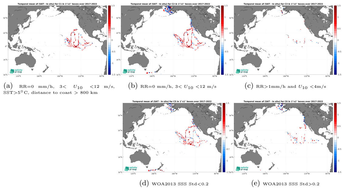
Figure 14: Temporal mean gridded over spatial boxes of size 1^\circ \times 1^\circ of \Delta SSS (SMOS SSS L2Q v331 - No FLAG (CMEMS-CATDS-CPDC) - Sairdrone) for 5 different subdatasets corresponding to:RR=0 mm/h, 3 < U_{10} < 12 m/s, SST >5^\circ C, distance to coast > 800 km (a), RR=0 mm/h, 3 < U_{10} < 12 m/s (b), RR >1 mm/h and U_{10} < 4 m/s (c), WOA2013 SSS Std <0.2 (d), WOA2013 SSS Std >0.2 (e).
