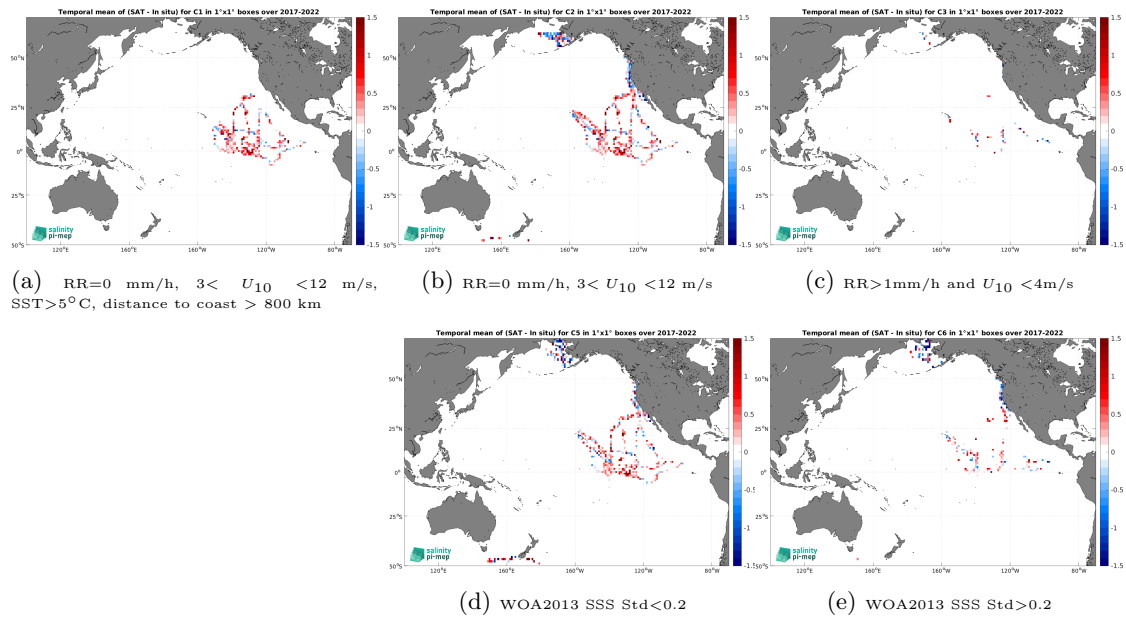
Figure 12: Temporal mean gridded over spatial boxes of size 1^\circ \times 1^\circ of \Delta SSS (SMOS SSS L2Q v331 - No FLAG (CMEMS-CATDS-CPDC) - Saildrone) for 5 different subdatasets corresponding to:RR=0 mm/h, 3 < U_{10} < 12 m/s, SST >5^\circ C, distance to coast > 800 km (a), RR=0 mm/h, 3 < U_{10} < 12 m/s (b), RR >1 mm/h and U_{10} < 4 m/s (c), WOA2013 SSS Std <0.2 (d), WOA2013 SSS Std >0.2 (e).
