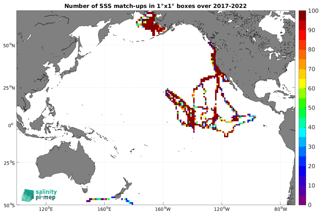
Figure 4: Number of SSS match-ups between Saildrone SSS and the SMOS SSS L2Q v331 - No FLAG (CMEMS-CATDS-CPDC) SSS product for the Pacific Ocean Pi-MEP region over 1°x1° boxes and for the full satellite product period.
