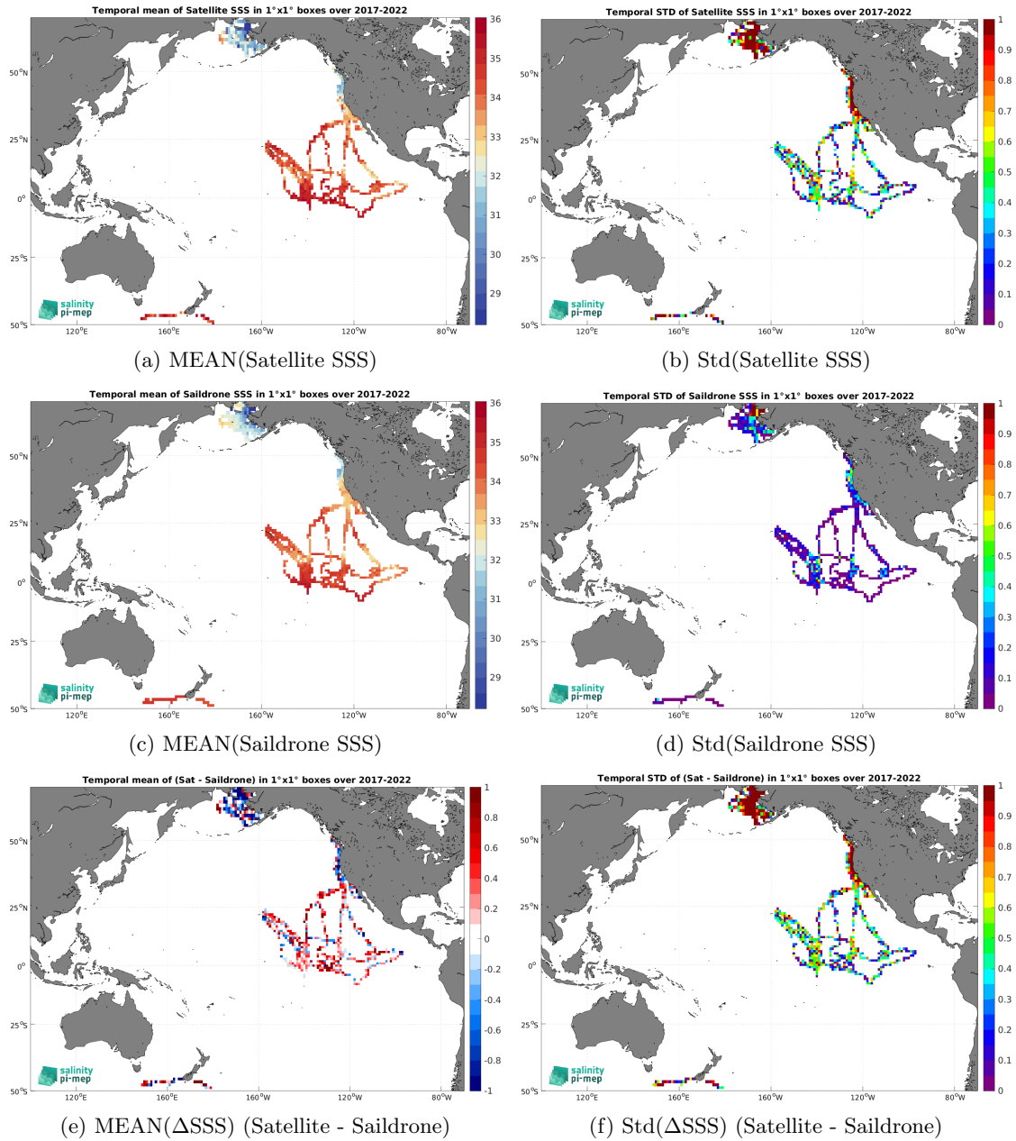
Figure 6: Temporal mean (left) and Std (right) of SSS from SMOS SSS L2Q v331 - No FLAG (CMEMS-CATDS-CPDC) (top), Saildrone (middle), and of \Delta SSS (Satellite - Saildrone). Only match-up pairs are used to generate these maps.
