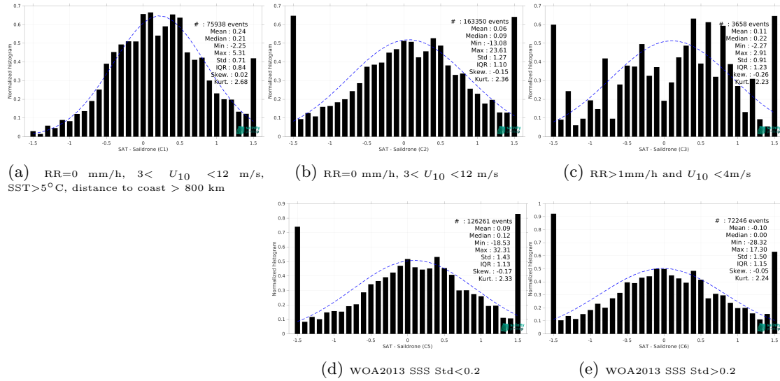
Figure 13: Normalized histogram of \Delta SSS (SMOS SSS L2Q v331 - No FLAG (CMEMS-CATDS-CPDC) - Salldrone) for 5 different subdatasets corresponding to: RR=0 mm/h, 3 < U_{10} < 12 m/s, SST > 5°C, distance to coast > 800 km (a), RR=0 mm/h, 3 < U_{10} < 12 m/s (b), RR > 1mm/h and U_{10} < 4 m/s (c), WOA2013 SSS Std < 0.2 (d), WOA2013 SSS Std > 0.2 (e).
