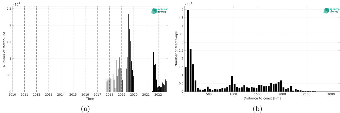
Figure 1: Number of match-ups between Saildrone and SMOS SSS L2Q v331 - No FLAG (CMEMS-CATDS-CPDC) SSS as a function of time (a) and as function of the distance to coast (b) over the Pacific Ocean Pi-MEP region and for the full satellite product period.
