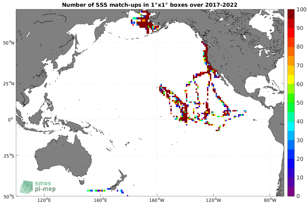
Figure 4: Number of SSS match-ups between Saildrone SSS and the SMOS SSS L2Q v331 - No FLAG (CMEMS-CATDS-CPDC) SSS product for the Pacific Ocean Pi-MEP region over 1^\circ \times 1^\circ boxes and for the full satellite product period.
