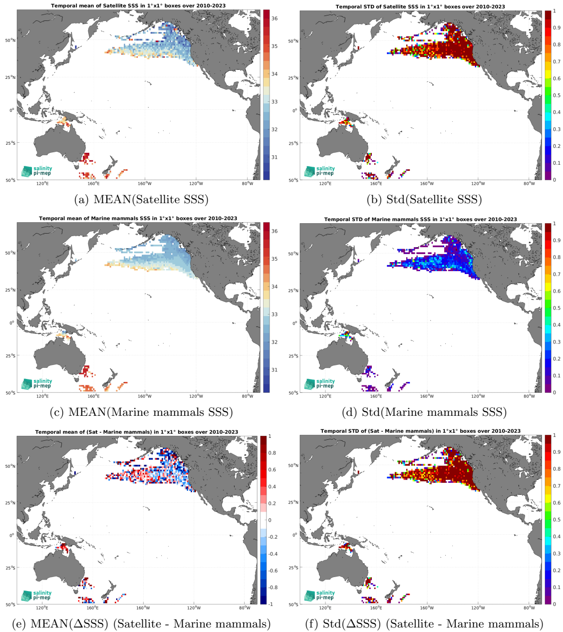
Figure 7: Temporal mean (left) and Std (right) of SSS from SMOS SSS L2Q v331 - No FLAG (CMEMS-CATDS-CPDC) (top), Marine mammals (middle), and of \Delta SSS (Satellite - Marine mammals). Only match-up pairs are used to generate these maps.
