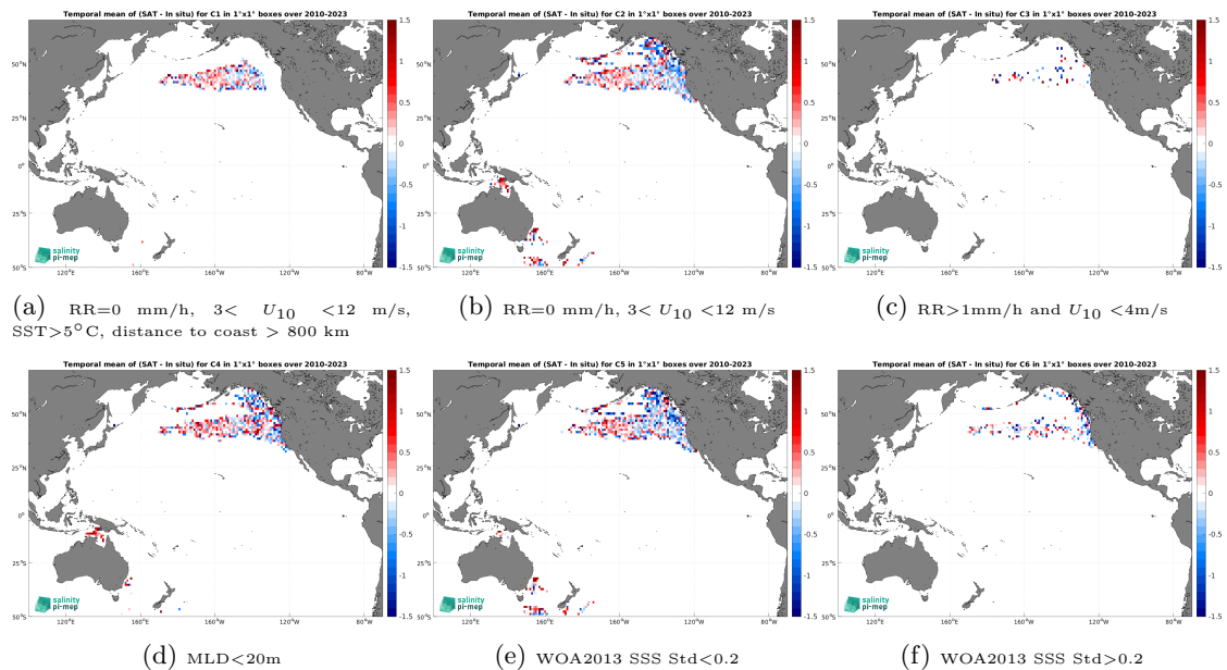
Figure 14: Temporal mean gridded over spatial boxes of size 1^\circ \times 1^\circ of \Delta SSS (SMOS SSS L2Q v331 - No FLAG (CMEMS-CATDS-CPDC) - Marine mammals) for 6 different subdatasets corresponding to:RR=0 mm/h, 3 < U_{10} < 12 m/s, SST >5^\circ C, distance to coast > 800 km (a), RR=0 mm/h, 3 < U_{10} < 12 m/s (b), RR >1 mm/h and U_{10} < 4 m/s (c),MLD <20 m (d),WOA2013 SSS Std <0.2 (e),WOA2013 SSS Std >0.2 (f).
