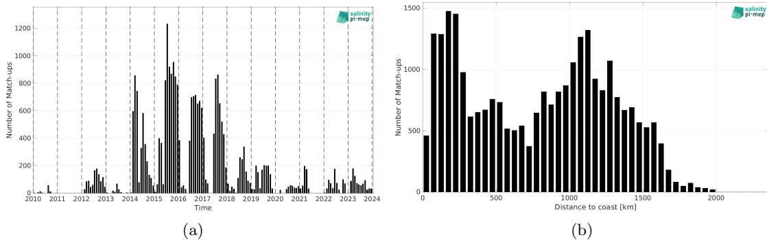
Figure 2: Number of match-ups between Marine mammals and SMOS SSS L2Q v331 - No FLAG (CMEMS-CATDS-CPDC) SSS as a function of time (a) and as function of the distance to coast (b) over the Pacific Ocean Pi-MEP region and for the full satellite product period.
