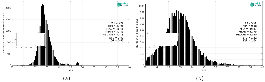
Figure 3: Histograms of SSS from Marine mammals (a) and SMOS SSS L2Q v331 - No FLAG (CMEMS-CATDS-CPDC) (b) considering all match-up pairs per bins of 0.1 over the Pacific Ocean Pi-MEP region and for the full satellite product period.
