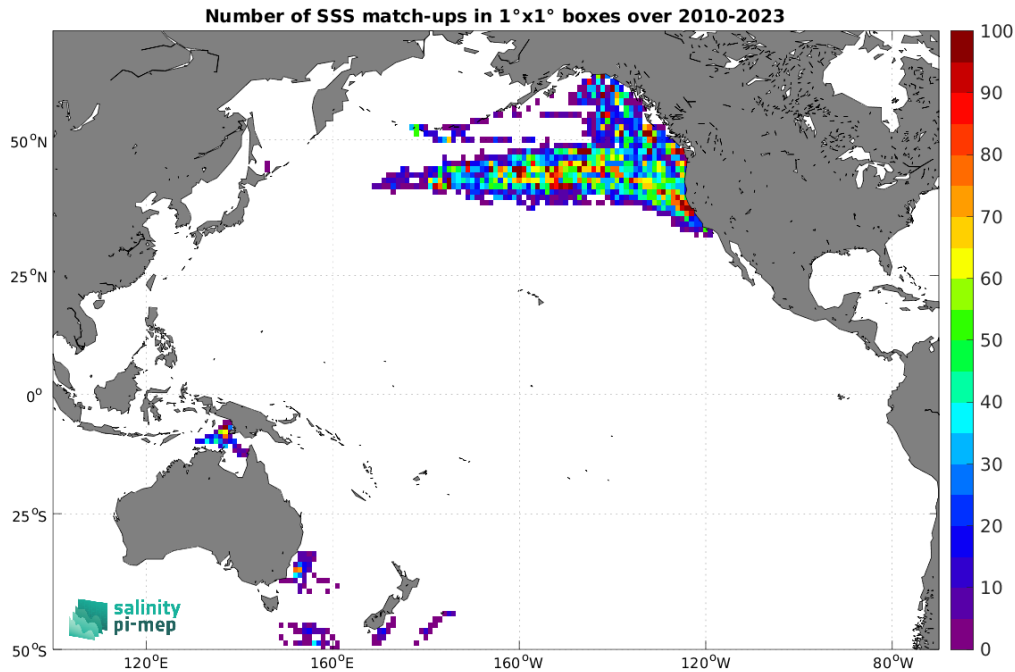
Figure 5: Number of SSS match-ups between Marine mammals SSS and the SMOS SSS L2Q v331 - No FLAG (CMEMS-CATDS-CPDC) SSS product for the Pacific Ocean Pi-MEP region over 1^\circ \times 1^\circ boxes and for the full satellite product period.
