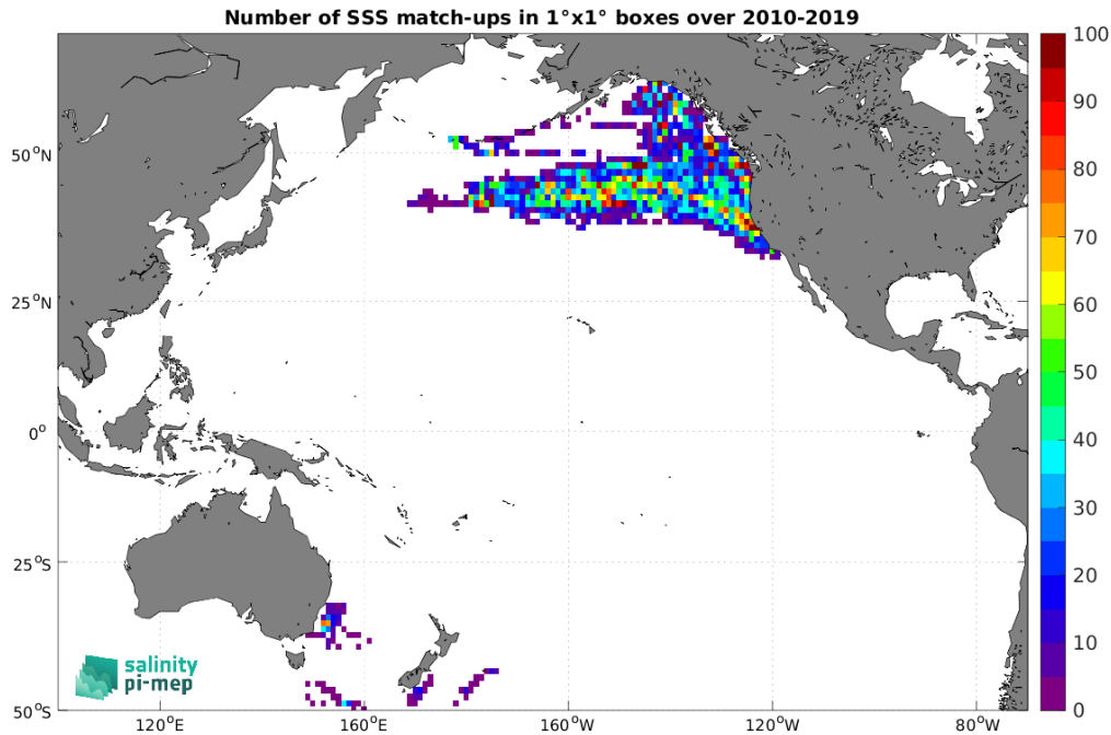
Figure 4: Number of SSS match-ups between Marine mammals SSS and the SMOS SSS L2Q v331 - No FLAG (CMEMS-CATDS-CPDC) SSS product for the Pacific Ocean Pi-MEP region over 1^\circ \times 1^\circ boxes and for the full satellite product period.
