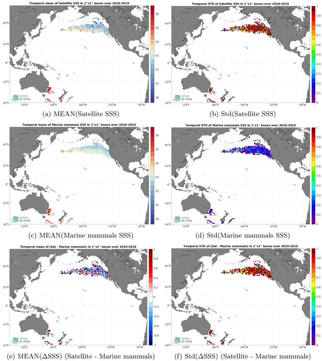
Figure 6: Temporal mean (left) and Std (right) of SSS from SMOS SSS L2Q v331 - No FLAG (CMEMS-CATDS-CPDC) (top), Marine mammals (middle), and of \Delta SSS (Satellite - Marine mammals). Only match-up pairs are used to generate these maps.
