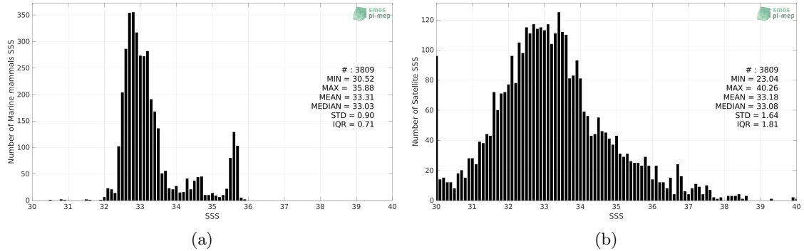
Figure 2: Histograms of SSS from Marine mammals (a) and SMOS SSS L2Q v331 - No FLAG (CMEMS-CATDS-CPDC) (b) considering all match-up pairs per bins of 0.1 over the Pacific Ocean Pi-MEP region and for the full satellite product period.
