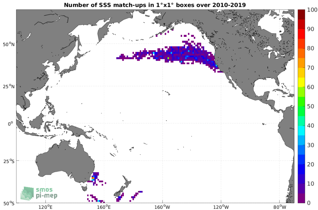
Figure 4: Number of SSS match-ups between Marine mammals SSS and the SMOS SSS L2Q v331 - No FLAG (CMEMS-CATDS-CPDC) SSS product for the Pacific Ocean Pi-MEP region over 1°×1° boxes and for the full satellite product period.
