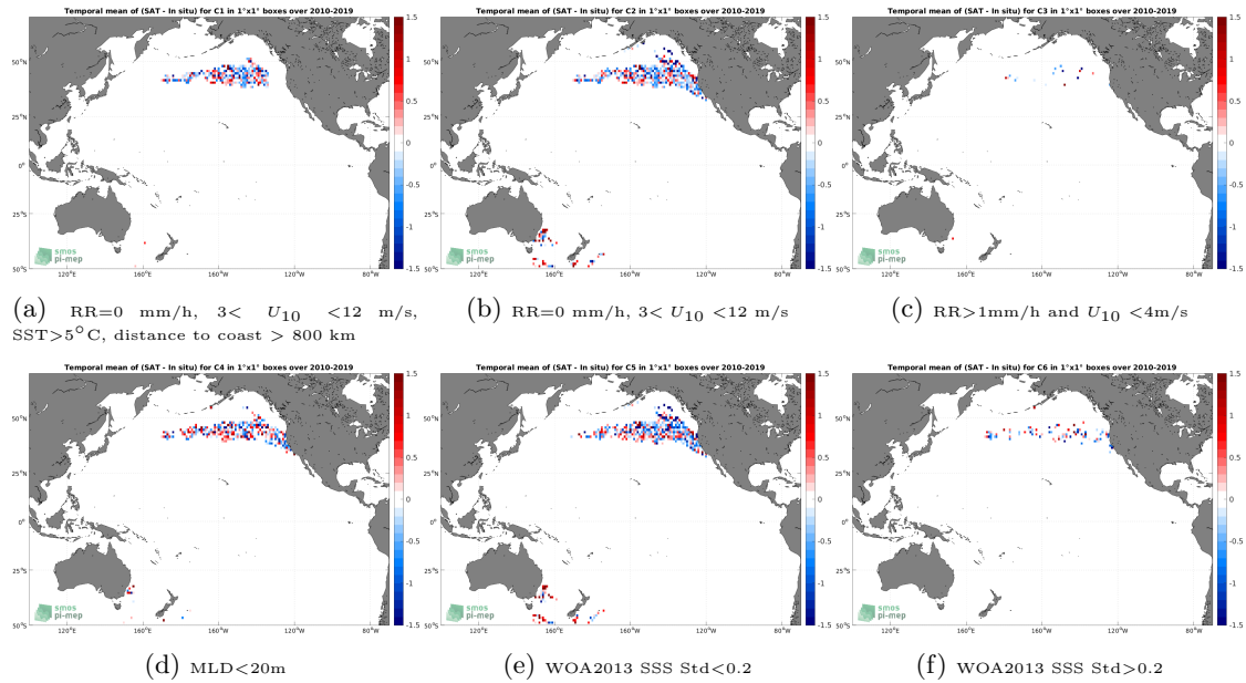
Figure 12: Temporal mean gridded over spatial boxes of size 1^{\circ}\times 1^{\circ} of \Delta\text{SSS} (SMOS SSS L2Q v331 - No FLAG (CMEMS-CATDS-CPDC) - Marine mammals) for 6 different subdatasets corresponding to:RR=0 mm/h, 3 < U_{10} < 12 m/s, SST >5^{\circ}\text{C} , distance to coast > 800 km (a), RR=0 mm/h, 3 < U_{10} < 12 m/s (b), RR >1 mm/h and U_{10} < 4 m/s (c),MLD <20 m (d),WOA2013 SSS Std <0.2 (e),WOA2013 SSS Std >0.2 (f).
