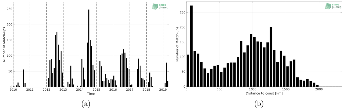
Figure 1: Number of match-ups between Marine mammals and SMOS SSS L2Q v331 - No FLAG (CMEMS-CATDS-CPDC) SSS as a function of time (a) and as function of the distance to coast (b) over the Pacific Ocean Pi-MEP region and for the full satellite product period.
