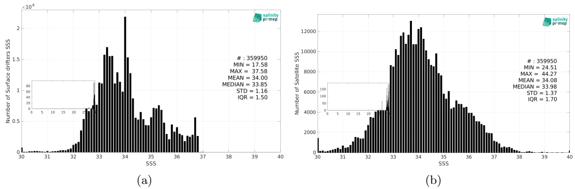
Figure 3: Histograms of SSS from Surface drifters (a) and SMOS SSS L2Q v331 - No FLAG (CMEMS-CATDS-CPDC) (b) considering all match-up pairs per bins of 0.1 over the Pacific Ocean Pi-MEP region and for the full satellite product period.
