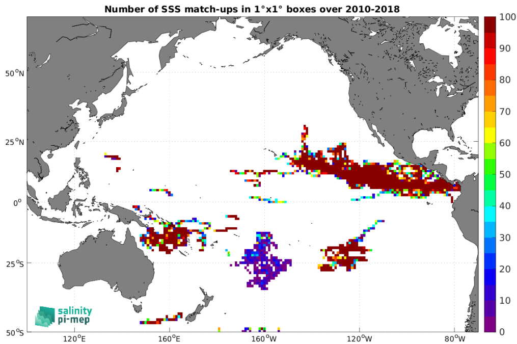
Figure 4: Number of SSS match-ups between Surface drifters SSS and the SMOS SSS L2Q v331 - No FLAG (CMEMS-CATDS-CPDC) SSS product for the Pacific Ocean Pi-MEP region over 1^\circ \times 1^\circ boxes and for the full satellite product period.
