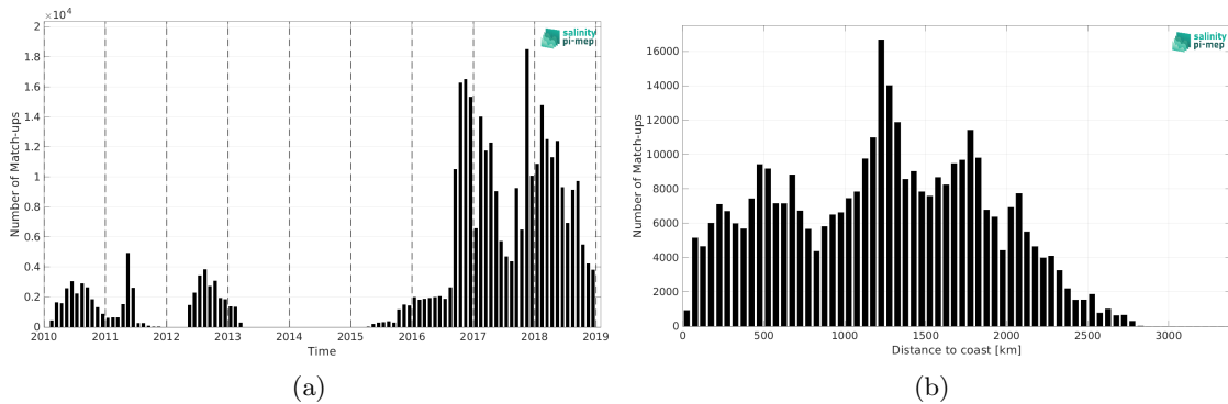
Figure 2: Number of match-ups between Surface drifters and SMOS SSS L2Q v331 - No FLAG (CMEMS-CATDS-CPDC) SSS as a function of time (a) and as function of the distance to coast (b) over the Pacific Ocean Pi-MEP region and for the full satellite product period.
