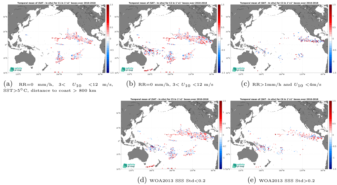
Figure 11: Temporal mean gridded over spatial boxes of size 1^\circ \times 1^\circ of \Delta\text{SSS} (SMOS SSS L2Q v331 - No FLAG (CMEMS-CATDS-CPDC) - Surface drifters) for 5 different subdatasets corresponding to:RR=0 mm/h, 3 < U_{10} < 12 m/s, SST >5^\circ\text{C} , distance to coast > 800 km (a), RR=0 mm/h, 3 < U_{10} < 12 m/s (b), RR >1 mm/h and U_{10} < 4 m/s (c), WOA2013 SSS Std <0.2 (d), WOA2013 SSS Std >0.2 (e).
