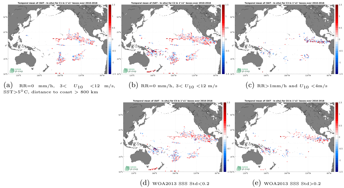
Figure 11: Temporal mean gridded over spatial boxes of size 1^\circ \times 1^\circ of \Delta SSS (SMOS SSS L2Q v331 - No FLAG (CMEMS-CATDS-CPDC) - Surface drifters) for 5 different subdatasets corresponding to:RR=0 mm/h, 3 < U_{10} < 12 m/s, SST >5^\circ C, distance to coast > 800 km (a), RR=0 mm/h, 3 < U_{10} < 12 m/s (b), RR >1 mm/h and U_{10} < 4 m/s (c), WOA2013 SSS Std <0.2 (d), WOA2013 SSS Std >0.2 (e).
