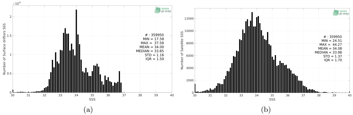
Figure 2: Histograms of SSS from Surface drifters (a) and SMOS SSS L2Q v331 - No FLAG (CMEMS-CATDS-CPDC) (b) considering all match-up pairs per bins of 0.1 over the Pacific Ocean Pi-MEP region and for the full satellite product period.
