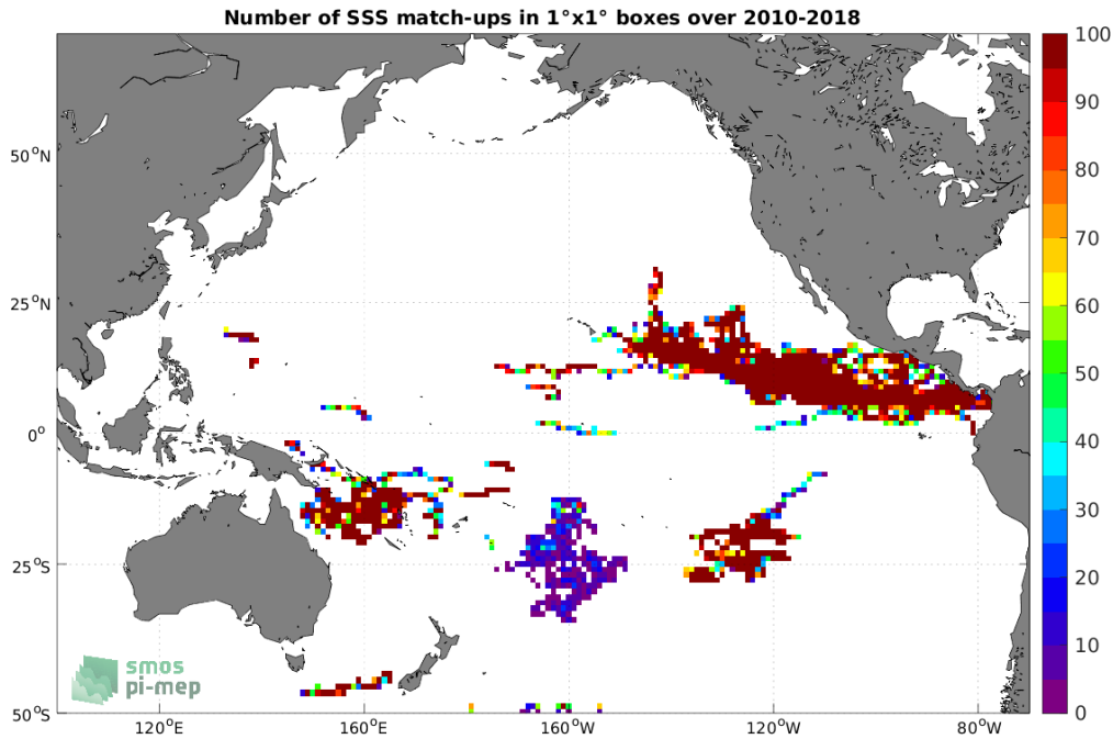
Figure 3: Number of SSS match-ups between Surface drifters SSS and the SMOS SSS L2Q v331 - No FLAG (CMEMS-CATDS-CPDC) SSS product for the Pacific Ocean Pi-MEP region over 1^\circ \times 1^\circ boxes and for the full satellite product period.
