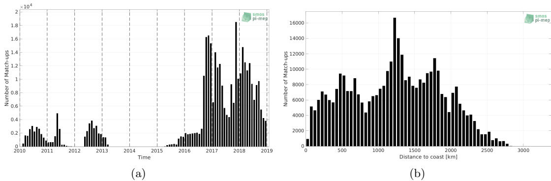
Figure 1: Number of match-ups between Surface drifters and SMOS SSS L2Q v331 - No FLAG (CMEMS-CATDS-CPDC) SSS as a function of time (a) and as function of the distance to coast (b) over the Pacific Ocean Pi-MEP region and for the full satellite product period.
