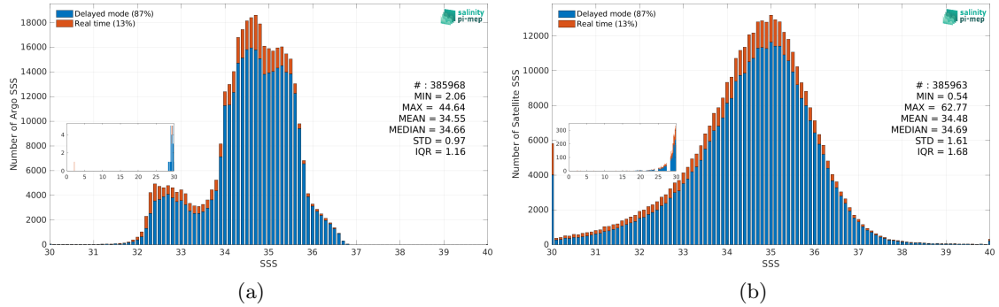
Figure 3: Histograms of SSS from Argo (a) and SMOS SSS L2Q v331 - No FLAG (CMEMS-CATDS-CPDC) (b) considering all match-up pairs per bins of 0.1 over the Pacific Ocean Pi-MEP region and for the full satellite product period.
