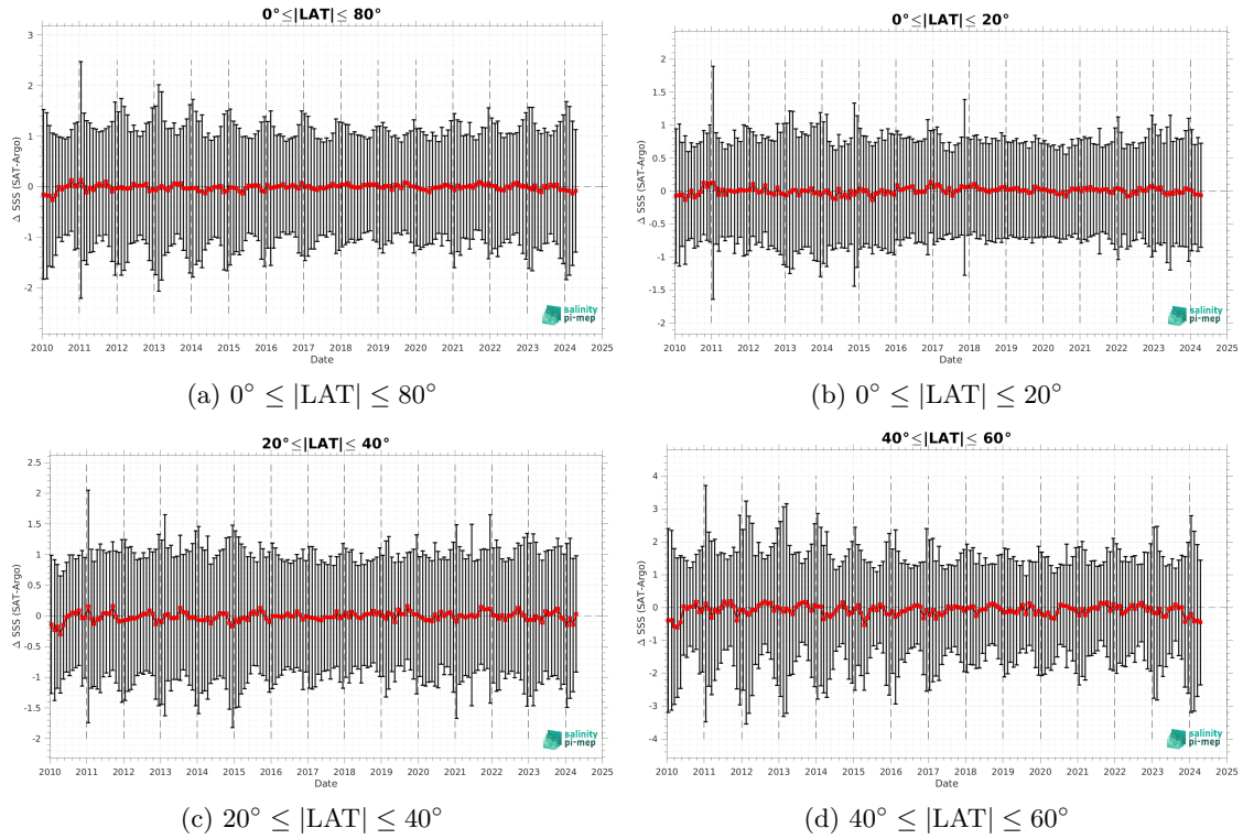
Figure 11: Monthly median (red curves) of \Delta SSS (Satellite - Argo) and \pm 1 Std (black vertical thick bars) as function of time for all the collected Pi-MEP match-up pairs estimated over the Pacific Ocean Pi-MEP region and for the full satellite product period are shown for different latitude bands: (a) 80°S-80°N, (b) 20°S-20°N, (c) 40°S-20°S and 20°N-40°N and (d) 60°S-40°S and 40°N-60°N.
