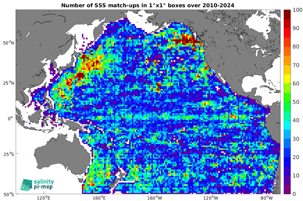
Figure 5: Number of SSS match-ups between Argo SSS and the SMOS SSS L2Q v331 - No FLAG (CMEMS-CATDS-CPDC) SSS product for the Pacific Ocean Pi-MEP region over 1^\circ \times 1^\circ boxes and for the full satellite product period.
