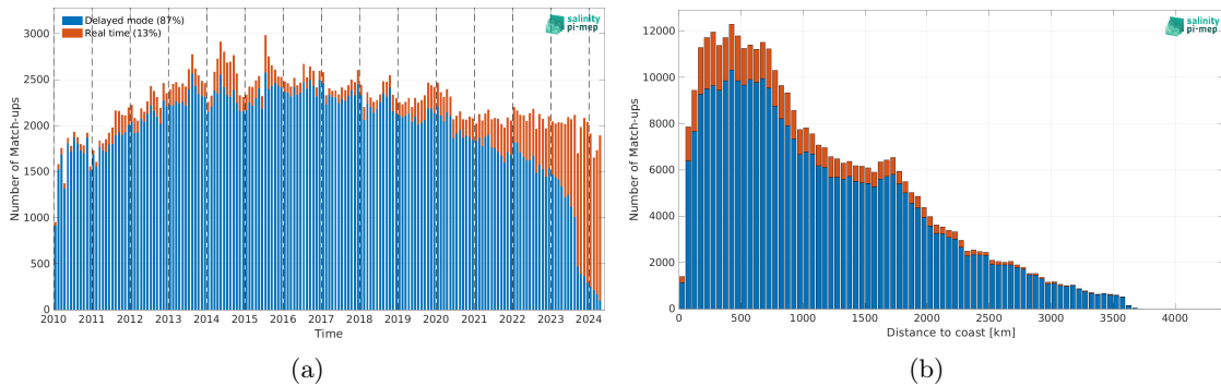
Figure 2: Number of match-ups between Argo and SMOS SSS L2Q v331 - No FLAG (CMEMS-CATDS-CPDC) SSS as a function of time (a) and as function of the distance to coast (b) over the Pacific Ocean Pi-MEP region and for the full satellite product period.
