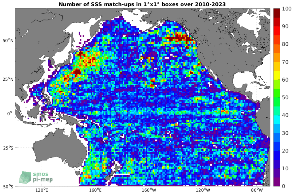
Figure 4: Number of SSS match-ups between Argo SSS and the SMOS SSS L2Q v331 - No FLAG (CMEMS-CATDS-CPDC) SSS product for the Pacific Ocean Pi-MEP region over 1^\circ \times 1^\circ boxes and for the full satellite product period.
