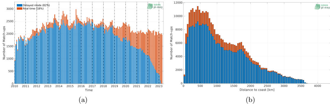
Figure 1: Number of match-ups between Argo and SMOS SSS L2Q v331 - No FLAG (CMEMS-CATDS-CPDC) SSS as a function of time (a) and as function of the distance to coast (b) over the Pacific Ocean Pi-MEP region and for the full satellite product period.
