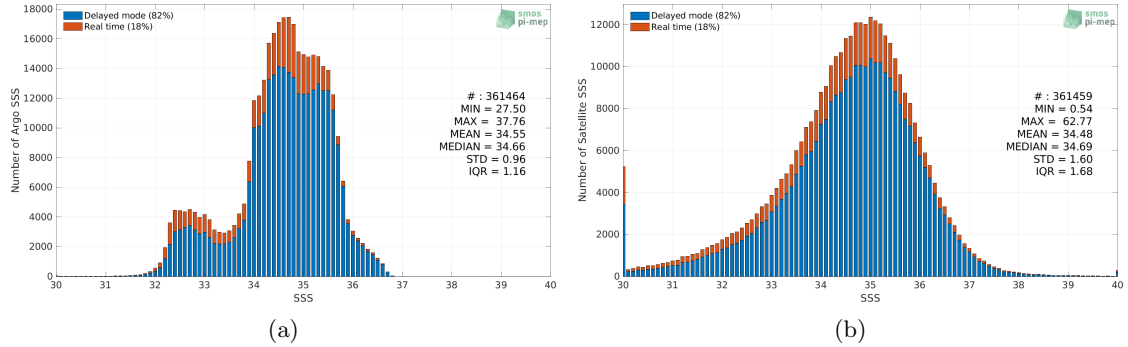
Figure 2: Histograms of SSS from Argo (a) and SMOS SSS L2Q v331 - No FLAG (CMEMS-CATDS-CPDC) (b) considering all match-up pairs per bins of 0.1 over the Pacific Ocean Pi-MEP region and for the full satellite product period.
