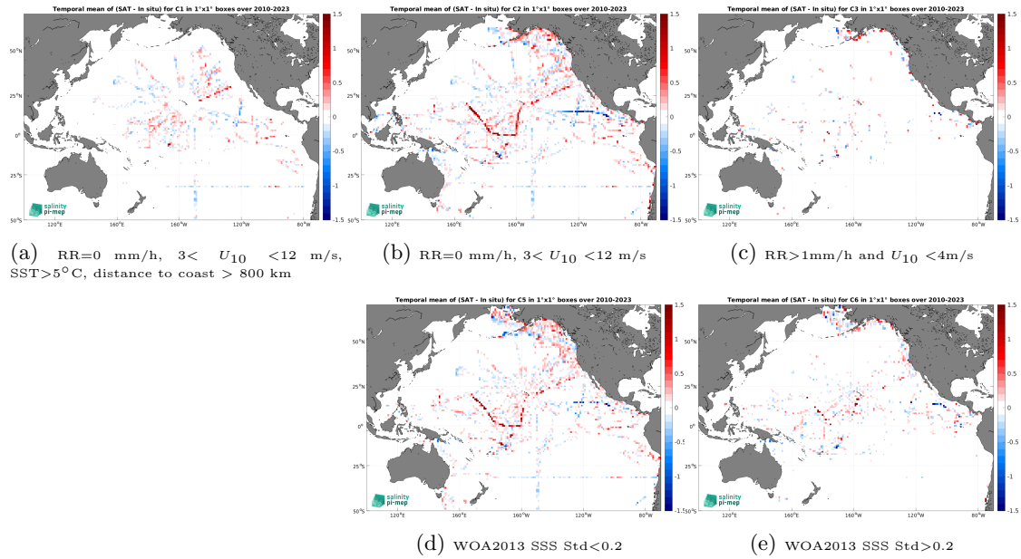
Figure 12: Temporal mean gridded over spatial boxes of size 1^\circ \times 1^\circ of \Delta\text{SSS} (SMOS SSS L3 v9 - 9 Days (CATDS-CEC-LOCEAN) - TSG (SAMOS)) for 5 different subdatasets corresponding to:RR=0 mm/h, 3 < U_{10} < 12 m/s, SST >5^\circ\text{C} , distance to coast > 800 km (a), RR=0 mm/h, 3 < U_{10} < 12 m/s (b), RR >1 mm/h and U_{10} < 4 m/s (c), WOA2013 SSS Std <0.2 (d), WOA2013 SSS Std >0.2 (e).
