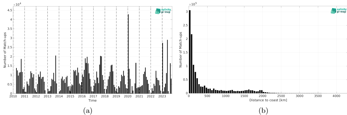
Figure 1: Number of match-ups between TSG (SAMOS) and SMOS SSS L3 v9 - 9 Days (CATDS-CEC-LOCEAN) SSS as a function of time (a) and as function of the distance to coast (b) over the Pacific Ocean Pi-MEP region and for the full satellite product period.
