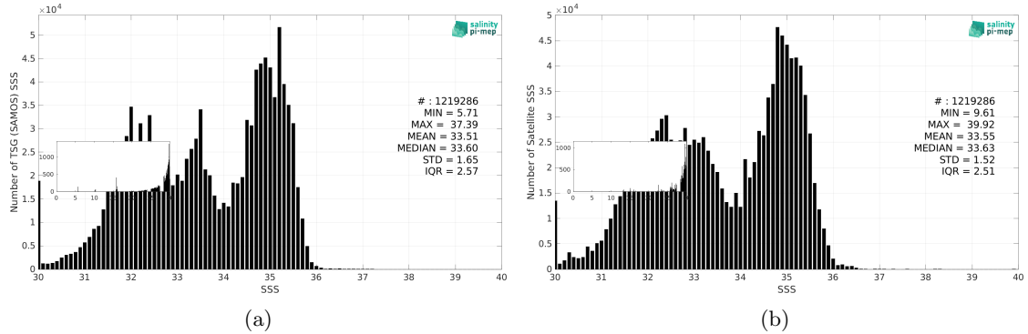
Figure 2: Histograms of SSS from TSG (SAMOS) (a) and SMOS SSS L3 v9 - 9 Days (CATDS-CEC-LOCEAN) (b) considering all match-up pairs per bins of 0.1 over the Pacific Ocean Pi-MEP region and for the full satellite product period.
