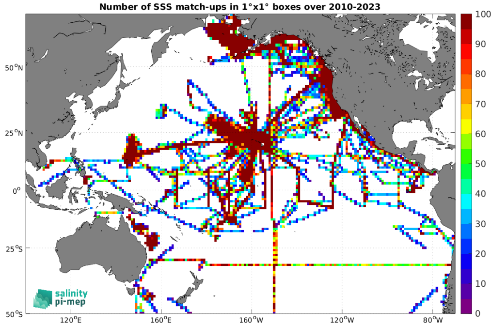
Figure 4: Number of SSS match-ups between TSG (SAMOS) SSS and the SMOS SSS L3 v9 - 9 Days (CATDS-CEC-LOCEAN) SSS product for the Pacific Ocean Pi-MEP region over 1^\circ \times 1^\circ boxes and for the full satellite product period.
