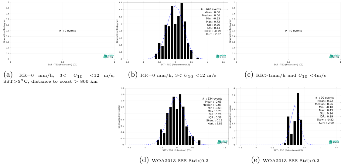
Figure 15: Normalized histogram of \Delta SSS (SMOS SSS L3 v9 - 9 Days (CATDS-CEC-LOCEAN) - TSG (Polarstern)) for 5 different subdatasets corresponding to: RR=0 mm/h, 3 < U_{10} < 12 m/s, SST > 5°C, distance to coast > 800 km (a), RR=0 mm/h, 3 < U_{10} < 12 m/s (b), RR > 1mm/h and U_{10} < 4 m/s (c), WOA2013 SSS Std < 0.2 (d), WOA2013 SSS Std > 0.2 (e).
