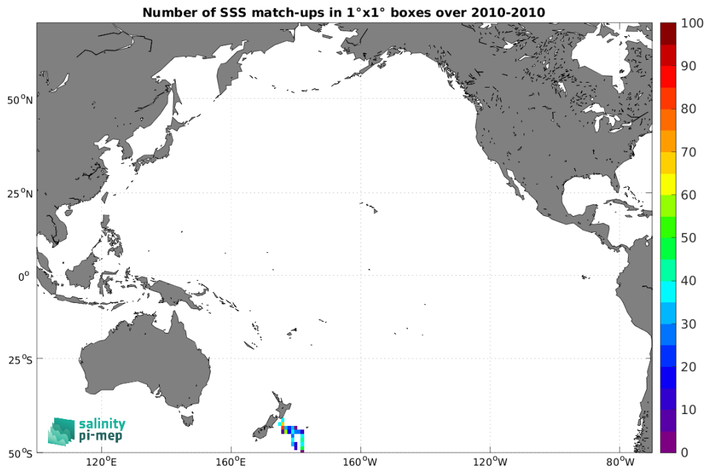
Figure 5: Number of SSS match-ups between TSG (Polarstern) SSS and the SMOS SSS L3 v9 - 9 Days (CATDS-CEC-LOCEAN) SSS product for the Pacific Ocean Pi-MEP region over 1^\circ \times 1^\circ boxes and for the full satellite product period.
