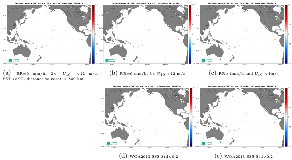
Figure 14: Temporal mean gridded over spatial boxes of size 1^\circ \times 1^\circ of \Delta\text{SSS} (SMOS SSS L3 v9 - 9 Days (CATDS-CEC-LOCEAN) - TSG (Polarstern)) for 5 different subdatasets corresponding to:RR=0 mm/h, 3 < U_{10} < 12 m/s, SST > 5^\circ\text{C} , distance to coast > 800 km (a), RR=0 mm/h, 3 < U_{10} < 12 m/s (b), RR > 1 mm/h and U_{10} < 4 m/s (c), WOA2013 SSS Std < 0.2 (d), WOA2013 SSS Std > 0.2 (e).
