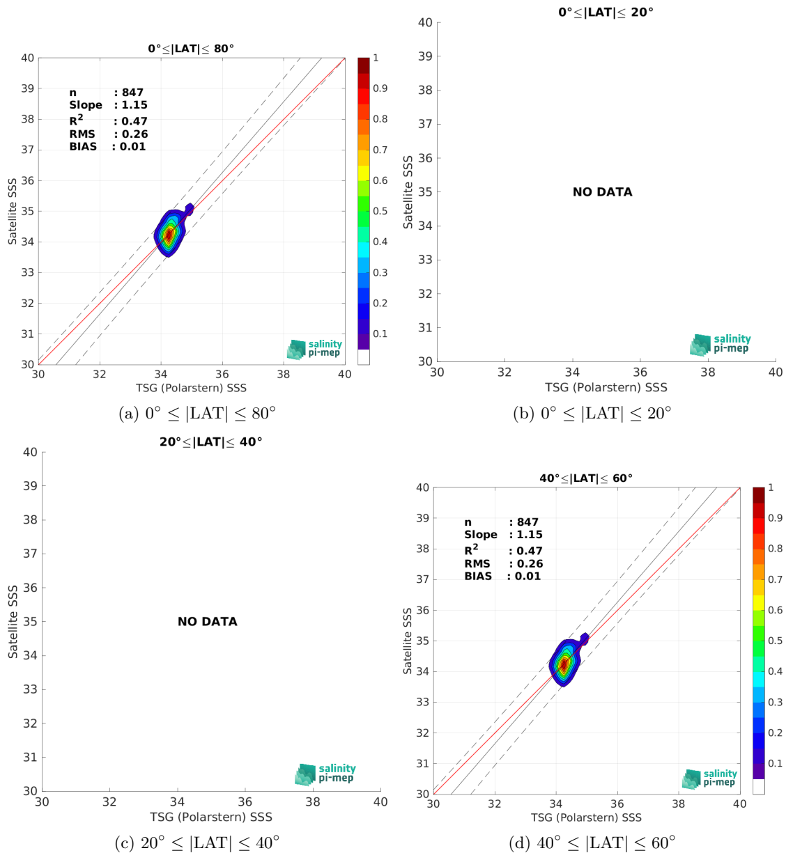
Figure 10: Contour maps of the concentration of SMOS SSS L3 v9 - 9 Days (CATDS-CEC-LOCEAN) SSS (y-axis) versus TSG (Polarstern) SSS (x-axis) at match-up pairs for different latitude bands. For each plot, the red line shows x=y . The black thin and dashed lines indicate a linear fit through the data cloud and the \pm 95\% confidence levels, respectively. The number of match-up pairs n , the slope and R^2 coefficient of the linear fit, the root mean square (RMS) and the mean bias between satellite and in situ data are indicated for each latitude band in each plot.
