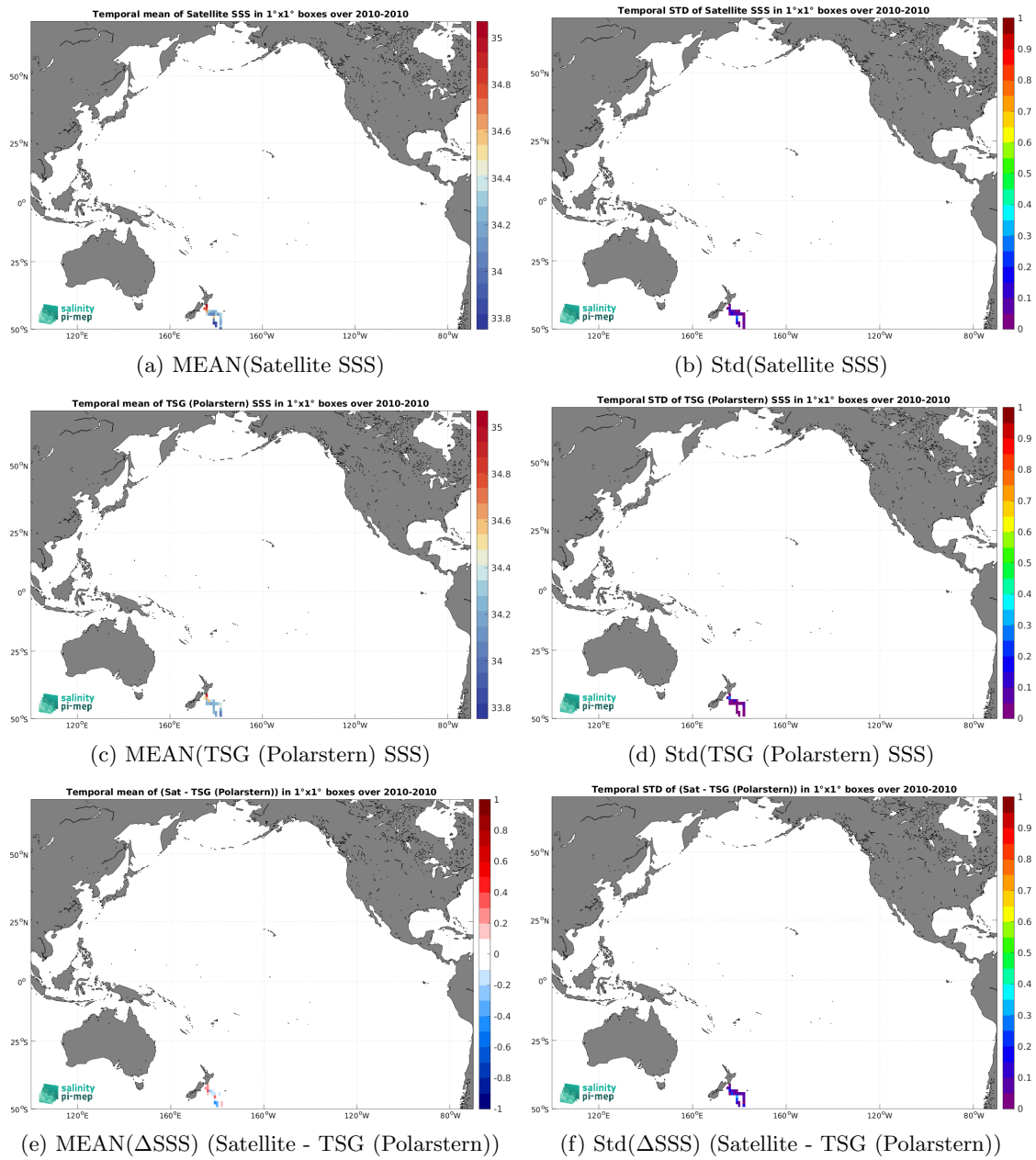
Figure 7: Temporal mean (left) and Std (right) of SSS from SMOS SSS L3 v9 - 9 Days (CATDS-CEC-LOCEAN) (top), TSG (Polarstern) (middle), and of \Delta SSS (Satellite - TSG (Polarstern)). Only match-up pairs are used to generate these maps.
