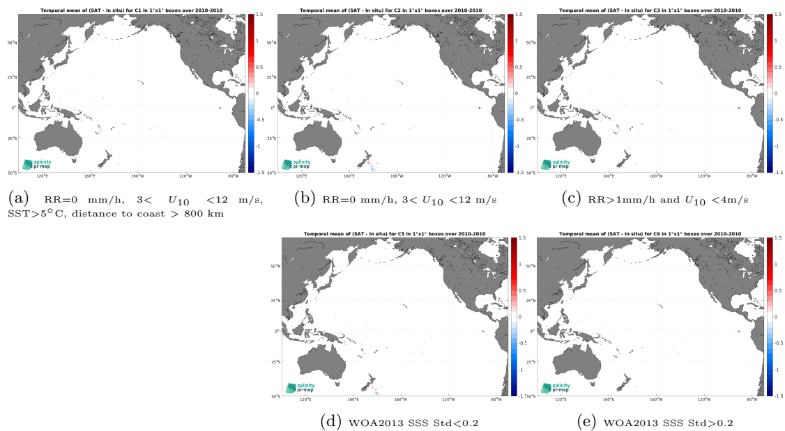
Figure 14: Temporal mean gridded over spatial boxes of size 1^\circ \times 1^\circ of \Delta SSS (SMOS SSS L3 v9 - 9 Days (CATDS-CEC-LOCEAN) - TSG (Polarstern)) for 5 different subdatasets corresponding to: RR=0 mm/h, 3 < U_{10} < 12 m/s, SST > 5^\circ\text{C} , distance to coast > 800 km (a), RR=0 mm/h, 3 < U_{10} < 12 m/s (b), RR > 1 mm/h and U_{10} < 4 m/s (c), WOA2013 SSS Std < 0.2 (d), WOA2013 SSS Std > 0.2 (e).
