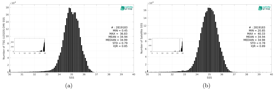
Figure 3: Histograms of SSS from TSG (LEGOS-DM) (a) and SMOS SSS L3 v9 - 9 Days (CATDS-CEC-LOCEAN) (b) considering all match-up pairs per bins of 0.1 over the Pacific Ocean Pi-MEP region and for the full satellite product period.
