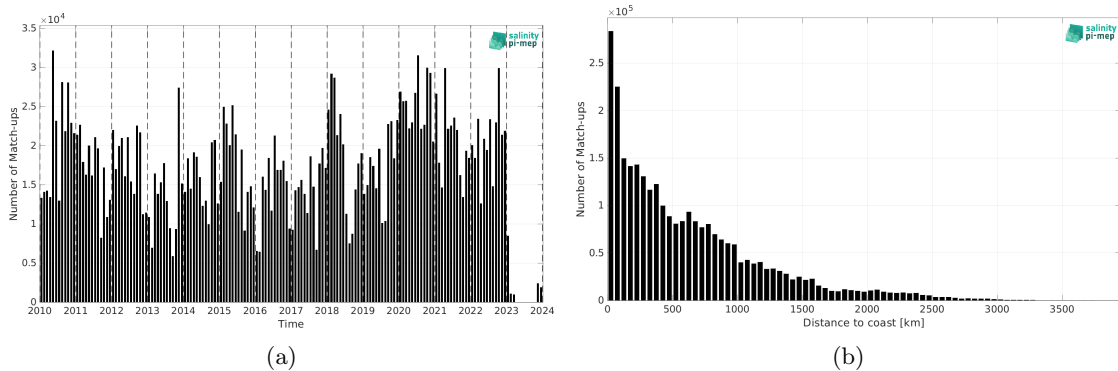
Figure 2: Number of match-ups between TSG (LEGOS-DM) and SMOS SSS L3 v9 - 9 Days (CATDS-CEC-LOCEAN) SSS as a function of time (a) and as function of the distance to coast (b) over the Pacific Ocean Pi-MEP region and for the full satellite product period.
