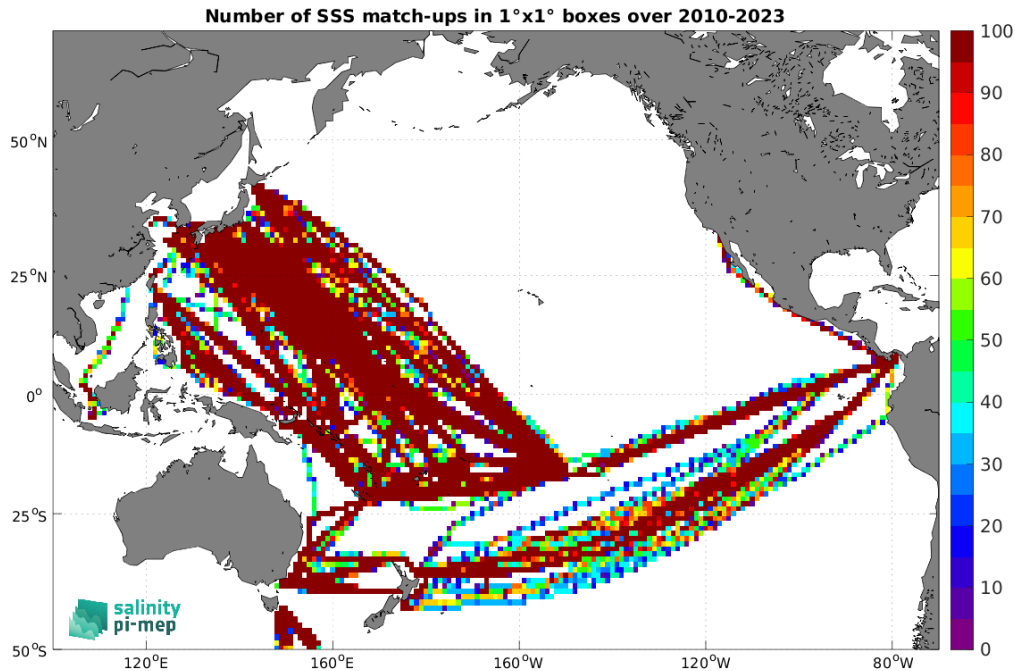
Figure 5: Number of SSS match-ups between TSG (LEGOS-DM) SSS and the SMOS SSS L3 v9 - 9 Days (CATDS-CEC-LOCEAN) SSS product for the Pacific Ocean Pi-MEP region over 1^\circ \times 1^\circ boxes and for the full satellite product period.
