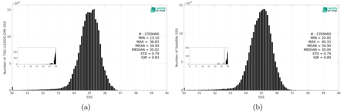
Figure 2: Histograms of SSS from TSG (LEGOS-DM) (a) and SMOS SSS L3 v9 - 9 Days (CATDS-CEC-LOCEAN) (b) considering all match-up pairs per bins of 0.1 over the Pacific Ocean Pi-MEP region and for the full satellite product period.
