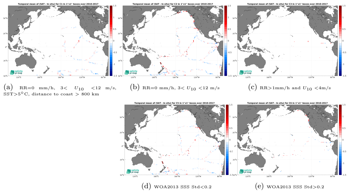
Figure 14: Temporal mean gridded over spatial boxes of size 1^\circ \times 1^\circ of \Delta SSS (SMOS SSS L3 v9 - 9 Days (CATDS-CEC-LOCEAN) - TSG (GOSUD-Sailing-ship)) for 5 different subdatasets corresponding to:RR=0 mm/h, 3 < U_{10} < 12 m/s, SST >5^\circ C, distance to coast > 800 km (a), RR=0 mm/h, 3 < U_{10} < 12 m/s (b), RR >1 mm/h and U_{10} < 4 m/s (c), WOA2013 SSS Std <0.2 (d), WOA2013 SSS Std >0.2 (e).
