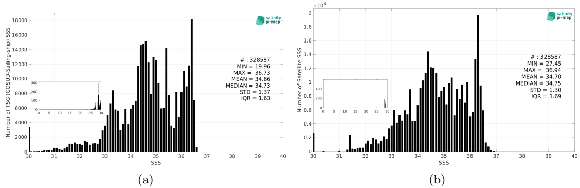
Figure 3: Histograms of SSS from TSG (GOSUD-Sailing-ship) (a) and SMOS SSS L3 v9 - 9 Days (CATDS-CEC-LOCEAN) (b) considering all match-up pairs per bins of 0.1 over the Pacific Ocean Pi-MEP region and for the full satellite product period.
