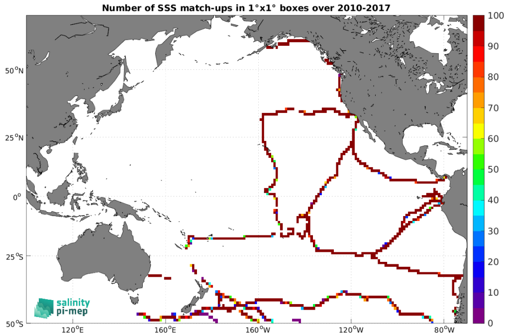
Figure 4: Number of SSS match-ups between TSG (GOSUD-Sailing-ship) SSS and the SMOS SSS L3 v9 - 9 Days (CATDS-CEC-LOCEAN) SSS product for the Pacific Ocean Pi-MEP region over 1^\circ \times 1^\circ boxes and for the full satellite product period.
