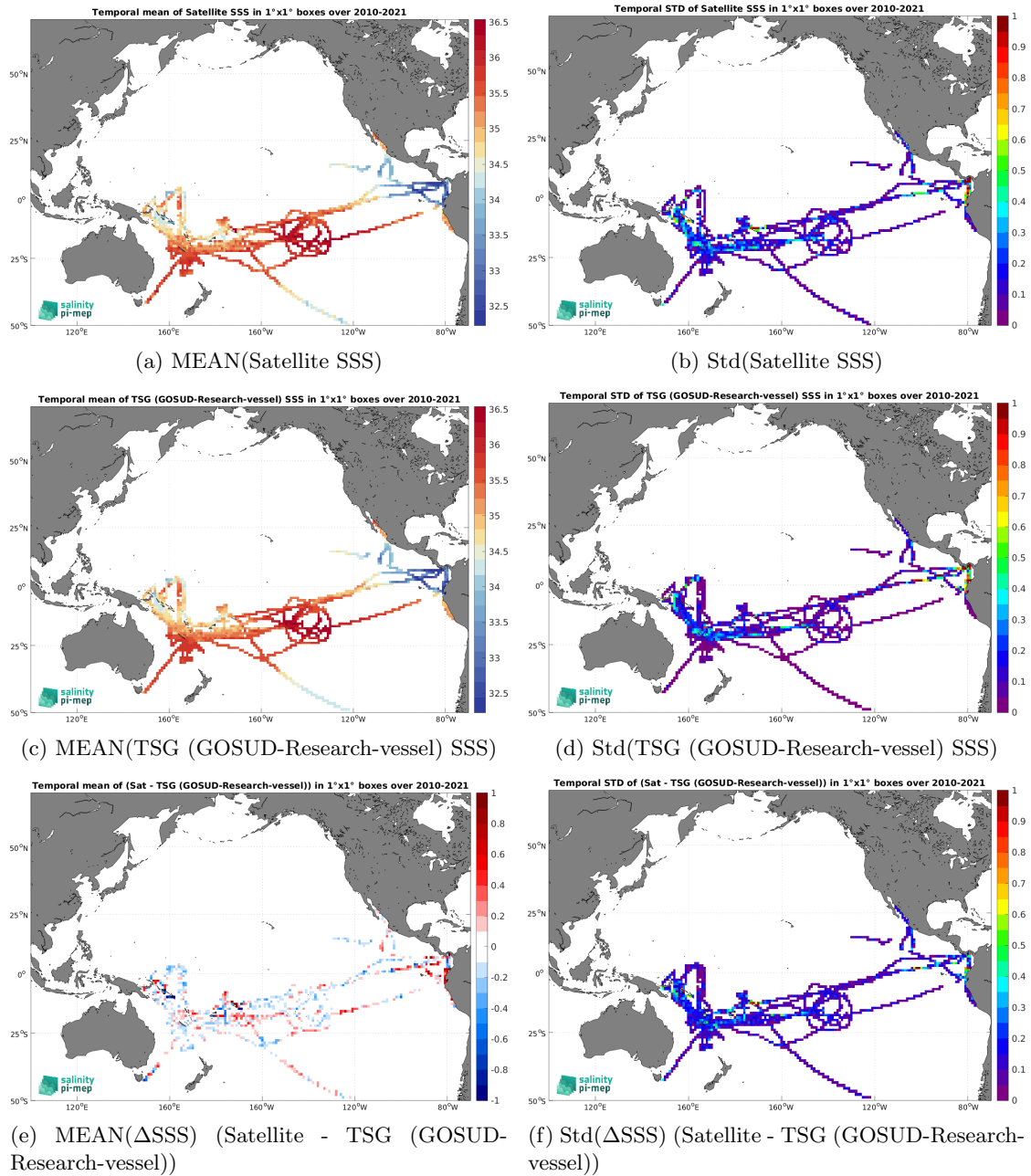
Figure 7: Temporal mean (left) and Std (right) of SSS from SMOS SSS L3 v9 - 9 Days (CATDS-CEC-LOCEAN) (top), TSG (GOSUD-Research-vessel) (middle), and of \Delta SSS (Satellite - TSG (GOSUD-Research-vessel)). Only match-up pairs are used to generate these maps.
