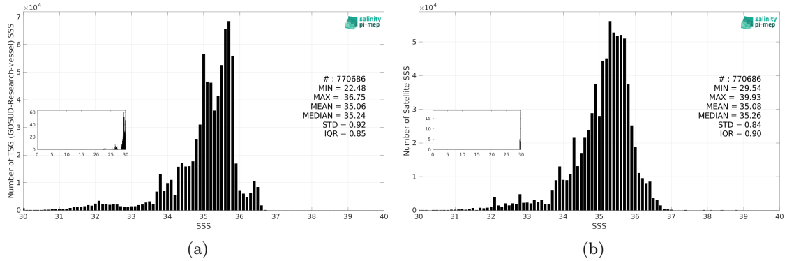
Figure 3: Histograms of SSS from TSG (GOSUD-Research-vessel) (a) and SMOS SSS L3 v9 - 9 Days (CATDS-CEC-LOCEAN) (b) considering all match-up pairs per bins of 0.1 over the Pacific Ocean Pi-MEP region and for the full satellite product period.
