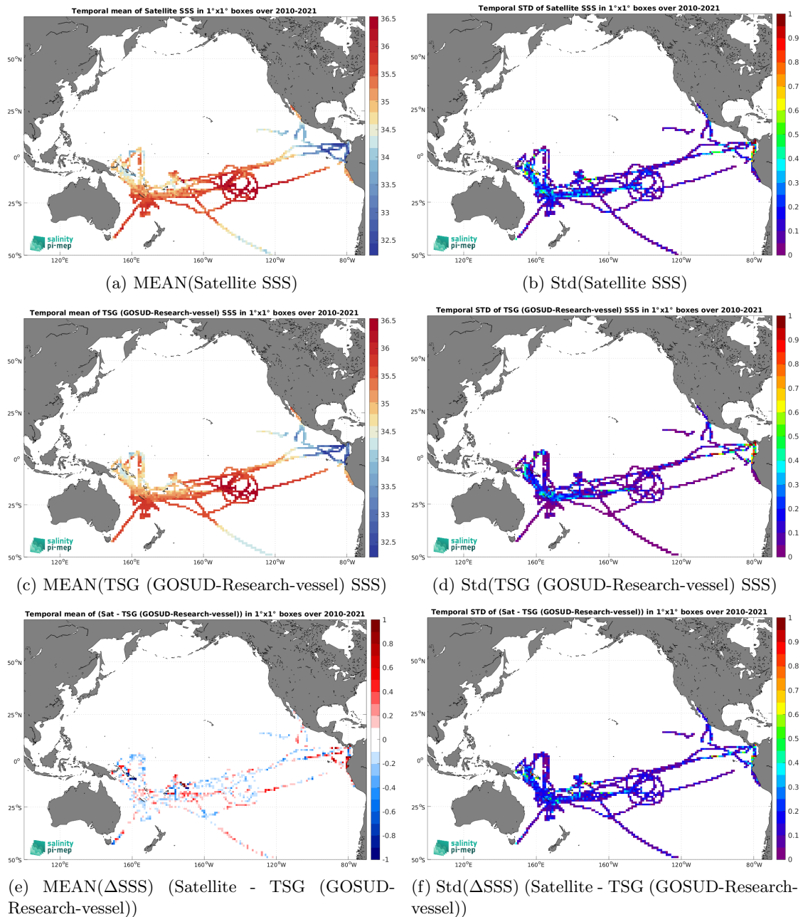
Figure 6: Temporal mean (left) and Std (right) of SSS from SMOS SSS L3 v9 - 9 Days (CATDS-CEC-LOCEAN) (top), TSG (GOSUD-Research-vessel) (middle), and of \Delta SSS (Satellite - TSG (GOSUD-Research-vessel)). Only match-up pairs are used to generate these maps.
