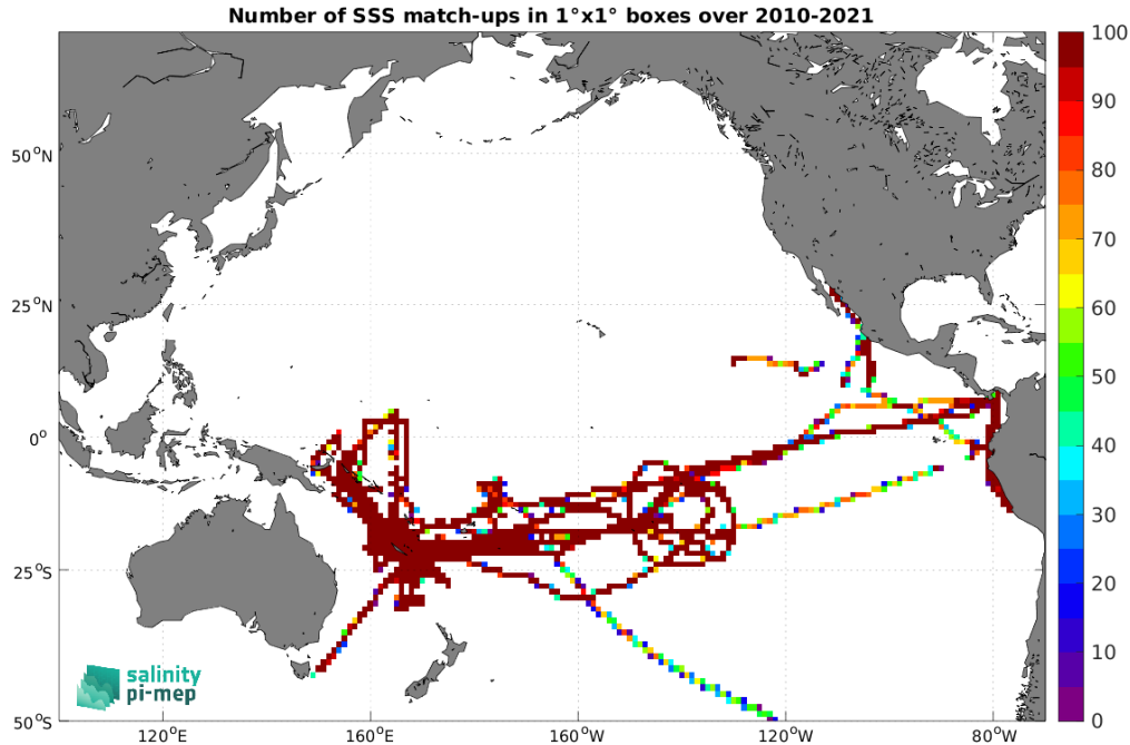
Figure 4: Number of SSS match-ups between TSG (GOSUD-Research-vessel) SSS and the SMOS SSS L3 v9 - 9 Days (CATDS-CEC-LOCEAN) SSS product for the Pacific Ocean Pi-MEP region over 1^\circ \times 1^\circ boxes and for the full satellite product period.
