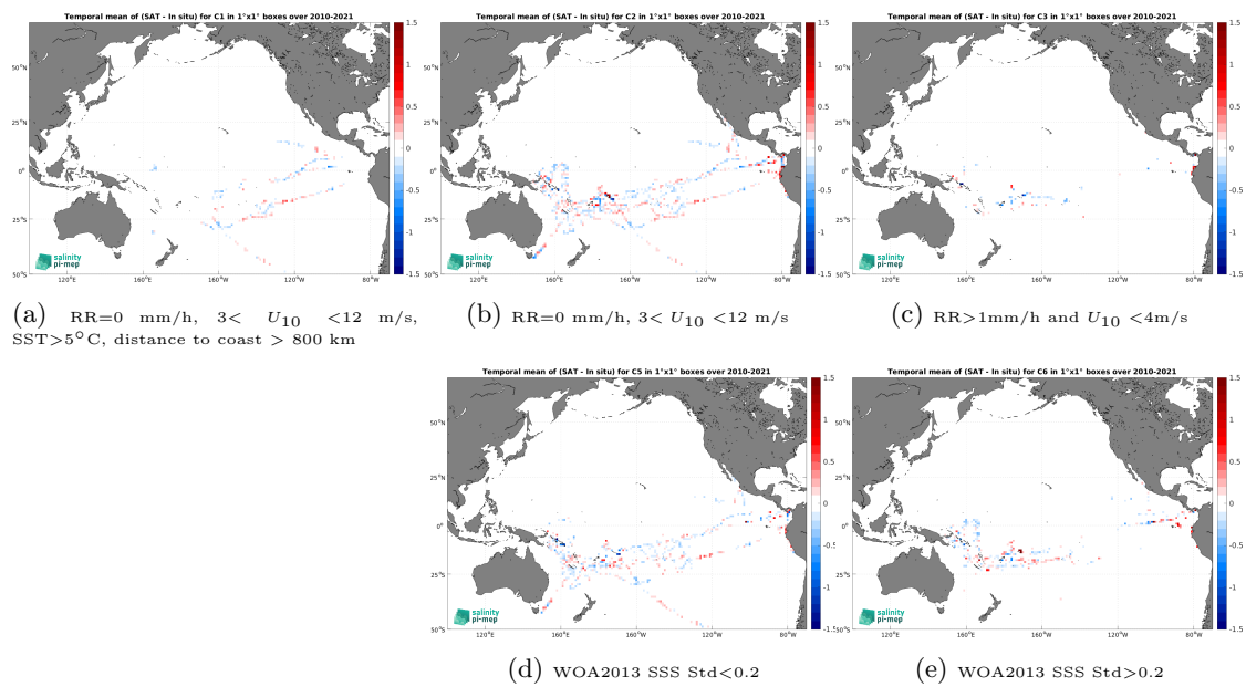
Figure 12: Temporal mean gridded over spatial boxes of size 1^\circ \times 1^\circ of \Delta SSS (SMOS SSS L3 v9 - 9 Days (CATDS-CEC-LOCEAN) - TSG (GOSUD-Research-vessel)) for 5 different subdatasets corresponding to:RR=0 mm/h, 3 < U_{10} < 12 m/s, SST >5^\circ C, distance to coast > 800 km (a), RR=0 mm/h, 3 < U_{10} < 12 m/s (b), RR >1 mm/h and U_{10} < 4 m/s (c), WOA2013 SSS Std <0.2 (d), WOA2013 SSS Std >0.2 (e).
