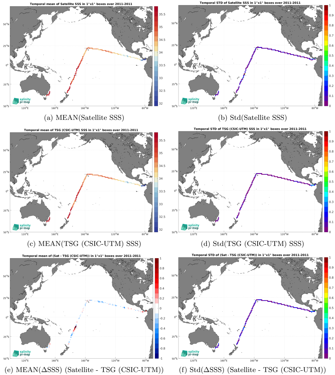
Figure 6: Temporal mean (left) and Std (right) of SSS from SMOS SSS L3 v9 - 9 Days (CATDS-CEC-LOCEAN) (top), TSG (CSIC-UTM) (middle), and of \Delta SSS (Satellite - TSG (CSIC-UTM)). Only match-up pairs are used to generate these maps.
