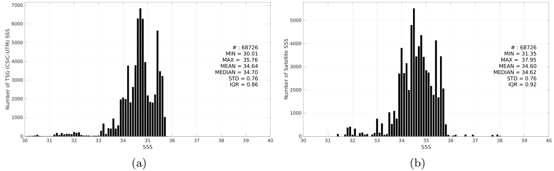
Figure 2: Histograms of SSS from TSG (CSIC-UTM) (a) and SMOS SSS L3 v9 - 9 Days (CATDS-CEC-LOCEAN) (b) considering all match-up pairs per bins of 0.1 over the Pacific Ocean Pi-MEP region and for the full satellite product period.
