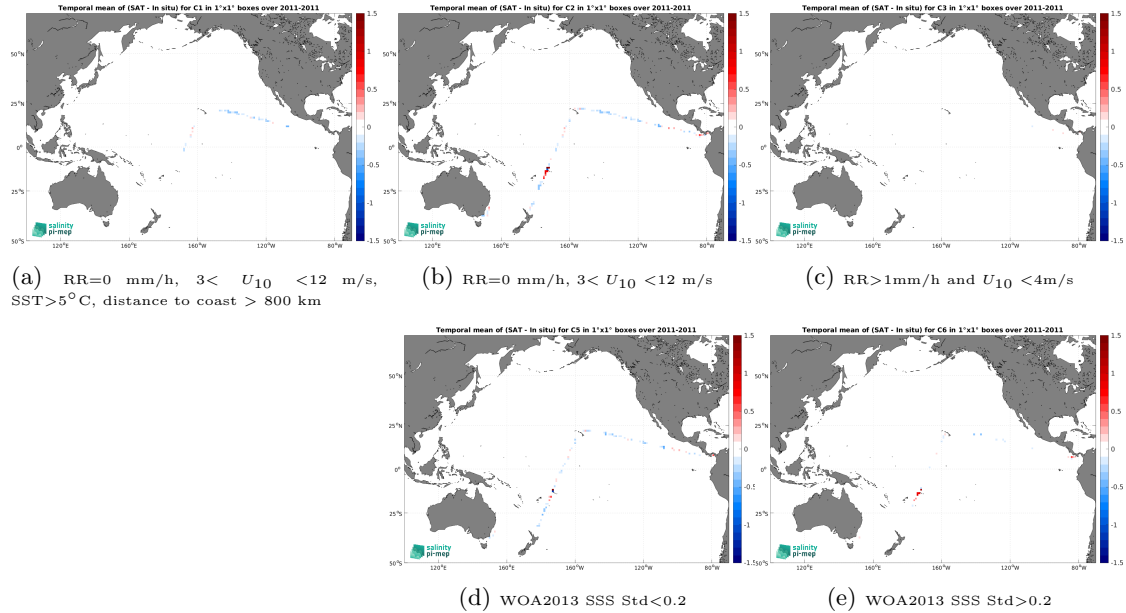
Figure 12: Temporal mean gridded over spatial boxes of size 1^{\circ}\times 1^{\circ} of \Delta\text{SSS} (SMOS SSS L3 v9 - 9 Days (CATDS-CEC-LOCEAN) - TSG (CSIC-UTM)) for 5 different subdatasets corresponding to:RR=0 mm/h, 3 < U_{10} < 12 m/s, SST >5^{\circ}\text{C} , distance to coast > 800 km (a), RR=0 mm/h, 3 < U_{10} < 12 m/s (b), RR >1 mm/h and U_{10} < 4 m/s (c), WOA2013 SSS Std <0.2 (d), WOA2013 SSS Std >0.2 (e).
