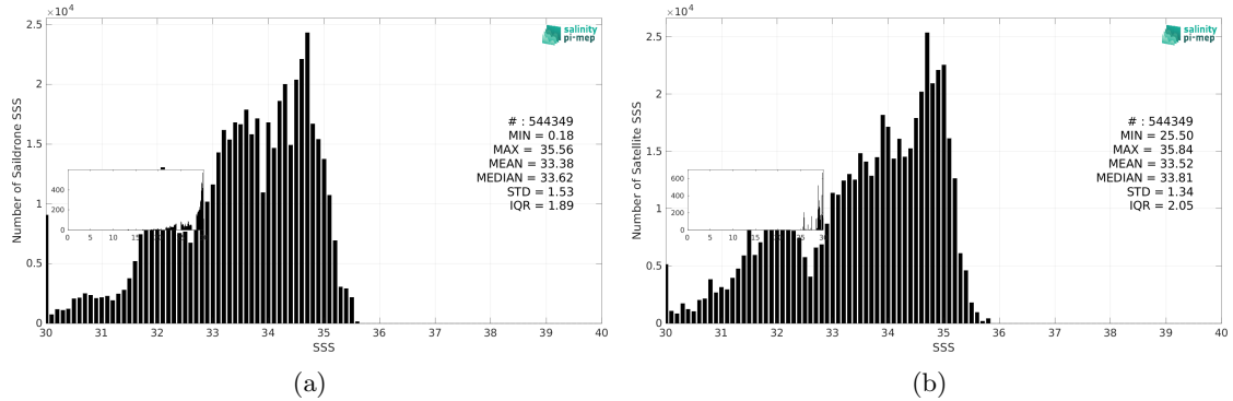
Figure 2: Histograms of SSS from Saildrone (a) and SMOS SSS L3 v9 - 9 Days (CATDS-CEC-LOCEAN) (b) considering all match-up pairs per bins of 0.1 over the Pacific Ocean Pi-MEP region and for the full satellite product period.
