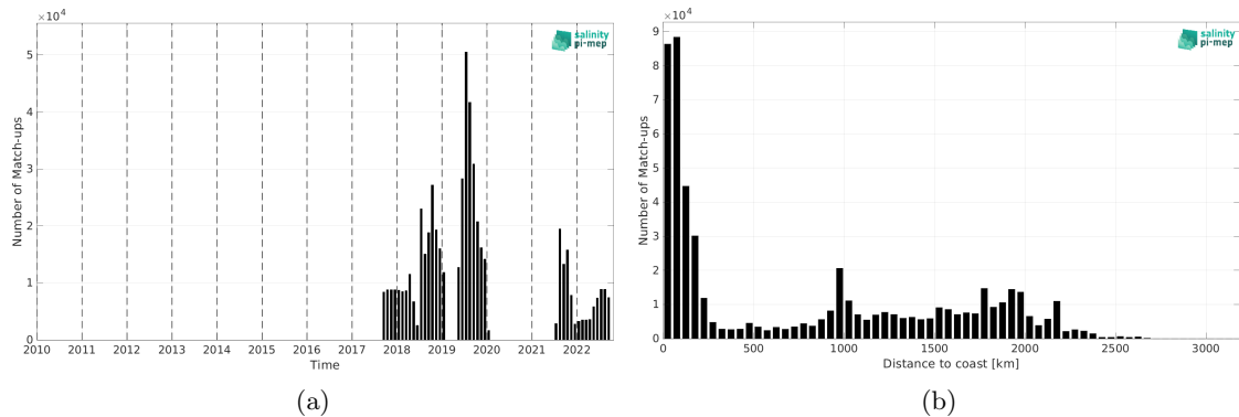
Figure 1: Number of match-ups between Saildrone and SMOS SSS L3 v9 - 9 Days (CATDS-CEC-LOCEAN) SSS as a function of time (a) and as function of the distance to coast (b) over the Pacific Ocean Pi-MEP region and for the full satellite product period.
