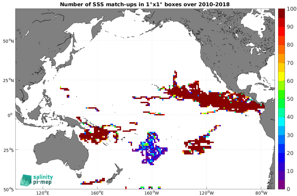
Figure 4: Number of SSS match-ups between Surface drifters SSS and the SMOS SSS L3 v9 - 9 Days (CATDS-CEC-LOCEAN) SSS product for the Pacific Ocean Pi-MEP region over 1^\circ \times 1^\circ boxes and for the full satellite product period.
