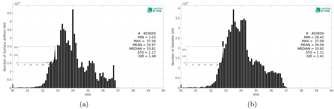
Figure 3: Histograms of SSS from Surface drifters (a) and SMOS SSS L3 v9 - 9 Days (CATDS-CEC-LOCEAN) (b) considering all match-up pairs per bins of 0.1 over the Pacific Ocean Pi-MEP region and for the full satellite product period.
