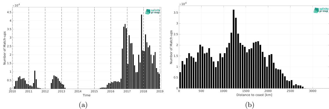
Figure 2: Number of match-ups between Surface drifters and SMOS SSS L3 v9 - 9 Days (CATDS-CEC-LOCEAN) SSS as a function of time (a) and as function of the distance to coast (b) over the Pacific Ocean Pi-MEP region and for the full satellite product period.
