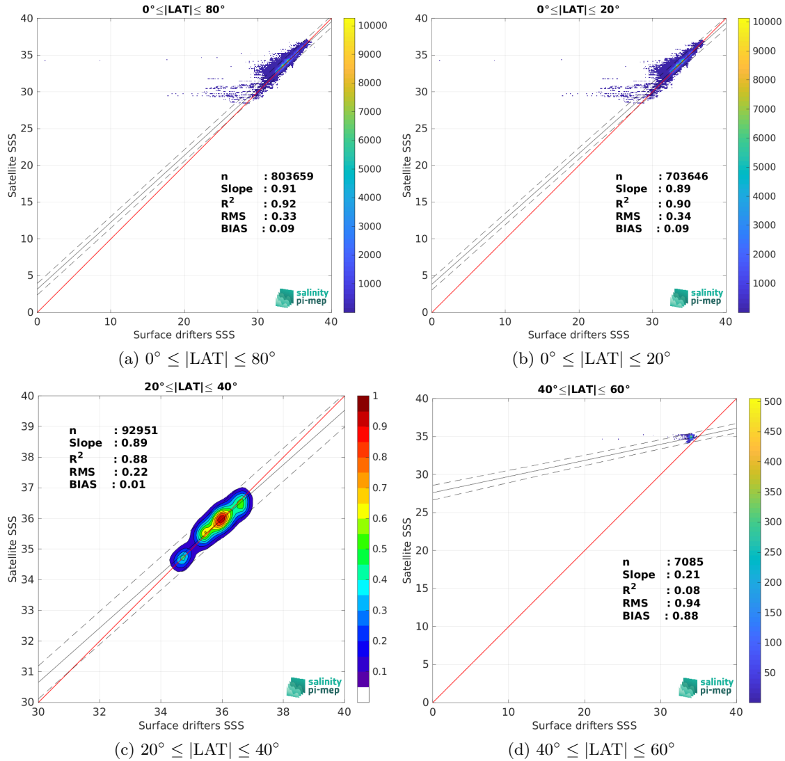
Figure 9: Contour maps of the concentration of SMOS SSS L3 v9 - 9 Days (CATDS-CEC-LOCEAN) SSS (y-axis) versus Surface drifters SSS (x-axis) at match-up pairs for different latitude bands. For each plot, the red line shows x=y . The black thin and dashed lines indicate a linear fit through the data cloud and the \pm 95\% confidence levels, respectively. The number match-up pairs n , the slope and R^2 coefficient of the linear fit, the root mean square (RMS) and the mean bias between satellite and in situ data are indicated for each latitude band in each plots.
