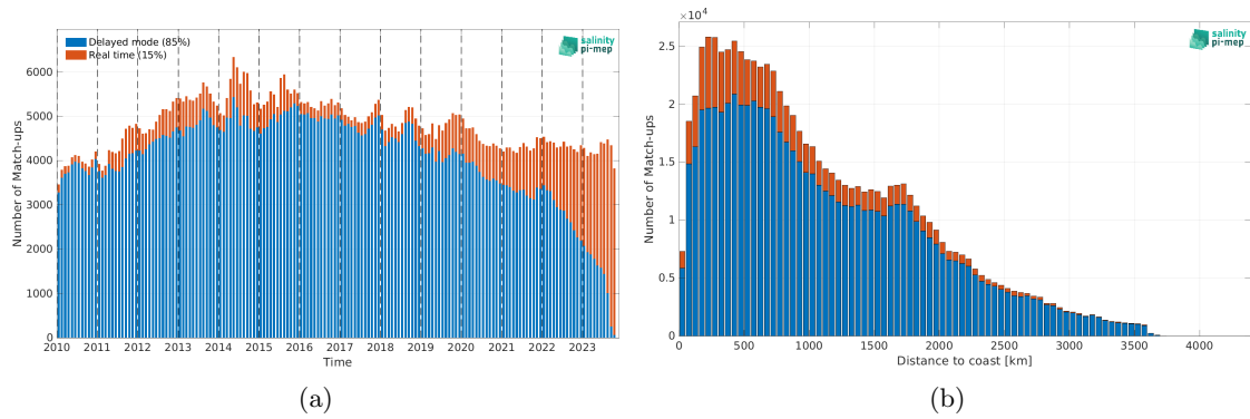
Figure 1: Number of match-ups between Argo and SMOS SSS L3 v9 - 9 Days (CATDS-CEC-LOCEAN) SSS as a function of time (a) and as function of the distance to coast (b) over the Pacific Ocean Pi-MEP region and for the full satellite product period.
