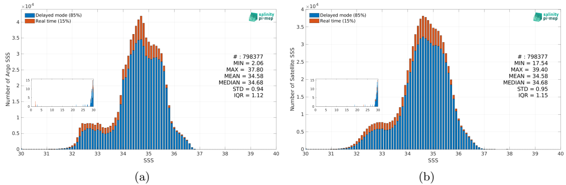
Figure 2: Histograms of SSS from Argo (a) and SMOS SSS L3 v9 - 9 Days (CATDS-CEC-LOCEAN) (b) considering all match-up pairs per bins of 0.1 over the Pacific Ocean Pi-MEP region and for the full satellite product period.
