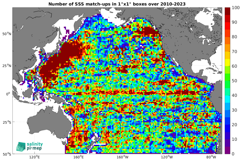
Figure 4: Number of SSS match-ups between Argo SSS and the SMOS SSS L3 v9 - 9 Days (CATDS-CEC-LOCEAN) SSS product for the Pacific Ocean Pi-MEP region over 1^\circ \times 1^\circ boxes and for the full satellite product period.
