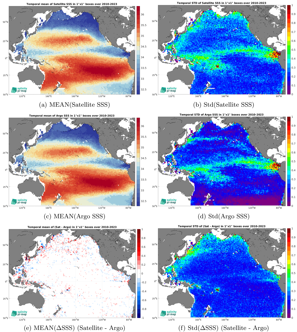
Figure 6: Temporal mean (left) and Std (right) of SSS from SMOS SSS L3 v9 - 9 Days (CATDS-CEC-LOCEAN) (top), Argo (middle), and of \Delta SSS (Satellite - Argo). Only match-up pairs are used to generate these maps.
