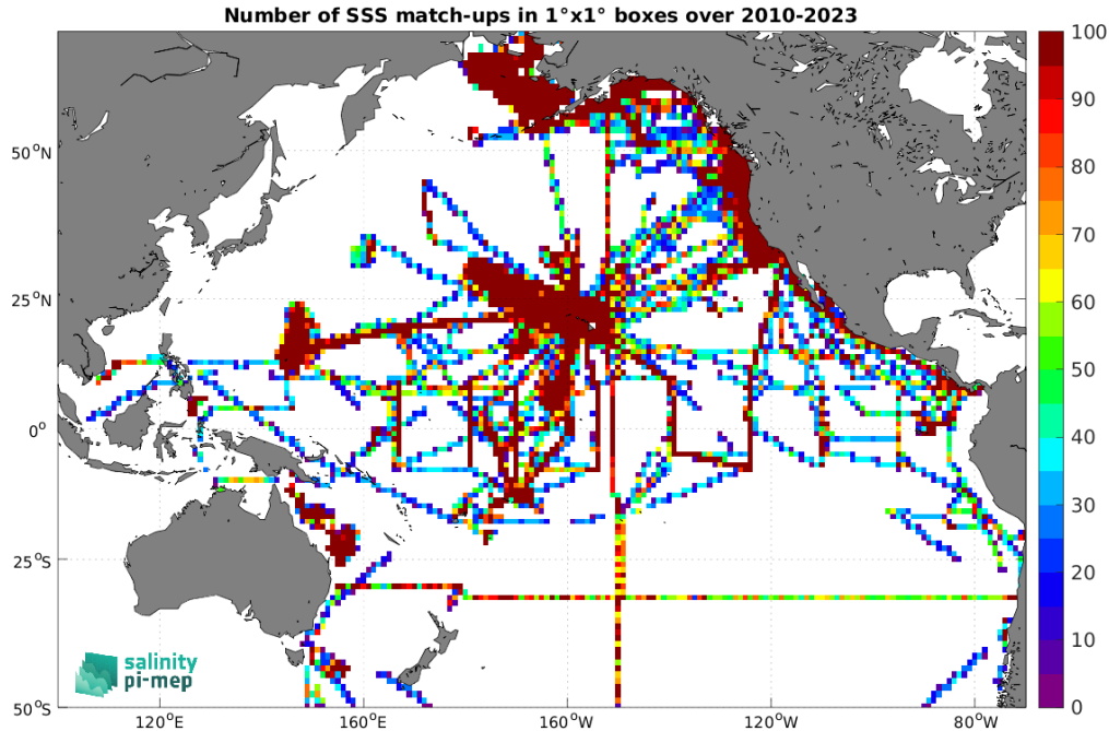
Figure 5: Number of SSS match-ups between TSG (SAMOS) SSS and the SMOS SSS L3 v9 - 18 Days (CATDS-CEC-LOCEAN) SSS product for the Pacific Ocean Pi-MEP region over 1^\circ \times 1^\circ boxes and for the full satellite product period.
