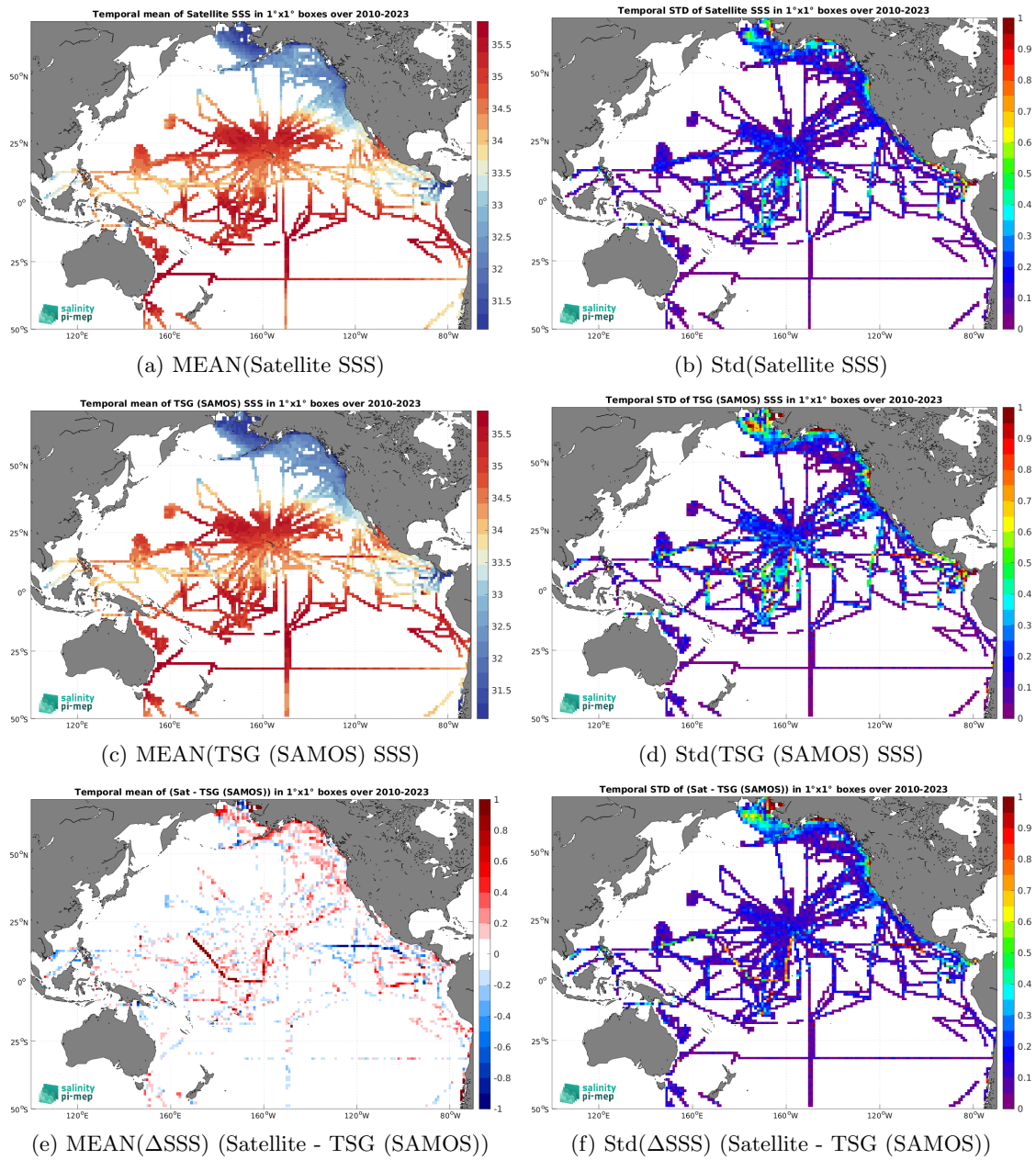
Figure 7: Temporal mean (left) and Std (right) of SSS from SMOS SSS L3 v9 - 18 Days (CATDS-CEC-LOCEAN) (top), TSG (SAMOS) (middle), and of \Delta SSS (Satellite - TSG (SAMOS)). Only match-up pairs are used to generate these maps.
