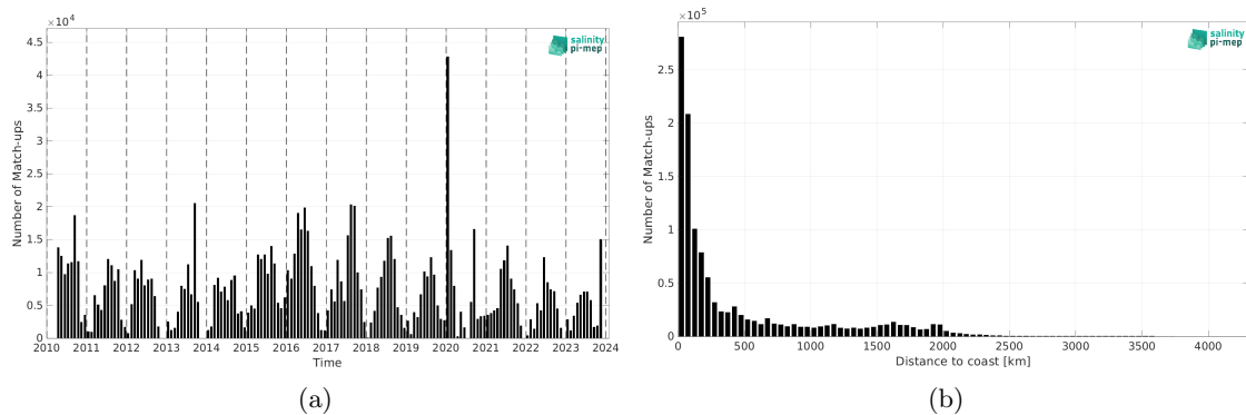
Figure 2: Number of match-ups between TSG (SAMOS) and SMOS SSS L3 v9 - 18 Days (CATDS-CEC-LOCEAN) SSS as a function of time (a) and as function of the distance to coast (b) over the Pacific Ocean Pi-MEP region and for the full satellite product period.
