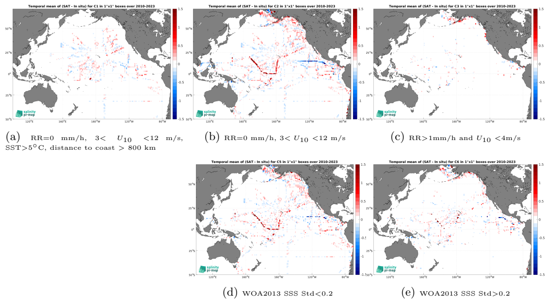
Figure 14: Temporal mean gridded over spatial boxes of size 1^\circ \times 1^\circ of \Delta SSS (SMOS SSS L3 v9 - 18 Days (CATDS-CEC-LOCEAN) - TSG (SAMOS)) for 5 different subdatasets corresponding to:RR=0 mm/h, 3 < U_{10} < 12 m/s, SST >5^\circ\text{C} , distance to coast > 800 km (a), RR=0 mm/h, 3 < U_{10} < 12 m/s (b), RR >1 mm/h and U_{10} < 4 m/s (c), WOA2013 SSS Std <0.2 (d), WOA2013 SSS Std >0.2 (e).
