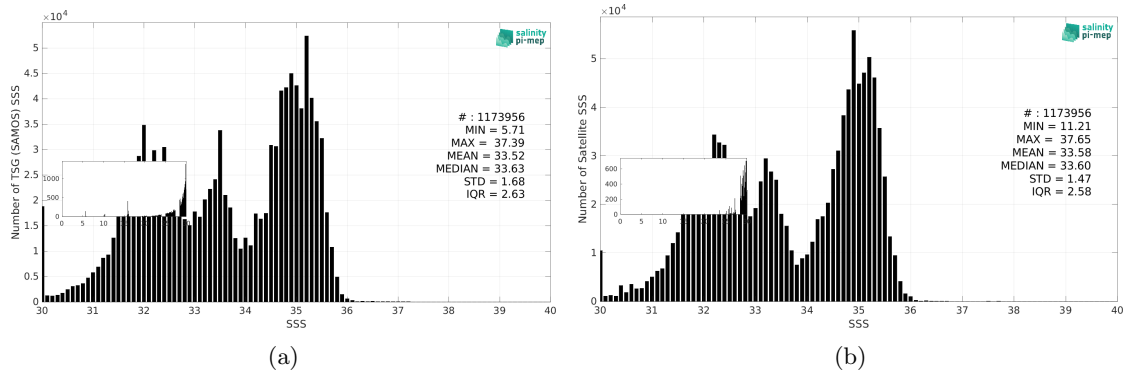
Figure 3: Histograms of SSS from TSG (SAMOS) (a) and SMOS SSS L3 v9 - 18 Days (CATDS-CEC-LOCEAN) (b) considering all match-up pairs per bins of 0.1 over the Pacific Ocean Pi-MEP region and for the full satellite product period.
