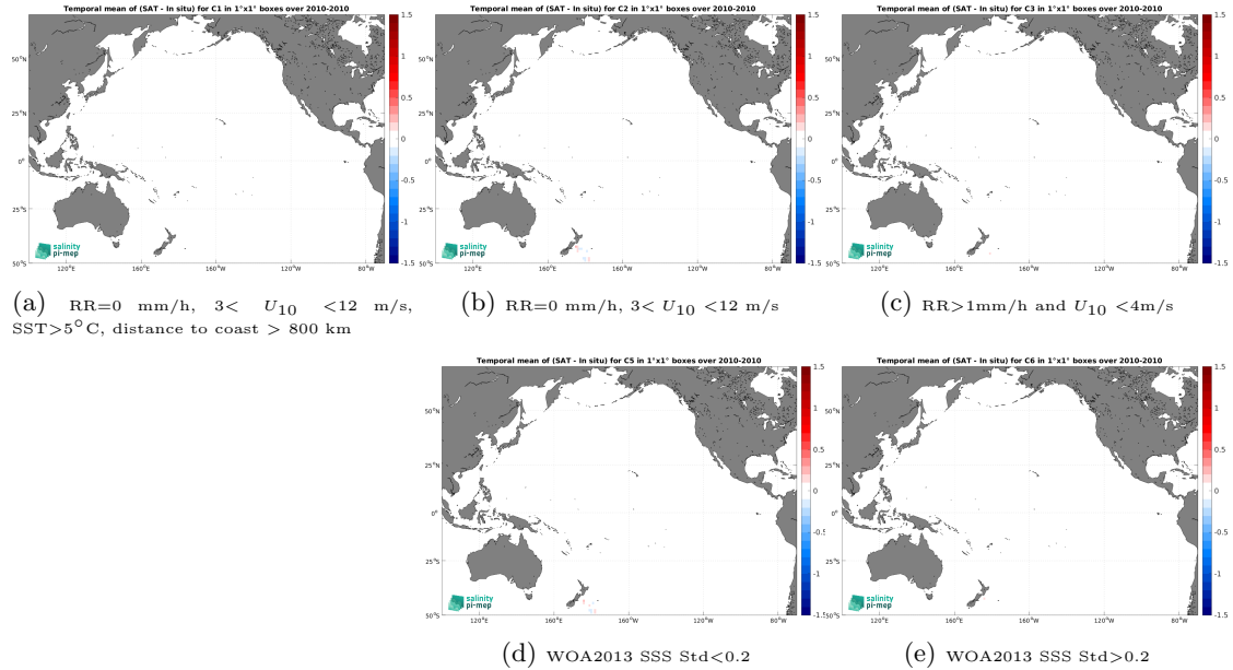
Figure 12: Temporal mean gridded over spatial boxes of size 1^{\circ}\times 1^{\circ} of \Delta\text{SSS} (SMOS SSS L3 v9 - 18 Days (CATDS-CEC-LOCEAN) - TSG (Polarstern)) for 5 different subdatasets corresponding to:RR=0 mm/h, 3 < U_{10} < 12 m/s, SST > 5^{\circ}\text{C} , distance to coast > 800 km (a), RR=0 mm/h, 3 < U_{10} < 12 m/s (b), RR > 1 mm/h and U_{10} < 4 m/s (c), WOA2013 SSS Std < 0.2 (d), WOA2013 SSS Std > 0.2 (e).
