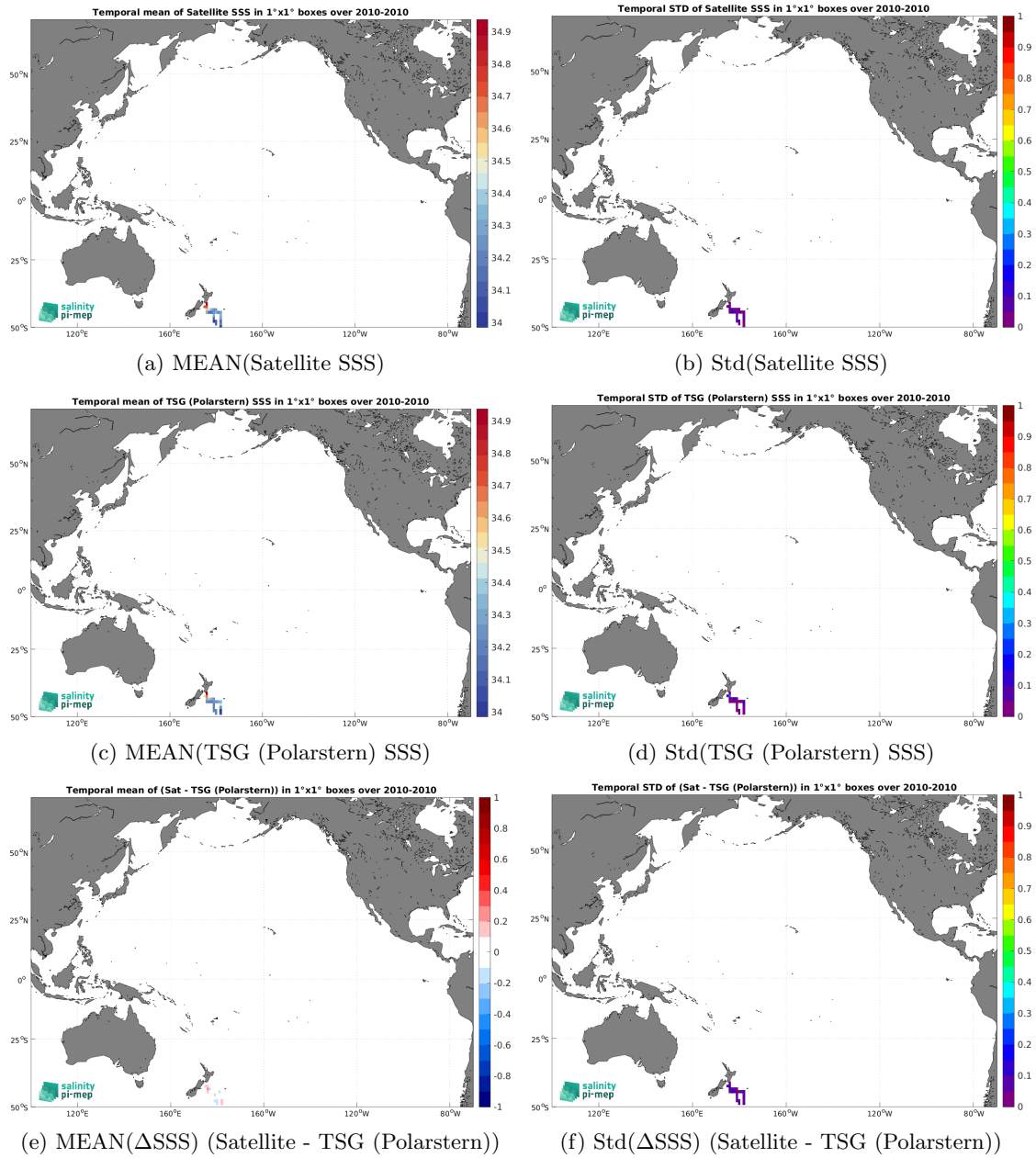
Figure 6: Temporal mean (left) and Std (right) of SSS from SMOS SSS L3 v9 - 18 Days (CATDS-CEC-LOCEAN) (top), TSG (Polarstern) (middle), and of \Delta SSS (Satellite - TSG (Polarstern)). Only match-up pairs are used to generate these maps.
