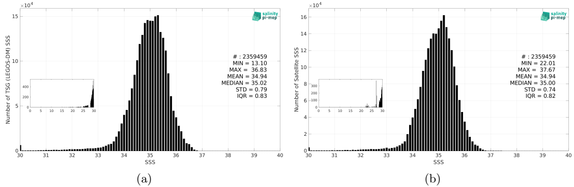
Figure 2: Histograms of SSS from TSG (LEGOS-DM) (a) and SMOS SSS L3 v9 - 18 Days (CATDS-CEC-LOCEAN) (b) considering all match-up pairs per bins of 0.1 over the Pacific Ocean Pi-MEP region and for the full satellite product period.
