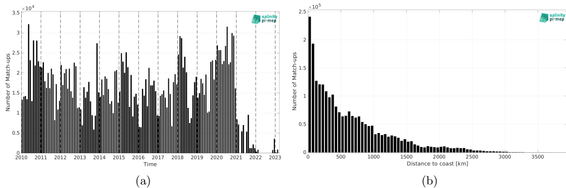
Figure 1: Number of match-ups between TSG (LEGOS-DM) and SMOS SSS L3 v9 - 18 Days (CATDS-CEC-LOCEAN) SSS as a function of time (a) and as function of the distance to coast (b) over the Pacific Ocean Pi-MEP region and for the full satellite product period.
