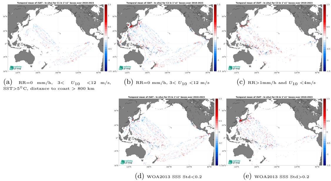
Figure 12: Temporal mean gridded over spatial boxes of size 1^\circ \times 1^\circ of \Delta SSS (SMOS SSS L3 v9 - 18 Days (CATDS-CEC-LOCEAN) - TSG (LEGOS-DM)) for 5 different subdatasets corresponding to:RR=0 mm/h, 3 < U_{10} < 12 m/s, SST >5^\circ C, distance to coast > 800 km (a), RR=0 mm/h, 3 < U_{10} < 12 m/s (b), RR >1 mm/h and U_{10} < 4 m/s (c), WOA2013 SSS Std <0.2 (d), WOA2013 SSS Std >0.2 (e).
