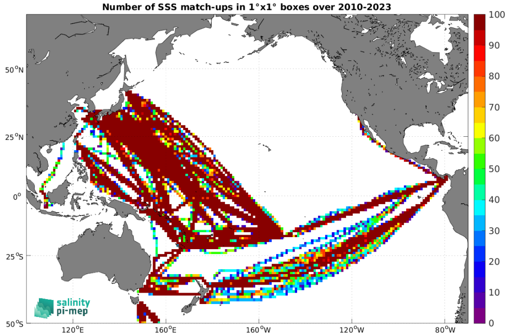
Figure 4: Number of SSS match-ups between TSG (LEGOS-DM) SSS and the SMOS SSS L3 v9 - 18 Days (CATDS-CEC-LOCEAN) SSS product for the Pacific Ocean Pi-MEP region over 1^\circ \times 1^\circ boxes and for the full satellite product period.
