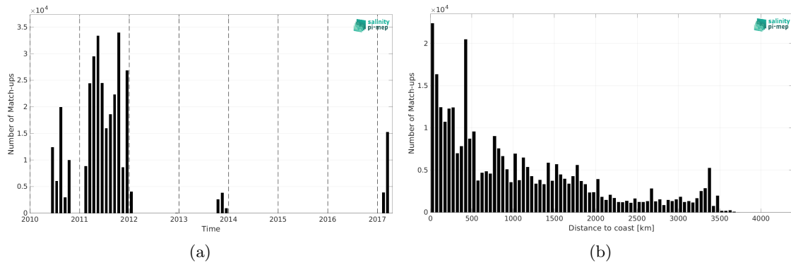
Figure 2: Number of match-ups between TSG (GOSUD-Sailing-ship) and SMOS SSS L3 v9 - 18 Days (CATDS-CEC-LOCEAN) SSS as a function of time (a) and as function of the distance to coast (b) over the Pacific Ocean Pi-MEP region and for the full satellite product period.
