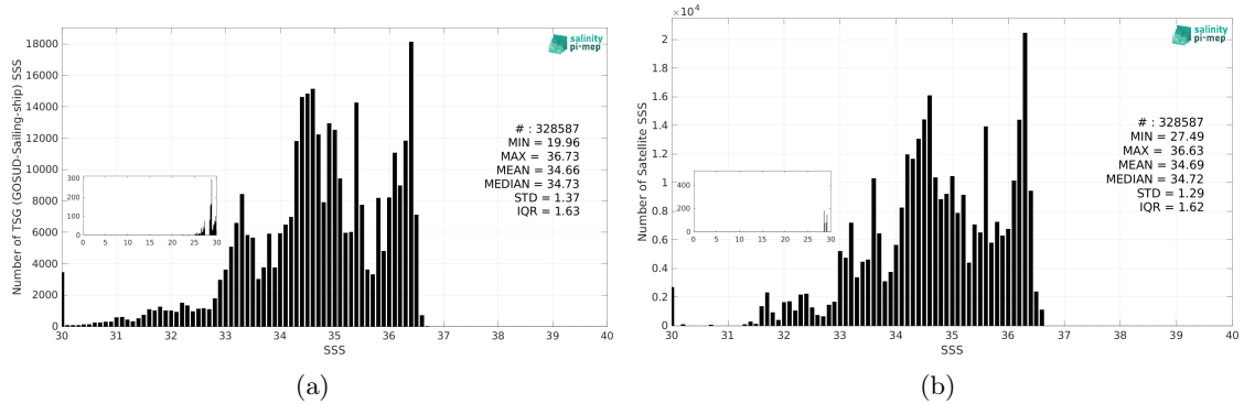
Figure 2: Histograms of SSS from TSG (GOSUD-Sailing-ship) (a) and SMOS SSS L3 v9 - 18 Days (CATDS-CEC-LOCEAN) (b) considering all match-up pairs per bins of 0.1 over the Pacific Ocean Pi-MEP region and for the full satellite product period.
