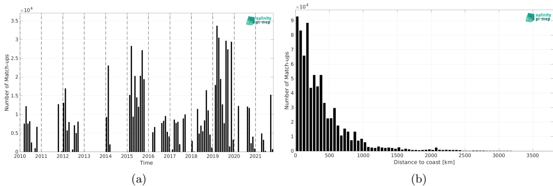
Figure 2: Number of match-ups between TSG (GOSUD-Research-vessel) and SMOS SSS L3 v9 - 18 Days (CATDS-CEC-LOCEAN) SSS as a function of time (a) and as function of the distance to coast (b) over the Pacific Ocean Pi-MEP region and for the full satellite product period.
