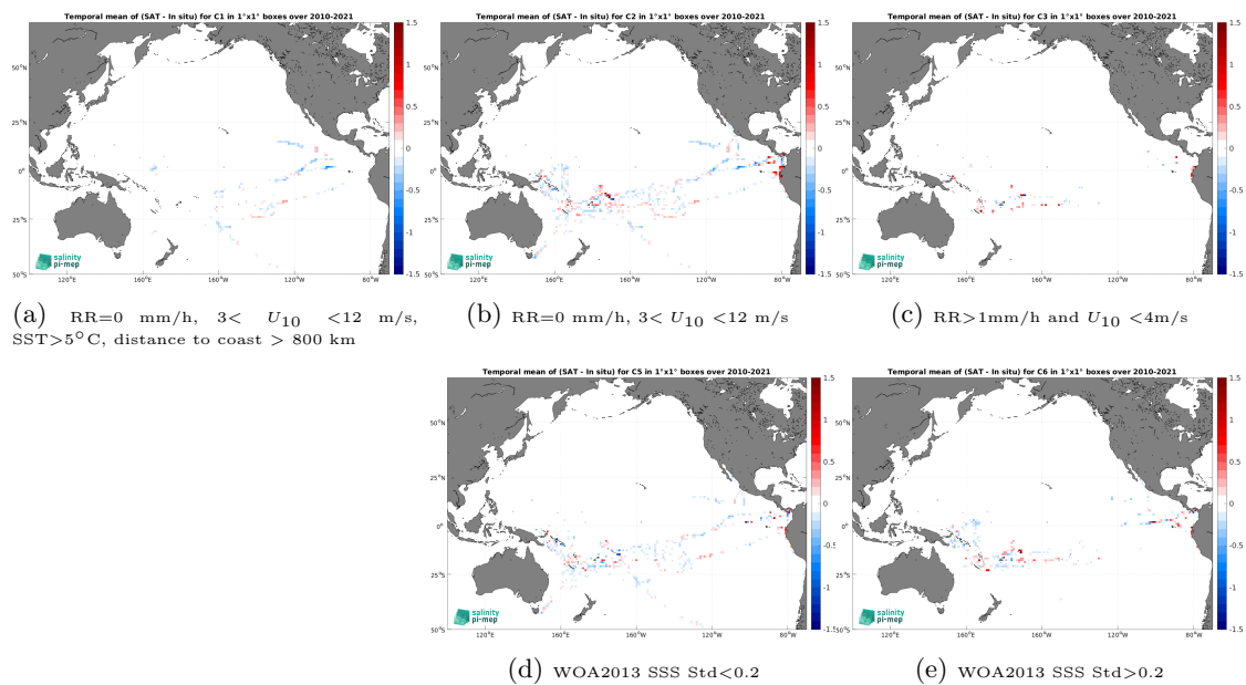
Figure 14: Temporal mean gridded over spatial boxes of size 1^\circ \times 1^\circ of \Delta SSS (SMOS SSS L3 v9 - 18 Days (CATDS-CEC-LOCEAN) - TSG (GOSUD-Research-vessel)) for 5 different subdatasets corresponding to: RR=0 mm/h, 3 < U_{10} < 12 m/s, SST > 5^\circ\text{C} , distance to coast > 800 km (a), RR=0 mm/h, 3 < U_{10} < 12 m/s (b), RR > 1 mm/h and U_{10} < 4 m/s (c), WOA2013 SSS Std < 0.2 (d), WOA2013 SSS Std > 0.2 (e).
