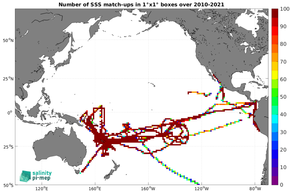
Figure 5: Number of SSS match-ups between TSG (GOSUD-Research-vessel) SSS and the SMOS SSS L3 v9 - 18 Days (CATDS-CEC-LOCEAN) SSS product for the Pacific Ocean Pi-MEP region over 1^\circ \times 1^\circ boxes and for the full satellite product period.
