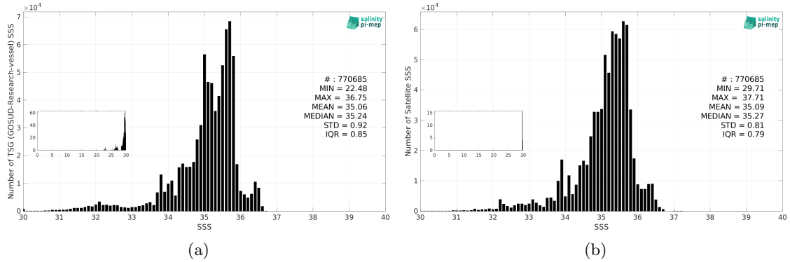
Figure 3: Histograms of SSS from TSG (GOSUD-Research-vessel) (a) and SMOS SSS L3 v9 - 18 Days (CATDS-CEC-LOCEAN) (b) considering all match-up pairs per bins of 0.1 over the Pacific Ocean Pi-MEP region and for the full satellite product period.
