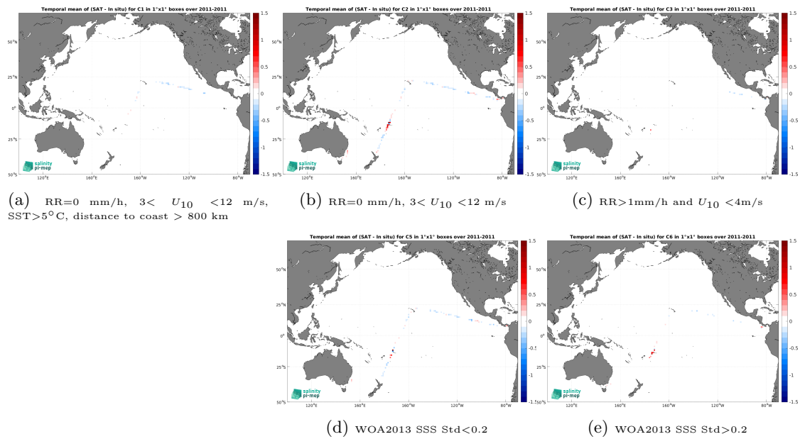
Figure 14: Temporal mean gridded over spatial boxes of size 1^\circ \times 1^\circ of \Delta SSS (SMOS SSS L3 v9 - 18 Days (CATDS-CEC-LOCEAN) - TSG (CSIC-UTM)) for 5 different subdatasets corresponding to:RR=0 mm/h, 3 < U_{10} < 12 m/s, SST >5^\circ\text{C} , distance to coast > 800 km (a), RR=0 mm/h, 3 < U_{10} < 12 m/s (b), RR >1 mm/h and U_{10} < 4 m/s (c), WOA2013 SSS Std <0.2 (d), WOA2013 SSS Std >0.2 (e).
