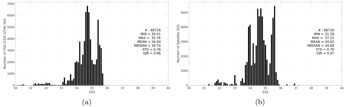
Figure 3: Histograms of SSS from TSG (CSIC-UTM) (a) and SMOS SSS L3 v9 - 18 Days (CATDS-CEC-LOCEAN) (b) considering all match-up pairs per bins of 0.1 over the Pacific Ocean Pi-MEP region and for the full satellite product period.
