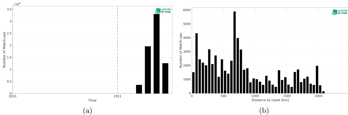
Figure 2: Number of match-ups between TSG (CSIC-UTM) and SMOS SSS L3 v9 - 18 Days (CATDS-CEC-LOCEAN) SSS as a function of time (a) and as function of the distance to coast (b) over the Pacific Ocean Pi-MEP region and for the full satellite product period.
