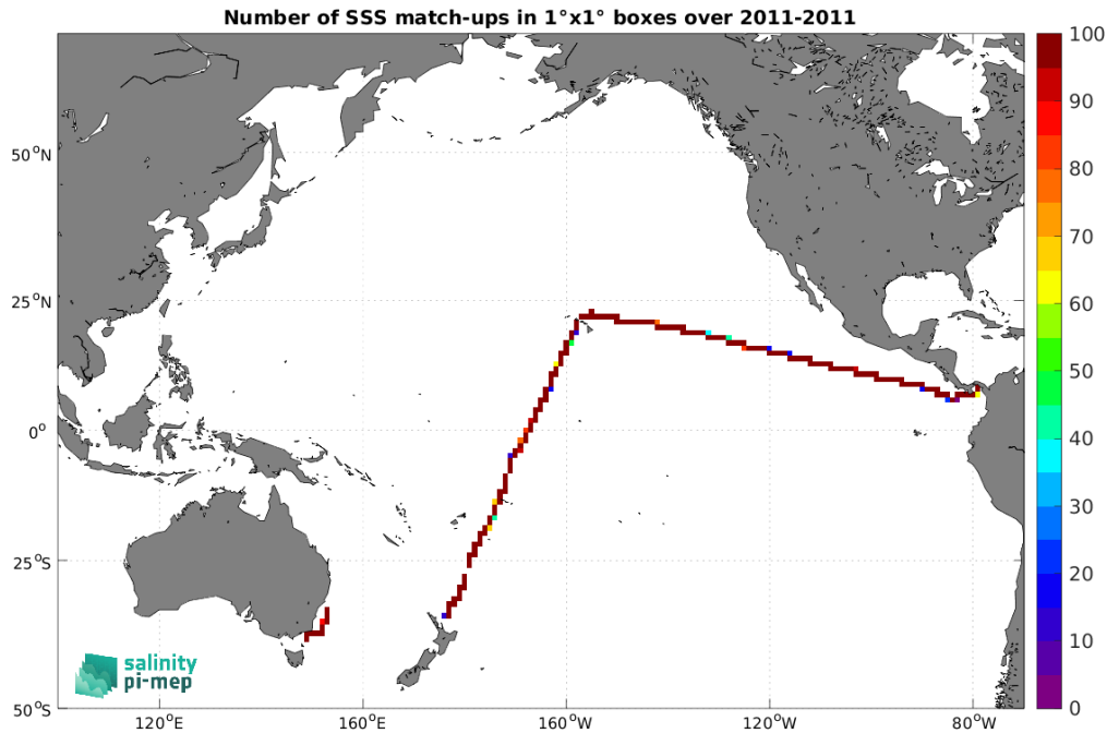
Figure 5: Number of SSS match-ups between TSG (CSIC-UTM) SSS and the SMOS SSS L3 v9 - 18 Days (CATDS-CEC-LOCEAN) SSS product for the Pacific Ocean Pi-MEP region over 1^\circ \times 1^\circ boxes and for the full satellite product period.
