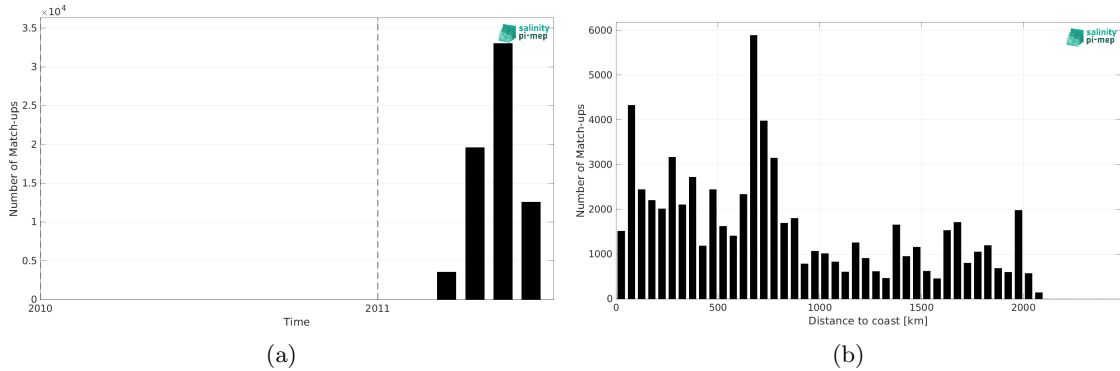
Figure 1: Number of match-ups between TSG (CSIC-UTM) and SMOS SSS L3 v9 - 18 Days (CATDS-CEC-LOCEAN) SSS as a function of time (a) and as function of the distance to coast (b) over the Pacific Ocean Pi-MEP region and for the full satellite product period.
