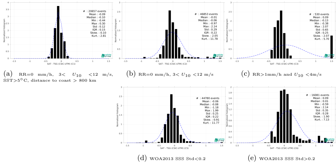
Figure 13: Normalized histogram of \Delta\text{SSS} (SMOS SSS L3 v9 - 18 Days (CATDS-CEC-LOCEAN) - TSG (CSIC-UTM)) for 5 different subdatasets corresponding to: RR=0 mm/h, 3 < U_{10} < 12 m/s, SST>5°C, distance to coast > 800 km (a), RR=0 mm/h, 3 < U_{10} < 12 m/s (b), RR>1mm/h and U_{10} < 4 m/s (c), WOA2013 SSS Std<0.2 (d), WOA2013 SSS Std>0.2 (e).
