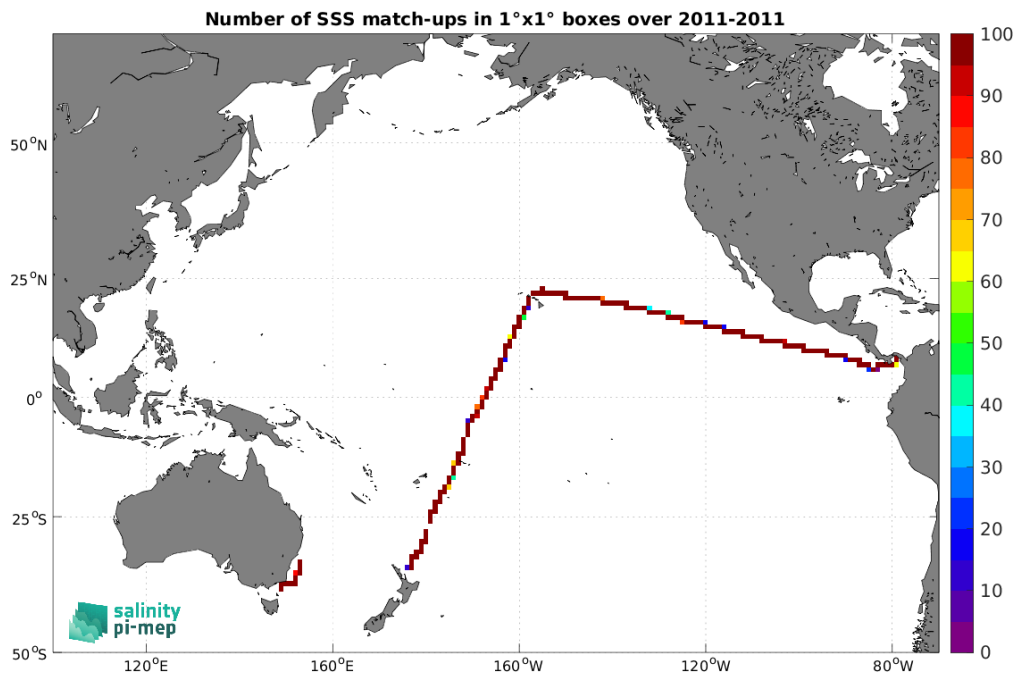
Figure 4: Number of SSS match-ups between TSG (CSIC-UTM) SSS and the SMOS SSS L3 v9 - 18 Days (CATDS-CEC-LOCEAN) SSS product for the Pacific Ocean Pi-MEP region over 1^\circ \times 1^\circ boxes and for the full satellite product period.
