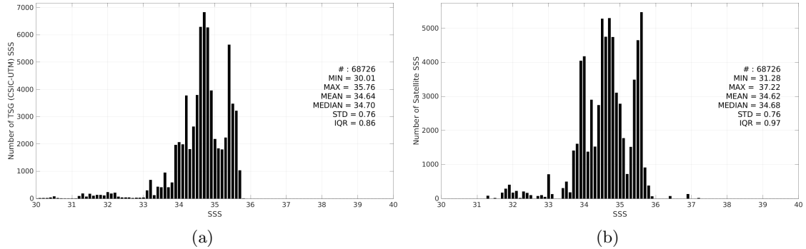
Figure 2: Histograms of SSS from TSG (CSIC-UTM) (a) and SMOS SSS L3 v9 - 18 Days (CATDS-CEC-LOCEAN) (b) considering all match-up pairs per bins of 0.1 over the Pacific Ocean Pi-MEP region and for the full satellite product period.
