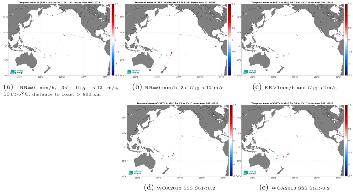
Figure 12: Temporal mean gridded over spatial boxes of size 1^{\circ}\times 1^{\circ} of \Delta\text{SSS} (SMOS SSS L3 v9 - 18 Days (CATDS-CEC-LOCEAN) - TSG (CSIC-UTM)) for 5 different subdatasets corresponding to: RR=0 mm/h, 3 < U_{10} < 12 m/s, SST > 5^{\circ}\text{C} , distance to coast > 800 km (a), RR=0 mm/h, 3 < U_{10} < 12 m/s (b), RR > 1 mm/h and U_{10} < 4 m/s (c), WOA2013 SSS Std < 0.2 (d), WOA2013 SSS Std > 0.2 (e).
