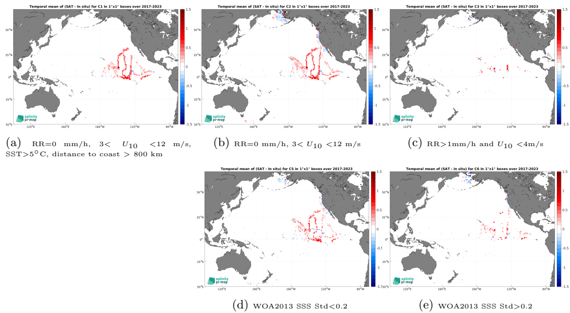
Figure 14: Temporal mean gridded over spatial boxes of size 1^\circ \times 1^\circ of \Delta SSS (SMOS SSS L3 v9 - 18 Days (CATDS-CEC-LOCEAN) - Saildrone) for 5 different subdatasets corresponding to: RR=0 mm/h, 3 < U_{10} < 12 m/s, SST > 5^\circ\text{C} , distance to coast > 800 km (a), RR=0 mm/h, 3 < U_{10} < 12 m/s (b), RR > 1 mm/h and U_{10} < 4 m/s (c), WOA2013 SSS Std < 0.2 (d), WOA2013 SSS Std > 0.2 (e).
