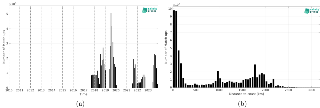
Figure 2: Number of match-ups between Saildrone and SMOS SSS L3 v9 - 18 Days (CATDS-CEC-LOCEAN) SSS as a function of time (a) and as function of the distance to coast (b) over the Pacific Ocean Pi-MEP region and for the full satellite product period.
