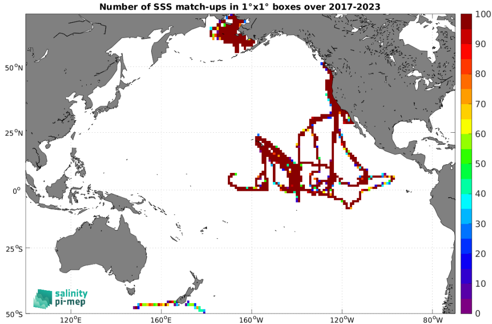
Figure 5: Number of SSS match-ups between Saildrone SSS and the SMOS SSS L3 v9 - 18 Days (CATDS-CEC-LOCEAN) SSS product for the Pacific Ocean Pi-MEP region over 1^\circ \times 1^\circ boxes and for the full satellite product period.
