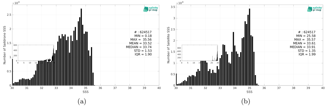
Figure 3: Histograms of SSS from Saildrone (a) and SMOS SSS L3 v9 - 18 Days (CATDS-CEC-LOCEAN) (b) considering all match-up pairs per bins of 0.1 over the Pacific Ocean Pi-MEP region and for the full satellite product period.
