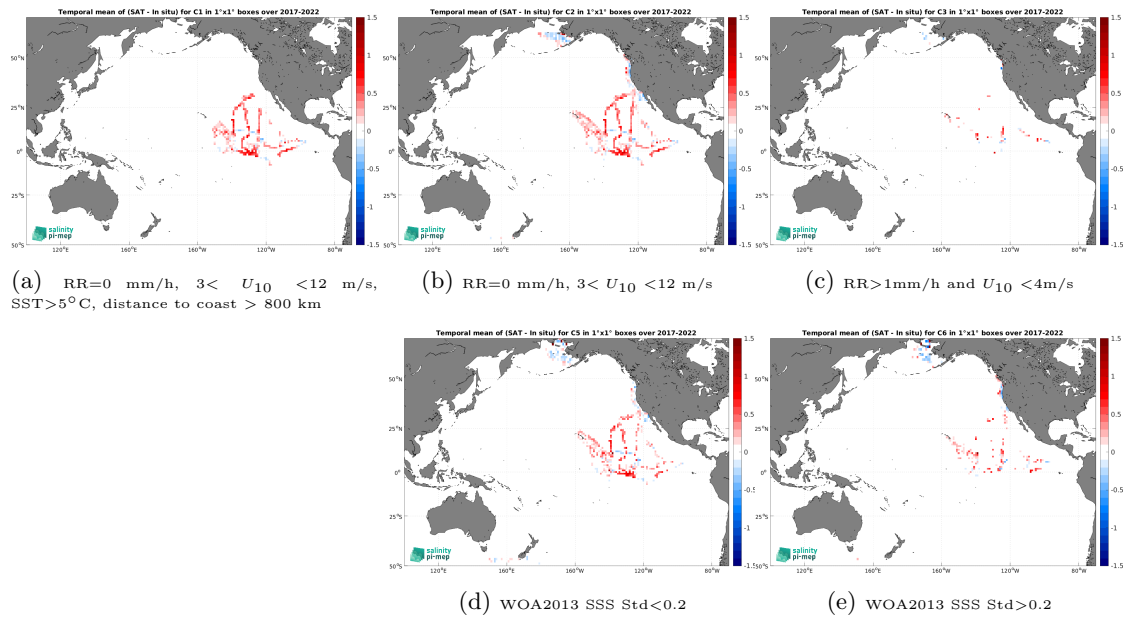
Figure 12: Temporal mean gridded over spatial boxes of size 1^\circ \times 1^\circ of \Delta SSS (SMOS SSS L3 v9 - 18 Days (CATDS-CEC-LOCEAN) - Saildrone) for 5 different subdatasets corresponding to:RR=0 mm/h, 3 < U_{10} < 12 m/s, SST >5^\circ C, distance to coast > 800 km (a), RR=0 mm/h, 3 < U_{10} < 12 m/s (b), RR >1 mm/h and U_{10} < 4 m/s (c), WOA2013 SSS Std <0.2 (d), WOA2013 SSS Std >0.2 (e).
