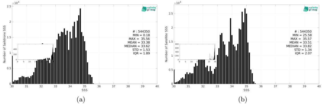
Figure 2: Histograms of SSS from Saildrone (a) and SMOS SSS L3 v9 - 18 Days (CATDS-CEC-LOCEAN) (b) considering all match-up pairs per bins of 0.1 over the Pacific Ocean Pi-MEP region and for the full satellite product period.
