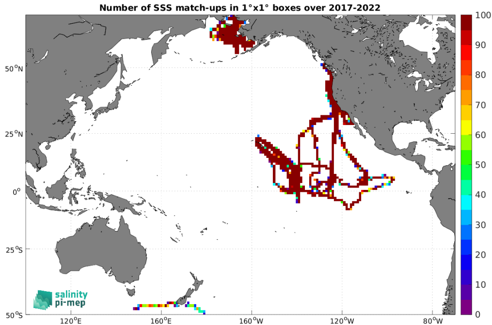
Figure 4: Number of SSS match-ups between Saildrone SSS and the SMOS SSS L3 v9 - 18 Days (CATDS-CEC-LOCEAN) SSS product for the Pacific Ocean Pi-MEP region over 1^\circ \times 1^\circ boxes and for the full satellite product period.
