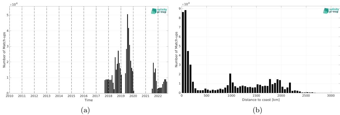
Figure 1: Number of match-ups between Saildrone and SMOS SSS L3 v9 - 18 Days (CATDS-CEC-LOCEAN) SSS as a function of time (a) and as function of the distance to coast (b) over the Pacific Ocean Pi-MEP region and for the full satellite product period.
