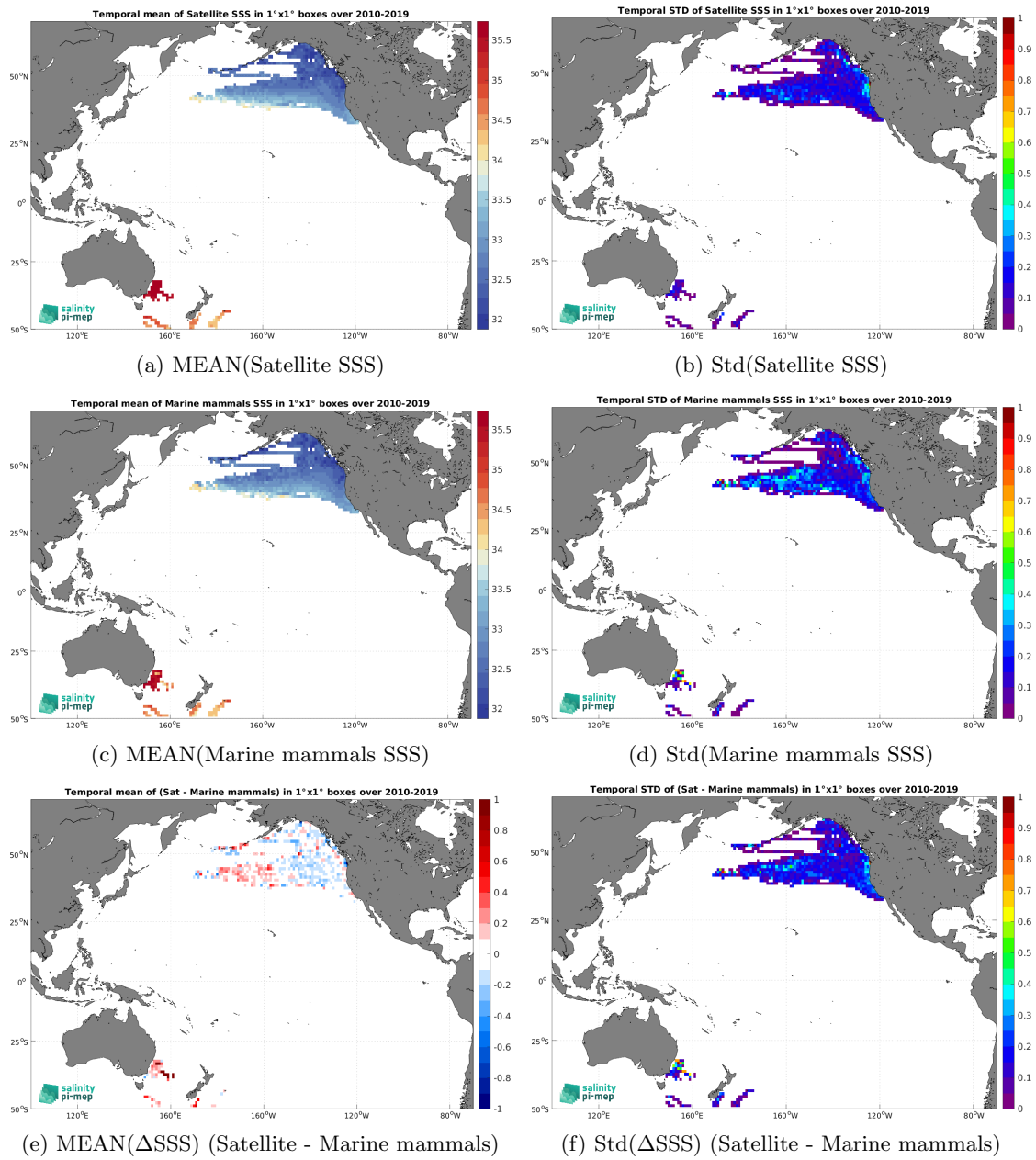
Figure 6: Temporal mean (left) and Std (right) of SSS from SMOS SSS L3 v9 - 18 Days (CATDS-CEC-LOCEAN) (top), Marine mammals (middle), and of \Delta SSS (Satellite - Marine mammals). Only match-up pairs are used to generate these maps.
