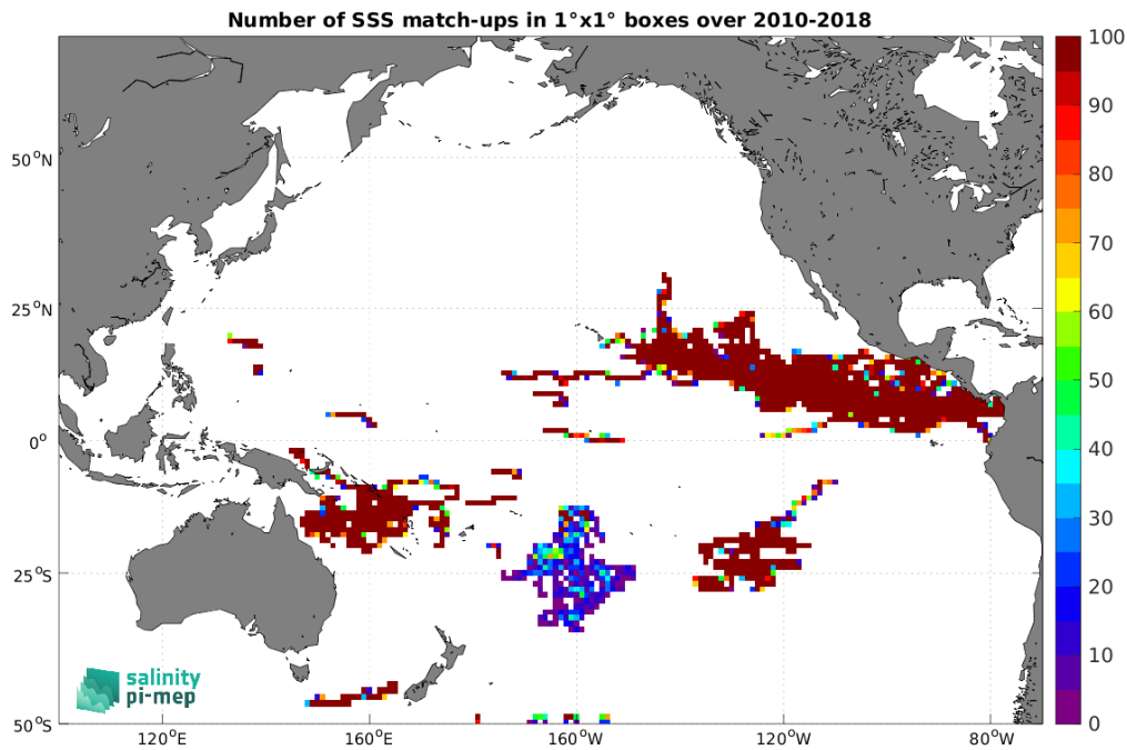
Figure 4: Number of SSS match-ups between Surface drifters SSS and the SMOS SSS L3 v9 - 18 Days (CATDS-CEC-LOCEAN) SSS product for the Pacific Ocean Pi-MEP region over 1^\circ \times 1^\circ boxes and for the full satellite product period.
