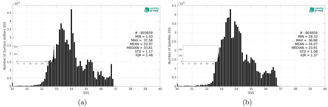
Figure 3: Histograms of SSS from Surface drifters (a) and SMOS SSS L3 v9 - 18 Days (CATDS-CEC-LOCEAN) (b) considering all match-up pairs per bins of 0.1 over the Pacific Ocean Pi-MEP region and for the full satellite product period.
