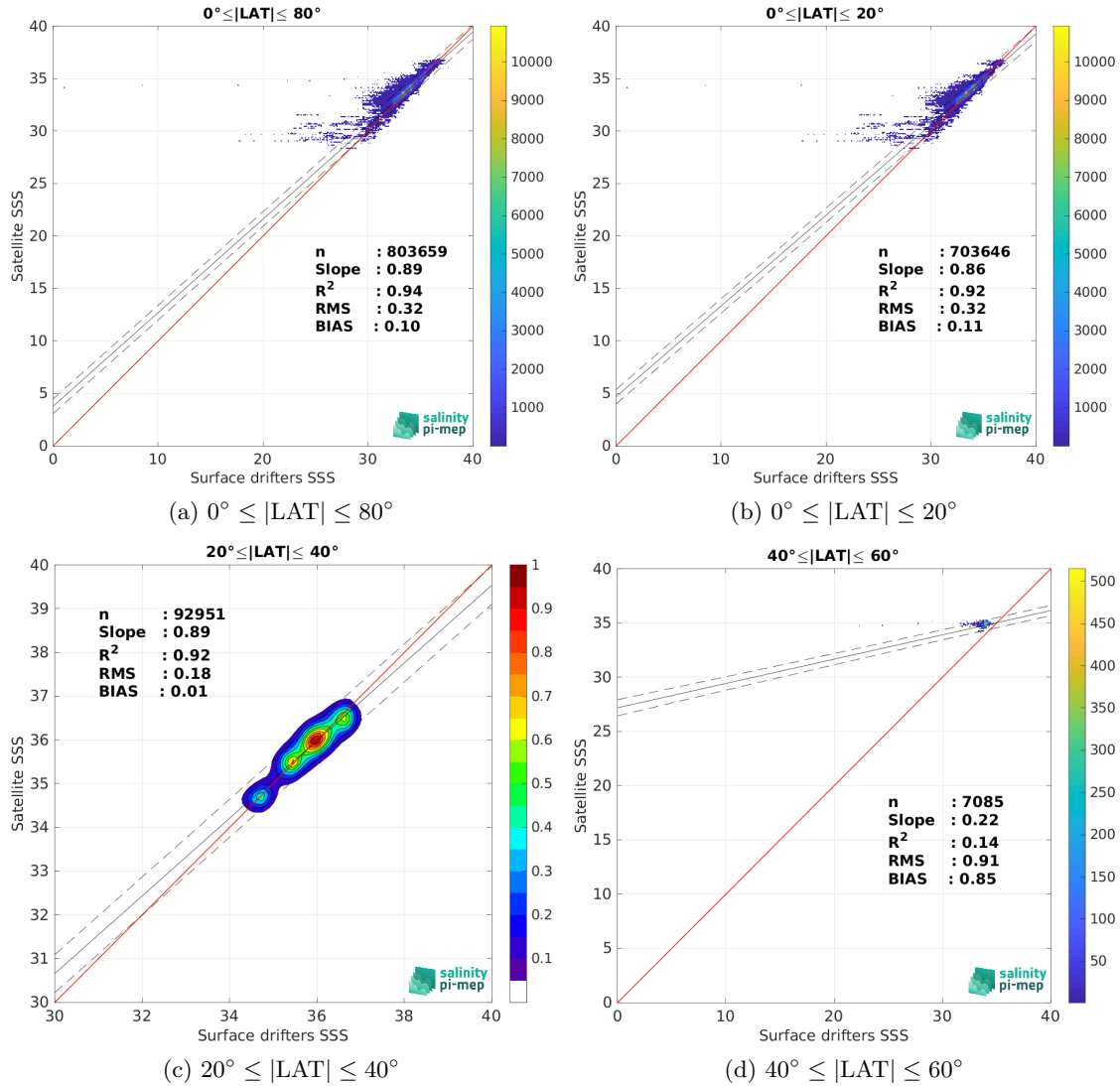
Figure 9: Contour maps of the concentration of SMOS SSS L3 v9 - 18 Days (CATDS-CEC-LOCEAN) SSS (y-axis) versus Surface drifters SSS (x-axis) at match-up pairs for different latitude bands. For each plot, the red line shows x=y . The black thin and dashed lines indicate a linear fit through the data cloud and the \pm 95\% confidence levels, respectively. The number match-up pairs n , the slope and R^2 coefficient of the linear fit, the root mean square (RMS) and the mean bias between satellite and in situ data are indicated for each latitude band in each plots.
