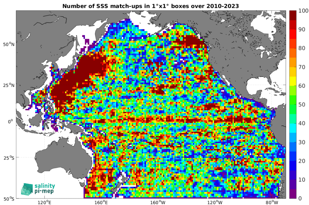
Figure 4: Number of SSS match-ups between Argo SSS and the SMOS SSS L3 v9 - 18 Days (CATDS-CEC-LOCEAN) SSS product for the Pacific Ocean Pi-MEP region over 1^\circ \times 1^\circ boxes and for the full satellite product period.
