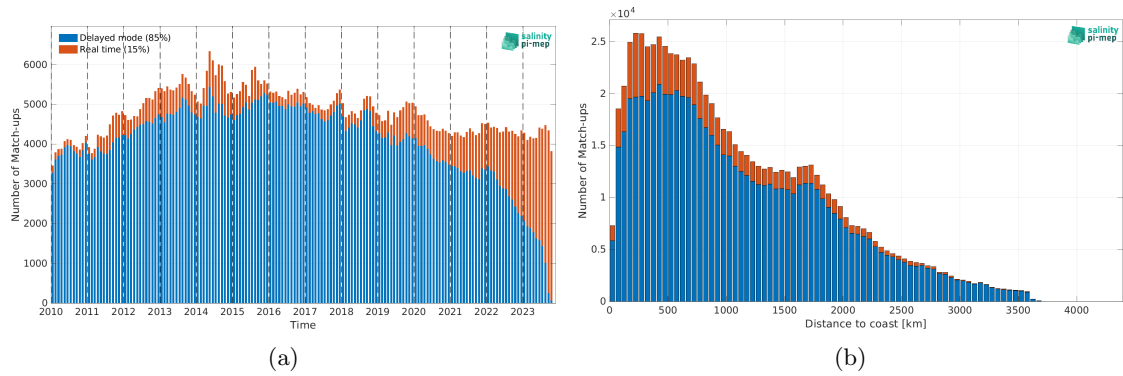
Figure 1: Number of match-ups between Argo and SMOS SSS L3 v9 - 18 Days (CATDS-CEC-LOCEAN) SSS as a function of time (a) and as function of the distance to coast (b) over the Pacific Ocean Pi-MEP region and for the full satellite product period.
