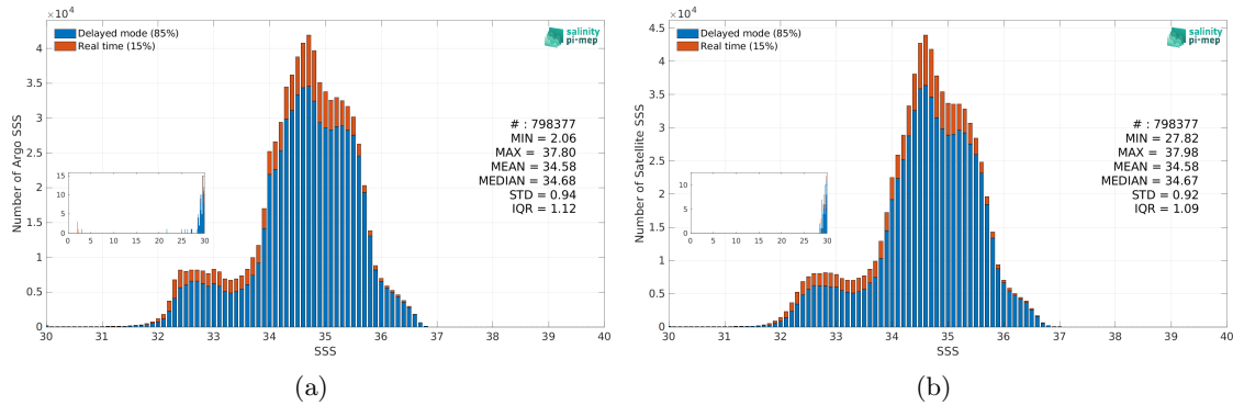
Figure 2: Histograms of SSS from Argo (a) and SMOS SSS L3 v9 - 18 Days (CATDS-CEC-LOCEAN) (b) considering all match-up pairs per bins of 0.1 over the Pacific Ocean Pi-MEP region and for the full satellite product period.
