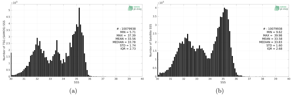
Figure 2: Histograms of SSS from TSG (SAMOS) (a) and SMOS SSS L3 v8 - 9 Days (CATDS-CECOS-LOCEAN) (b) considering all match-up pairs per bins of 0.1 over the Pacific Ocean Pi-MEP region and for the full satellite product period.
