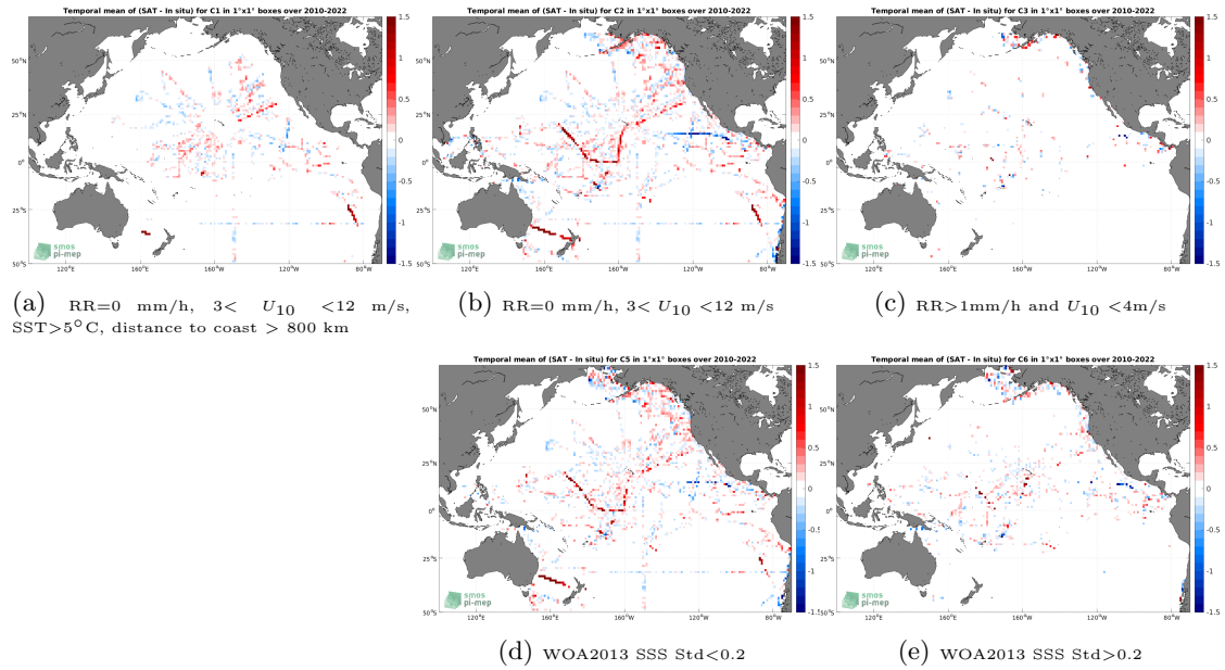
Figure 12: Temporal mean gridded over spatial boxes of size 1^\circ \times 1^\circ of \Delta SSS (SMOS SSS L3 v8 - 9 Days (CATDS-CECOS-LOCEAN) - TSG (SAMOS)) for 5 different subdatasets corresponding to:RR=0 mm/h, 3 < U_{10} < 12 m/s, SST >5^\circ C, distance to coast > 800 km (a), RR=0 mm/h, 3 < U_{10} < 12 m/s (b), RR >1 mm/h and U_{10} < 4 m/s (c), WOA2013 SSS Std <0.2 (d), WOA2013 SSS Std >0.2 (e).
