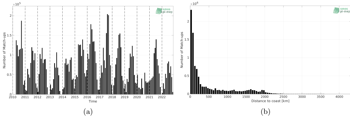
Figure 1: Number of match-ups between TSG (SAMOS) and SMOS SSS L3 v8 - 9 Days (CATDS-CECOS-LOCEAN) SSS as a function of time (a) and as function of the distance to coast (b) over the Pacific Ocean Pi-MEP region and for the full satellite product period.
