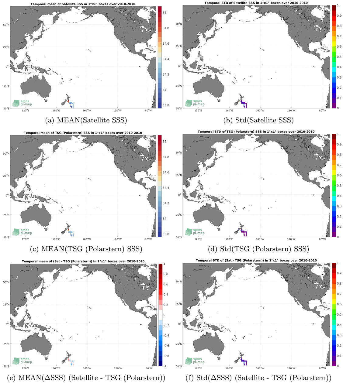
Figure 6: Temporal mean (left) and Std (right) of SSS from SMOS SSS L3 v8 - 9 Days (CATDS-CECOS-LOCEAN) (top), TSG (Polarstern) (middle), and of \Delta SSS (Satellite - TSG (Polarstern)). Only match-up pairs are used to generate these maps.
