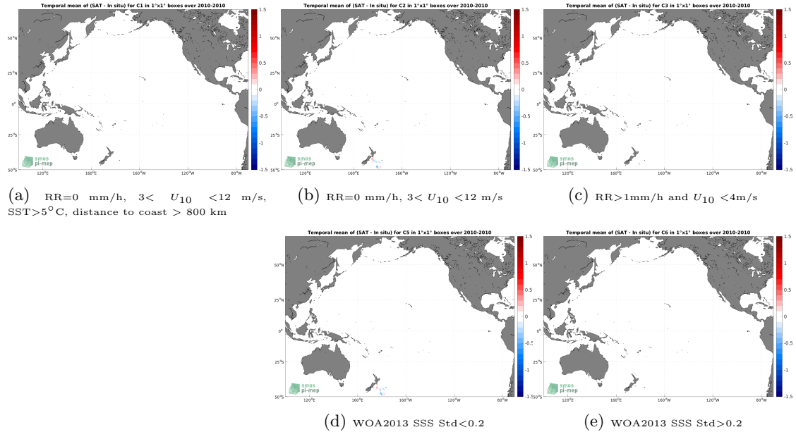
Figure 12: Temporal mean gridded over spatial boxes of size 1^{\circ}\times 1^{\circ} of \Delta\text{SSS} (SMOS SSS L3 v8 - 9 Days (CATDS-CECOS-LOCEAN) - TSG (Polarstern)) for 5 different subdatasets corresponding to:RR=0 mm/h, 3 < U_{10} < 12 m/s, SST >5^{\circ}\text{C} , distance to coast > 800 km (a), RR=0 mm/h, 3 < U_{10} < 12 m/s (b), RR >1 mm/h and U_{10} < 4 m/s (c), WOA2013 SSS Std <0.2 (d), WOA2013 SSS Std >0.2 (e).
