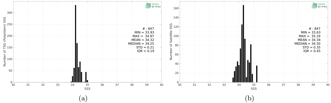
Figure 2: Histograms of SSS from TSG (Polarstern) (a) and SMOS SSS L3 v8 - 9 Days (CATDS-CECOS-LOCEAN) (b) considering all match-up pairs per bins of 0.1 over the Pacific Ocean Pi-MEP region and for the full satellite product period.
