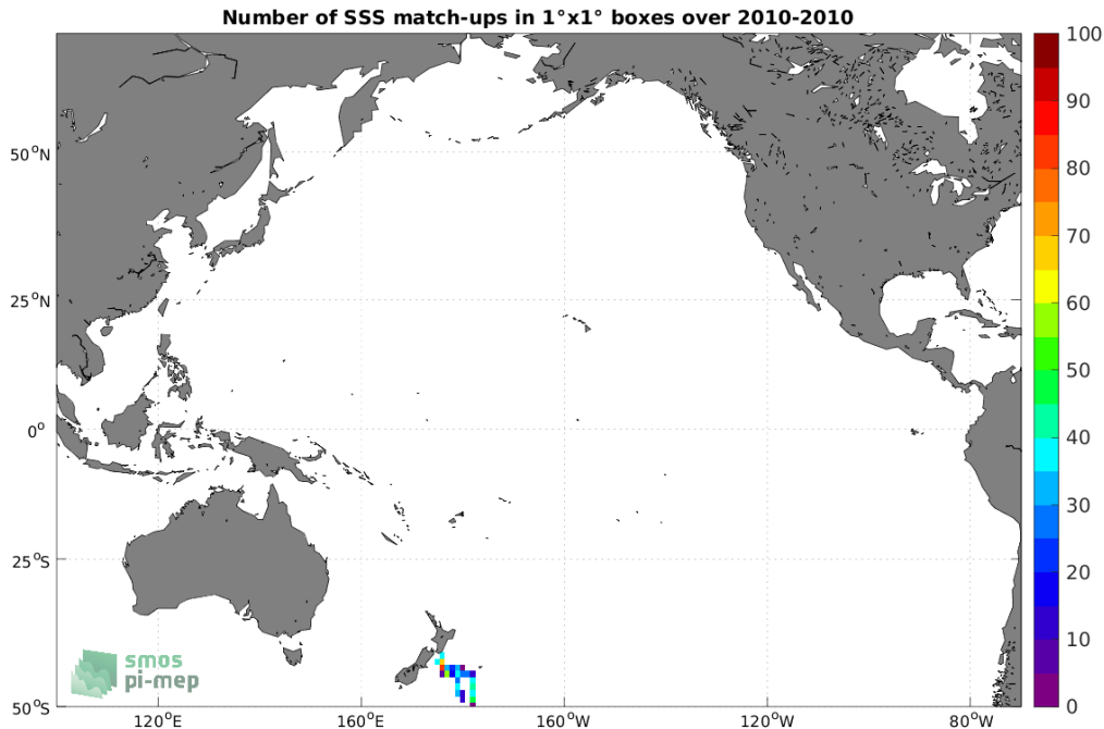
Figure 4: Number of SSS match-ups between TSG (Polarstern) SSS and the SMOS SSS L3 v8 - 9 Days (CATDS-CECOS-LOCEAN) SSS product for the Pacific Ocean Pi-MEP region over 1^\circ \times 1^\circ boxes and for the full satellite product period.
