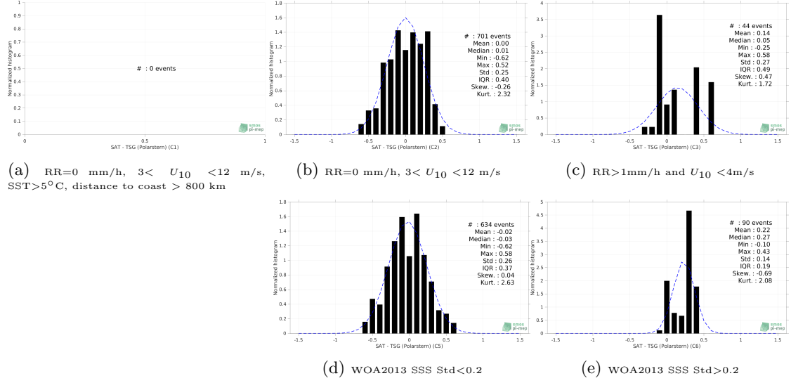
Figure 13: Normalized histogram of \Delta SSS (SMOS SSS L3 v8 - 9 Days (CATDS-CECOS-LOCEAN) - TSG (Polarstern)) for 5 different subdatasets corresponding to: RR=0 mm/h, 3 < U_{10} < 12 m/s, SST > 5°C, distance to coast > 800 km (a), RR=0 mm/h, 3 < U_{10} < 12 m/s (b), RR > 1mm/h and U_{10} < 4 m/s (c), WOA2013 SSS Std < 0.2 (d), WOA2013 SSS Std > 0.2 (e).
