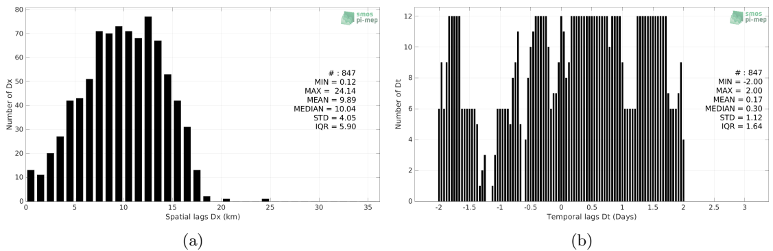
Figure 5: Histograms of the spatial (a) and temporal (b) lags between the location/time of the TSG (Polarstern) measurement and the date of the corresponding SMOS SSS L3 v8 - 9 Days (CATDS-CECOS-LOCEAN) SSS pixel.
