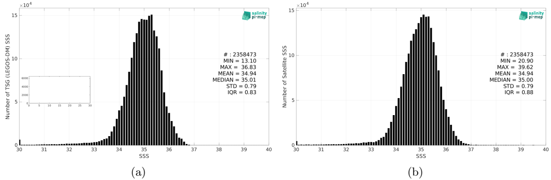
Figure 2: Histograms of SSS from TSG (LEGOS-DM) (a) and SMOS SSS L3 v8 - 9 Days (CATDS-CEC-LOCEAN) (b) considering all match-up pairs per bins of 0.1 over the Pacific Ocean Pi-MEP region and for the full satellite product period.
