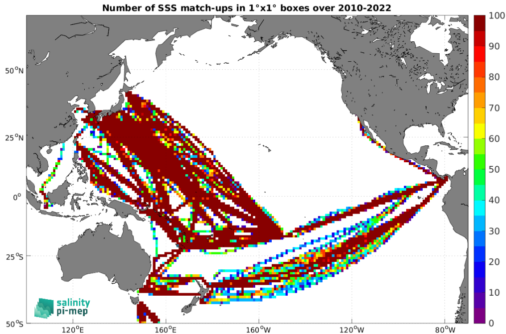
Figure 4: Number of SSS match-ups between TSG (LEGOS-DM) SSS and the SMOS SSS L3 v8 - 9 Days (CATDS-CEC-LOCEAN) SSS product for the Pacific Ocean Pi-MEP region over 1^\circ \times 1^\circ boxes and for the full satellite product period.
