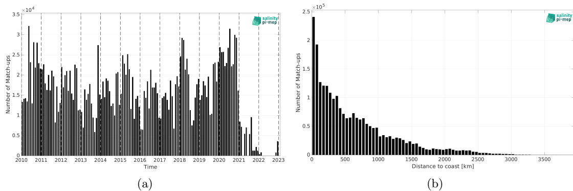
Figure 1: Number of match-ups between TSG (LEGOS-DM) and SMOS SSS L3 v8 - 9 Days (CATDS-CEC-LOCEAN) SSS as a function of time (a) and as function of the distance to coast (b) over the Pacific Ocean Pi-MEP region and for the full satellite product period.
