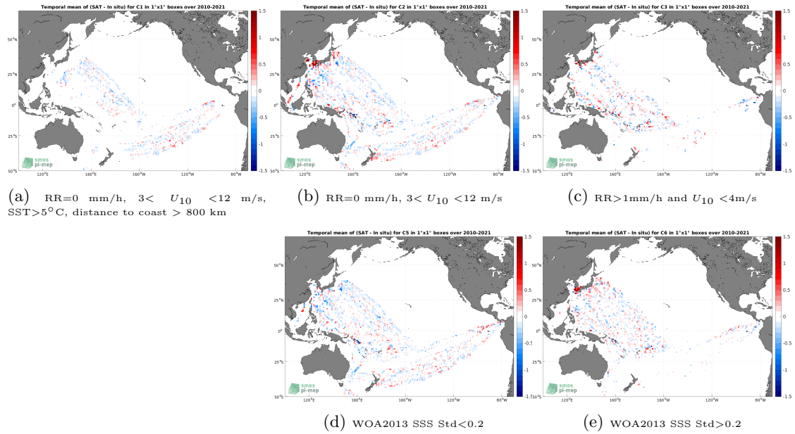
Figure 12: Temporal mean gridded over spatial boxes of size 1^\circ \times 1^\circ of \Delta SSS (SMOS SSS L3 v8 - 9 Days (CATDS-CECOS-LOCEAN) - TSG (LEGOS-DM)) for 5 different subdatasets corresponding to:RR=0 mm/h, 3 < U_{10} < 12 m/s, SST >5^\circ C, distance to coast > 800 km (a), RR=0 mm/h, 3 < U_{10} < 12 m/s (b), RR >1 mm/h and U_{10} < 4 m/s (c), WOA2013 SSS Std <0.2 (d), WOA2013 SSS Std >0.2 (e).
