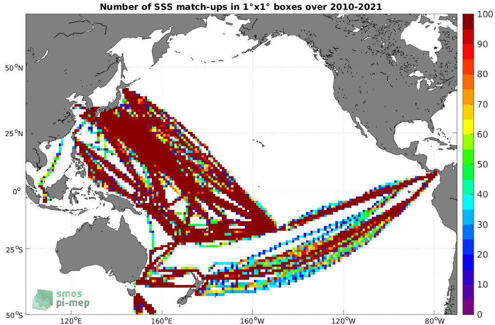
Figure 4: Number of SSS match-ups between TSG (LEGOS-DM) SSS and the SMOS SSS L3 v8 - 9 Days (CATDS-CECOS-LOCEAN) SSS product for the Pacific Ocean Pi-MEP region over 1^\circ \times 1^\circ boxes and for the full satellite product period.
