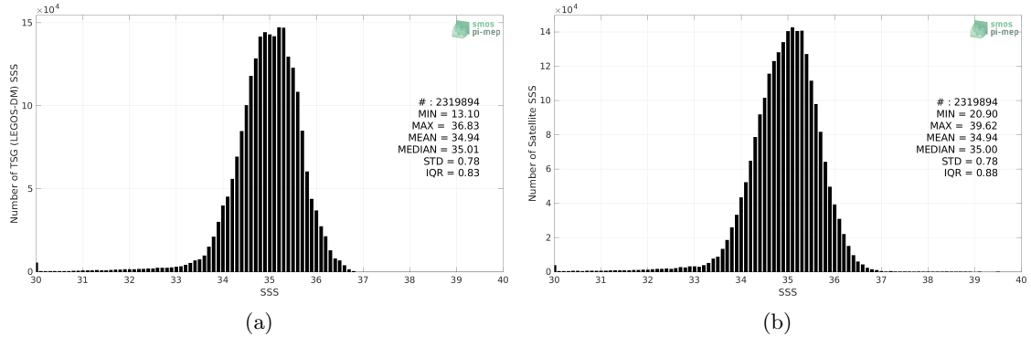
Figure 2: Histograms of SSS from TSG (LEGOS-DM) (a) and SMOS SSS L3 v8 - 9 Days (CATDS-CECOS-LOCEAN) (b) considering all match-up pairs per bins of 0.1 over the Pacific Ocean Pi-MEP region and for the full satellite product period.
