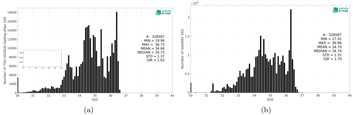
Figure 2: Histograms of SSS from TSG (GOSUD-Sailing-ship) (a) and SMOS SSS L3 v8 - 9 Days (CATDS-CEC-LOCEAN) (b) considering all match-up pairs per bins of 0.1 over the Pacific Ocean Pi-MEP region and for the full satellite product period.
