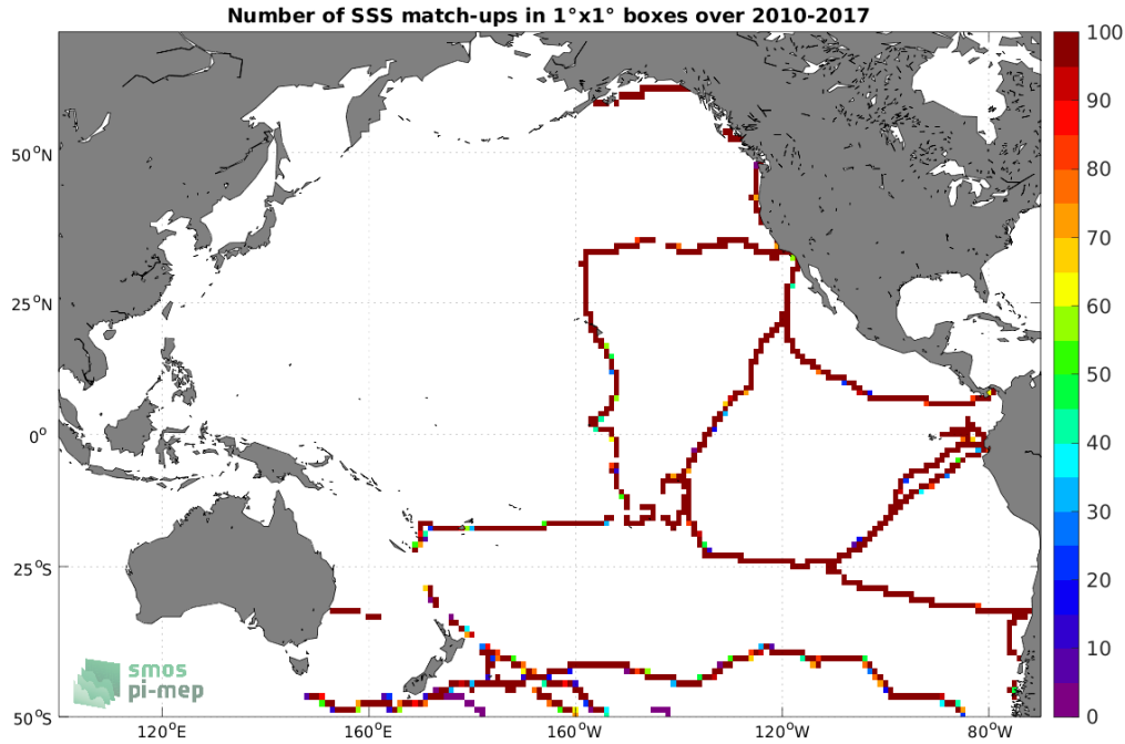
Figure 4: Number of SSS match-ups between TSG (GOSUD-Sailing-ship) SSS and the SMOS SSS L3 v8 - 9 Days (CATDS-CECOS-LOCEAN) SSS product for the Pacific Ocean Pi-MEP region over 1^\circ \times 1^\circ boxes and for the full satellite product period.
