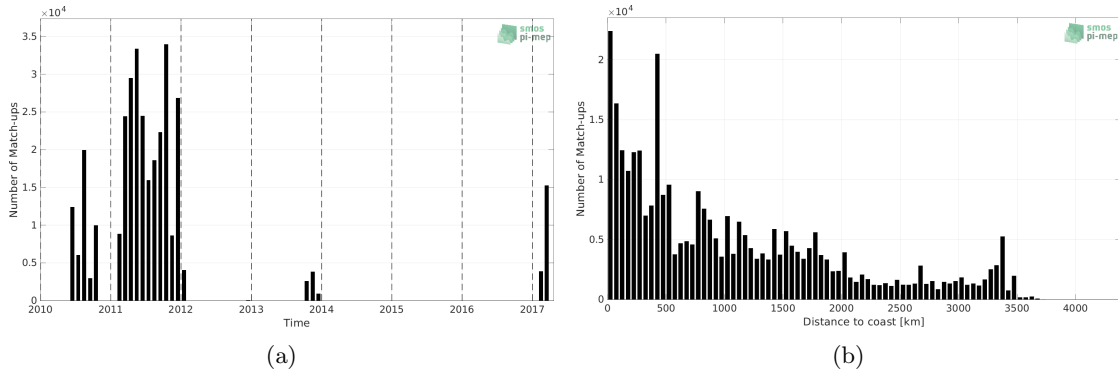
Figure 1: Number of match-ups between TSG (GOSUD-Sailing-ship) and SMOS SSS L3 v8 - 9 Days (CATDS-CECOS-LOCEAN) SSS as a function of time (a) and as function of the distance to coast (b) over the Pacific Ocean Pi-MEP region and for the full satellite product period.
