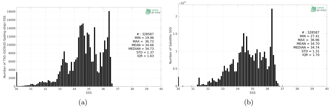
Figure 2: Histograms of SSS from TSG (GOSUD-Sailing-ship) (a) and SMOS SSS L3 v8 - 9 Days (CATDS-CECOS-LOCEAN) (b) considering all match-up pairs per bins of 0.1 over the Pacific Ocean Pi-MEP region and for the full satellite product period.
