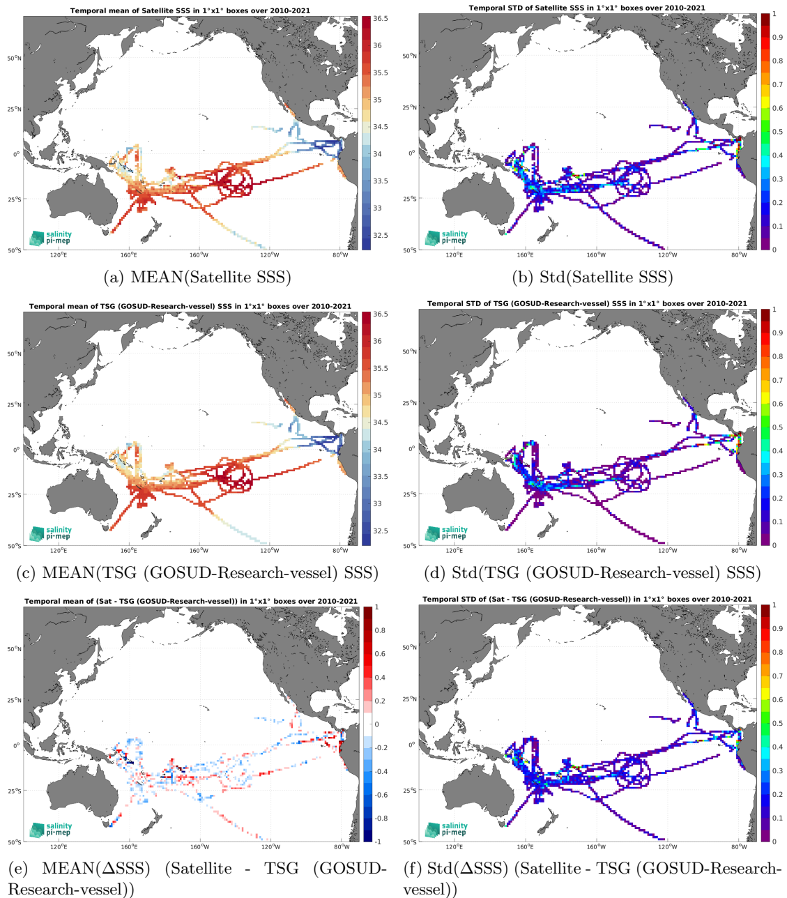
Figure 6: Temporal mean (left) and Std (right) of SSS from SMOS SSS L3 v8 - 9 Days (CATDS-CEC-LOCEAN) (top), TSG (GOSUD-Research-vessel) (middle), and of \Delta SSS (Satellite - TSG (GOSUD-Research-vessel)). Only match-up pairs are used to generate these maps.
