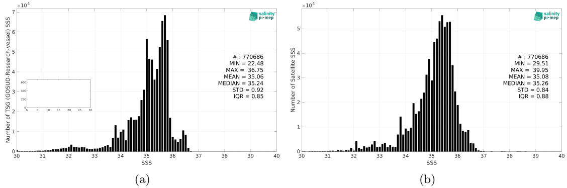
Figure 2: Histograms of SSS from TSG (GOSUD-Research-vessel) (a) and SMOS SSS L3 v8 - 9 Days (CATDS-CEC-LOCEAN) (b) considering all match-up pairs per bins of 0.1 over the Pacific Ocean Pi-MEP region and for the full satellite product period.
