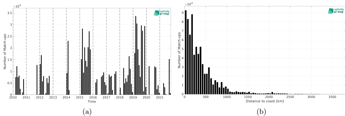
Figure 1: Number of match-ups between TSG (GOSUD-Research-vessel) and SMOS SSS L3 v8 - 9 Days (CATDS-CEC-LOCEAN) SSS as a function of time (a) and as function of the distance to coast (b) over the Pacific Ocean Pi-MEP region and for the full satellite product period.
