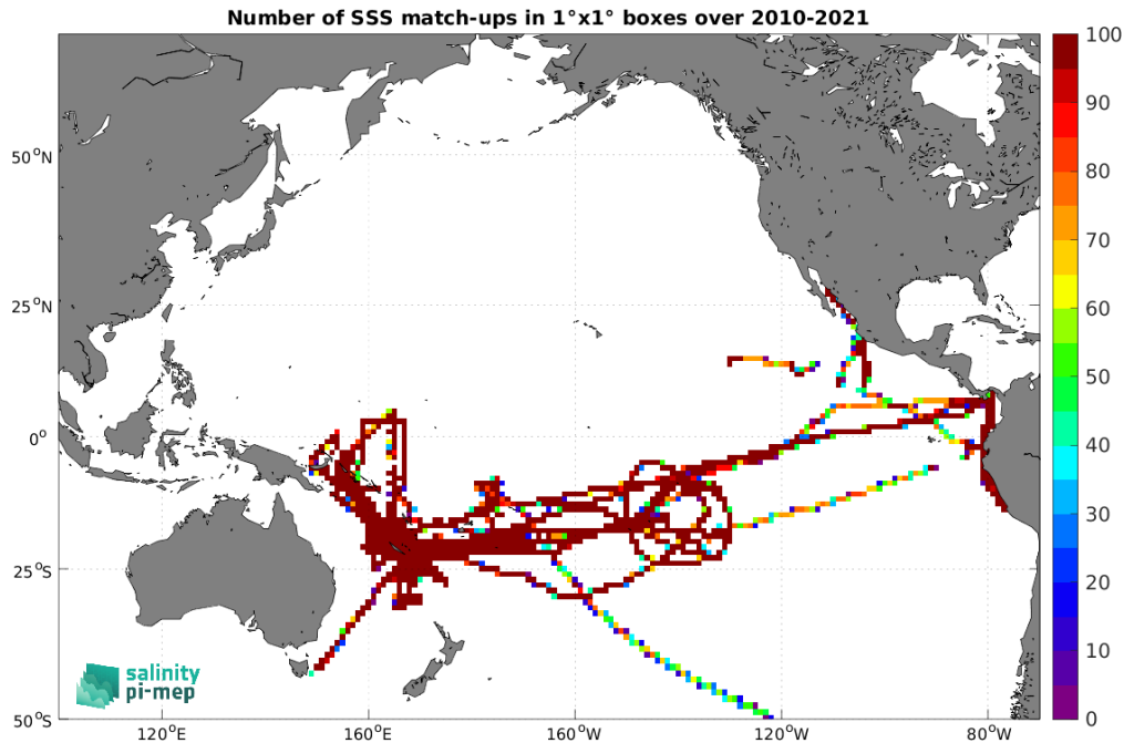
Figure 4: Number of SSS match-ups between TSG (GOSUD-Research-vessel) SSS and the SMOS SSS L3 v8 - 9 Days (CATDS-CEC-LOCEAN) SSS product for the Pacific Ocean Pi-MEP region over 1^\circ \times 1^\circ boxes and for the full satellite product period.
