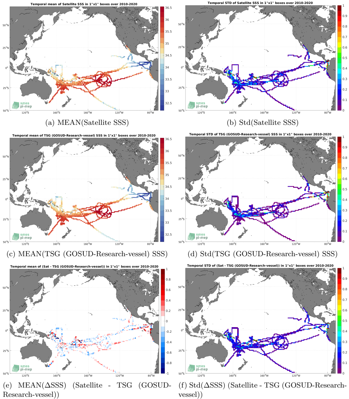
Figure 6: Temporal mean (left) and Std (right) of SSS from SMOS SSS L3 v8 - 9 Days (CATDS-CECOS-LOCEAN) (top), TSG (GOSUD-Research-vessel) (middle), and of \Delta SSS (Satellite - TSG (GOSUD-Research-vessel)). Only match-up pairs are used to generate these maps.
