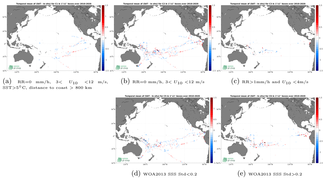
Figure 12: Temporal mean gridded over spatial boxes of size 1^\circ \times 1^\circ of \Delta SSS (SMOS SSS L3 v8 - 9 Days (CATDS-CECOS-LOCEAN) - TSG (GOSUD-Research-vessel)) for 5 different subdatasets corresponding to:RR=0 mm/h, 3 < U_{10} < 12 m/s, SST>5°C, distance to coast > 800 km (a), RR=0 mm/h, 3 < U_{10} < 12 m/s (b), RR>1mm/h and U_{10} < 4 m/s (c), WOA2013 SSS Std<0.2 (d), WOA2013 SSS Std>0.2 (e).
