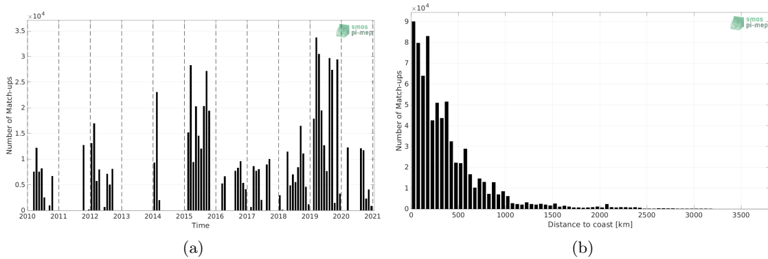
Figure 1: Number of match-ups between TSG (GOSUD-Research-vessel) and SMOS SSS L3 v8 - 9 Days (CATDS-CECOS-LOCEAN) SSS as a function of time (a) and as function of the distance to coast (b) over the Pacific Ocean Pi-MEP region and for the full satellite product period.
