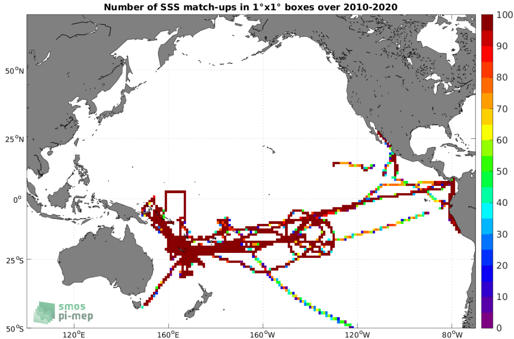
Figure 4: Number of SSS match-ups between TSG (GOSUD-Research-vessel) SSS and the SMOS SSS L3 v8 - 9 Days (CATDS-CECOS-LOCEAN) SSS product for the Pacific Ocean Pi-MEP region over 1^\circ \times 1^\circ boxes and for the full satellite product period.
