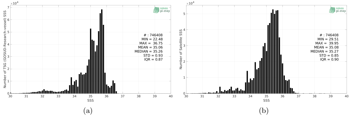
Figure 2: Histograms of SSS from TSG (GOSUD-Research-vessel) (a) and SMOS SSS L3 v8 - 9 Days (CATDS-CECOS-LOCEAN) (b) considering all match-up pairs per bins of 0.1 over the Pacific Ocean Pi-MEP region and for the full satellite product period.
